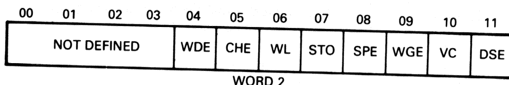
Figure 5-9 Silo Buffer for Status Word 2
