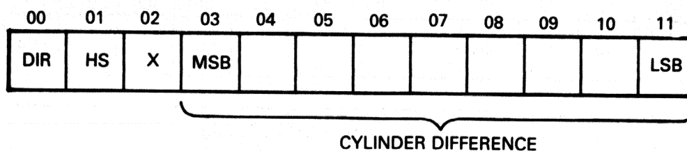
Figure 5-1 Command Register A During a Seek Command
