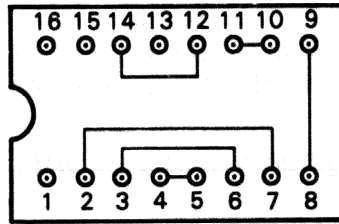
PRIORITY JUMPER PLUG FOR BUS REQUEST LEVEL FIVE (5)
