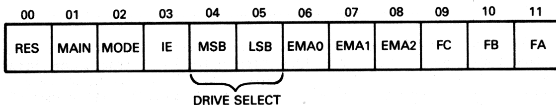
Figure 5-3 Command Register B
