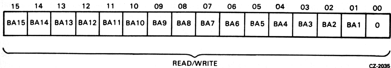
Figure 4-2 BA Register
