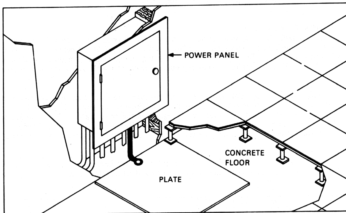
Figure 2-4 Power Panel Grounded To Metal Plate
