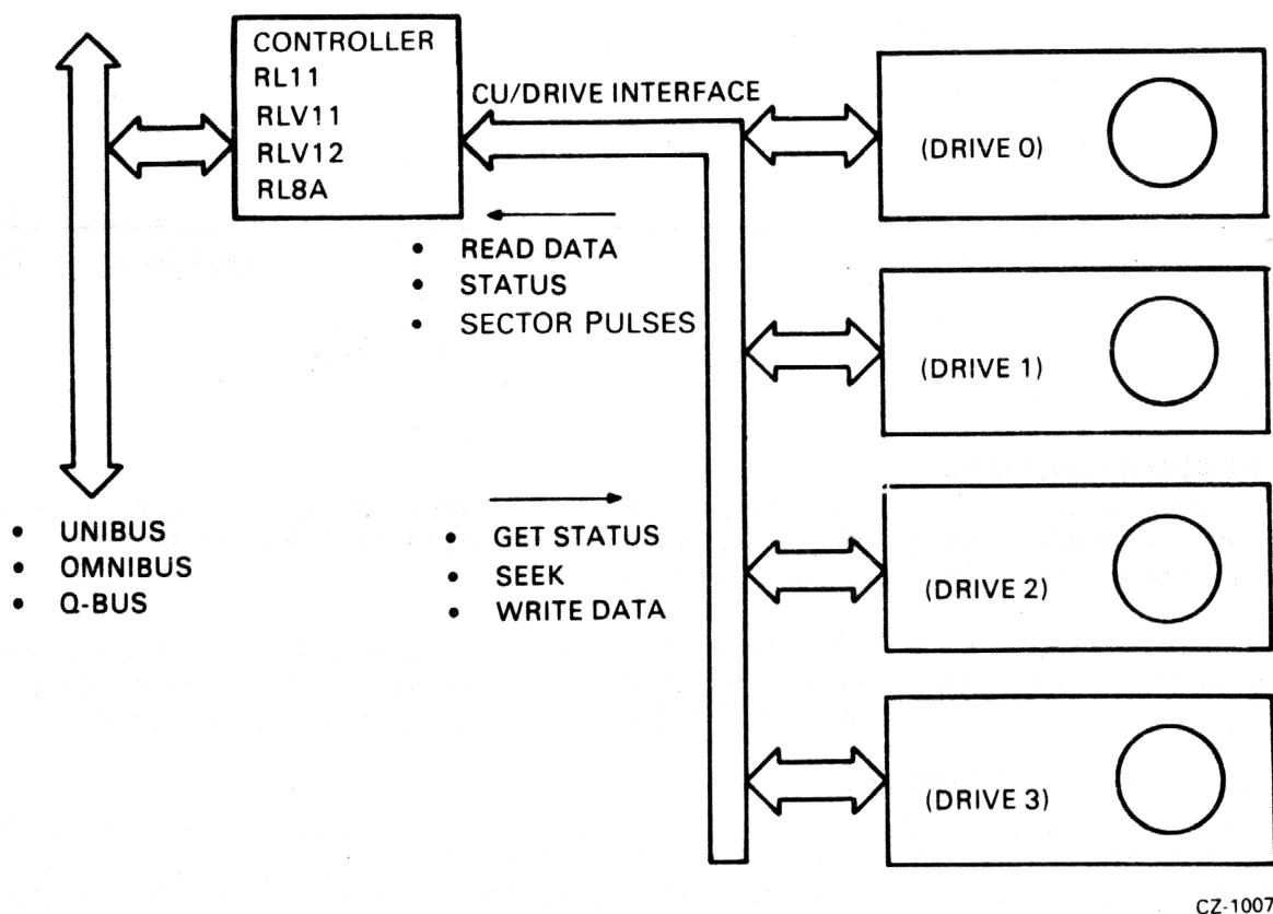
Figure 1-1 Typical RL01/RL02 Mass Storage Subsystem Configuration
