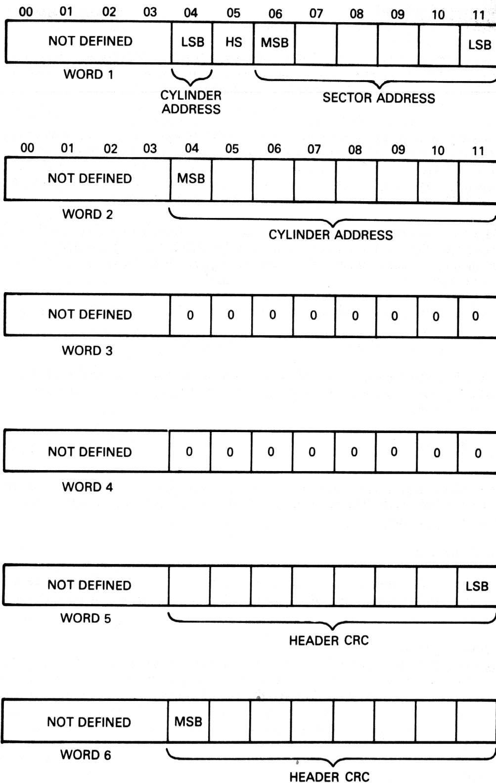
Figure 5-11 Register Summary (Sheet 3 of 3)
