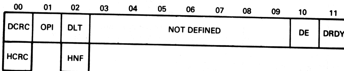
Figure 5-7 Error Register
