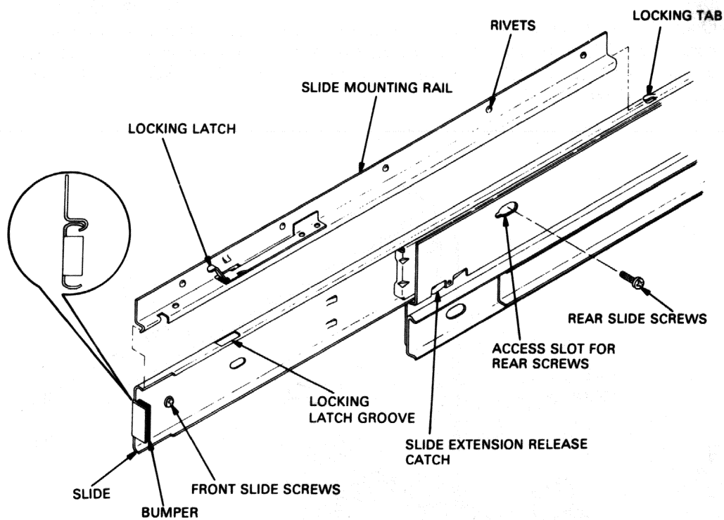
Figure 2-23b RL01/RL02 Cabinet Installation
