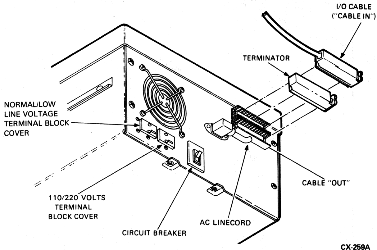
Figure 2-1 RL01/RL02 Disk Drive – Rear View
