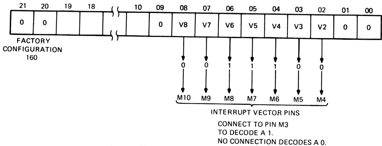
Figure 2-20 RLV12 Format Interrupt Vector
