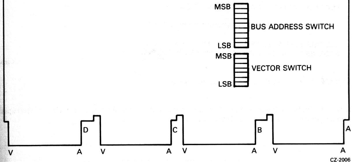
Figure 2-13 RLV11 Bus Interface Module (M8014) (Component Side)
