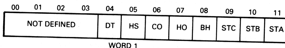
Figure 5-8 Silo Buffer for Status Word 1
