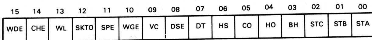
Figure 4-6 MPR – Following a Get Status Command
