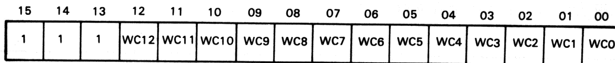
Figure 4-8 MPR – Used as a Word Counter
