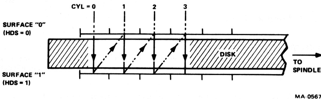
Figure 1-4 Access Method for Sequential Transfers
