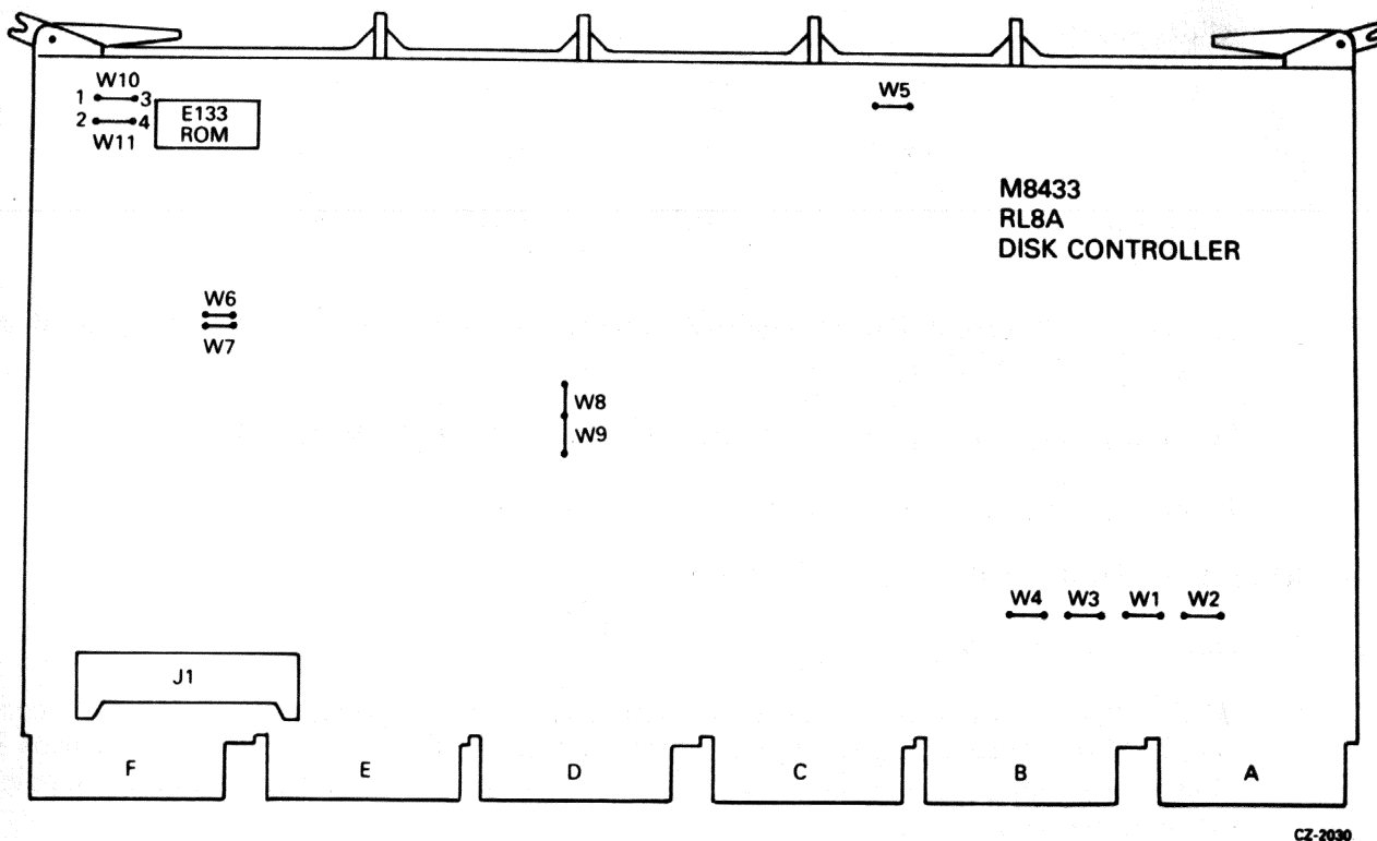
Figure 2-21 RL8A Jumpers
