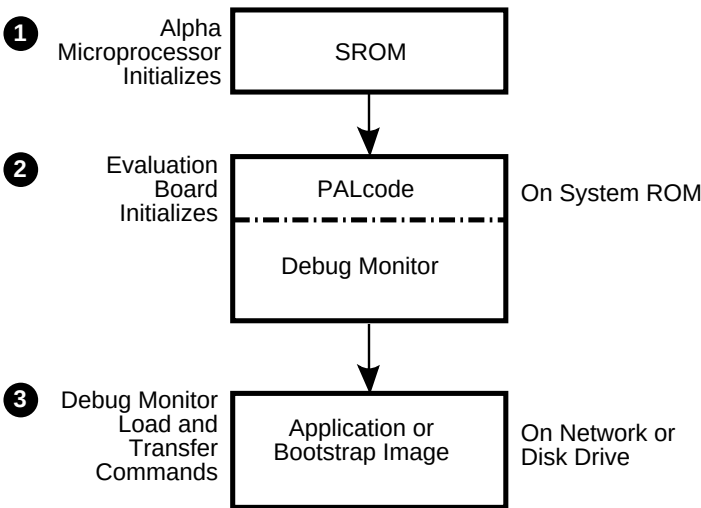
Figure 4-1 Bootstrap Process
