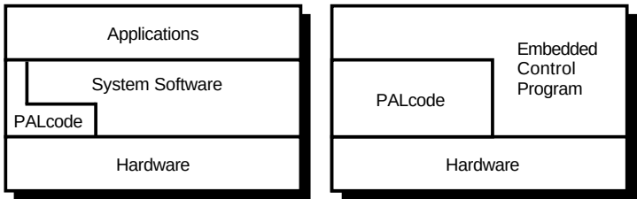
Figure 1-1 PALcode Role in Alpha Architecture
