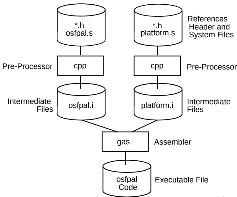
Figure 3–3 PALcode Build Process
