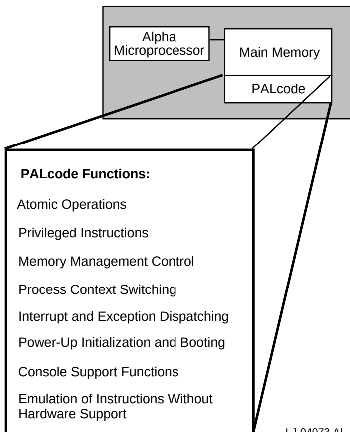
Figure 1-2 PALcode Functions
