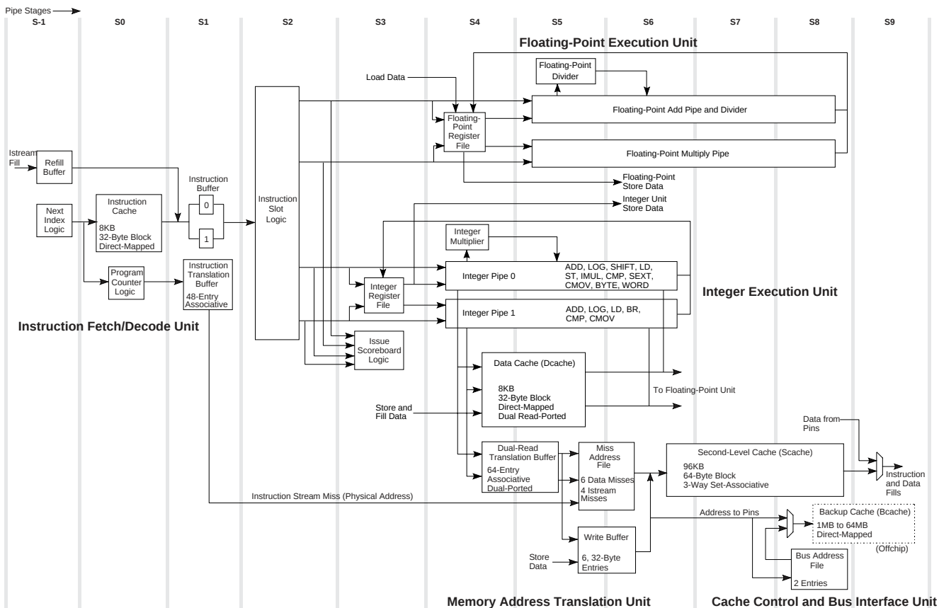
Figure 1 21164 Microprocessor Block/Pipe Flow Diagram
