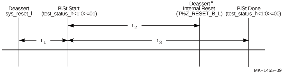
Figure 19 BiSt Timing Event—Time Line
