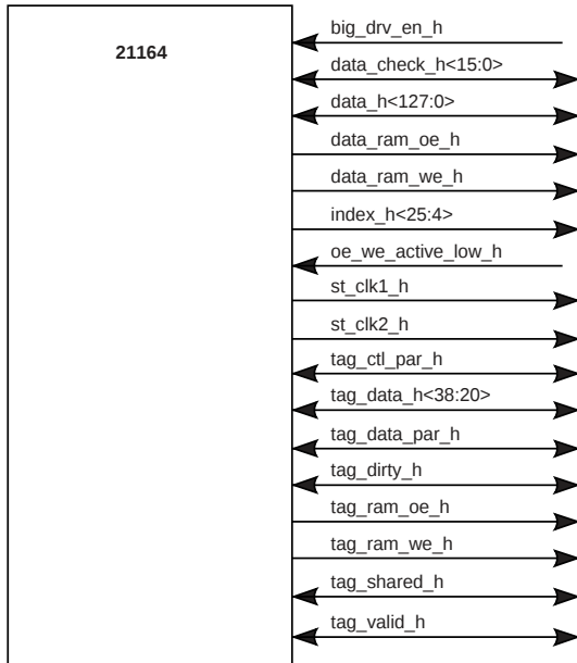
Figure 9 21164 Bcache Interface Signals
