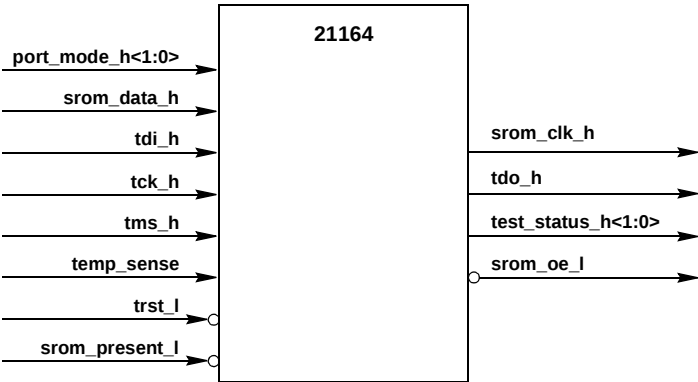
Figure 12 21164 Test Signals
