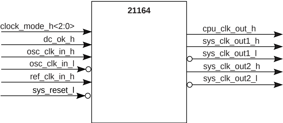
Figure 6 21164 Clock Signals
