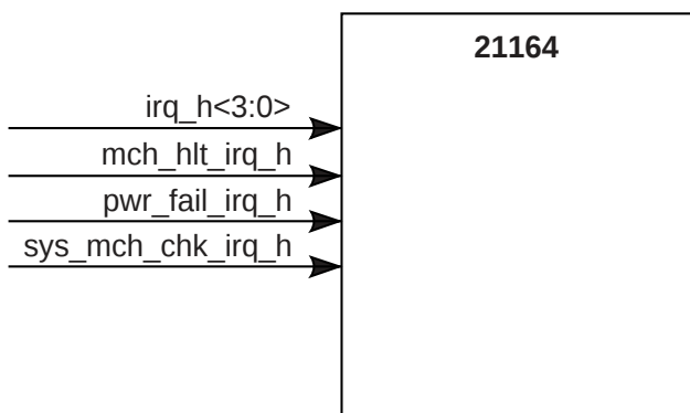
Figure 11 21164 Interrupt Signals
