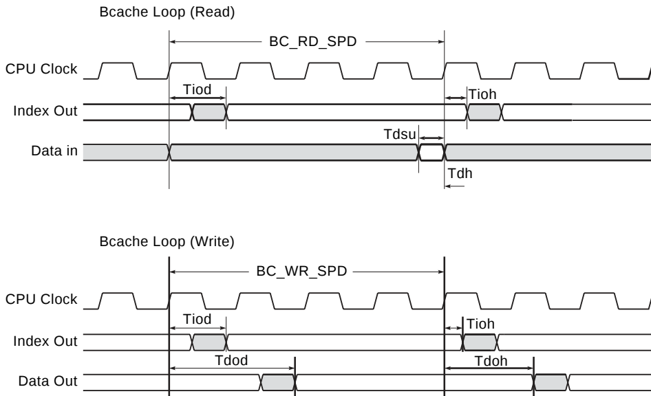
Figure 16 Bcache Timing
