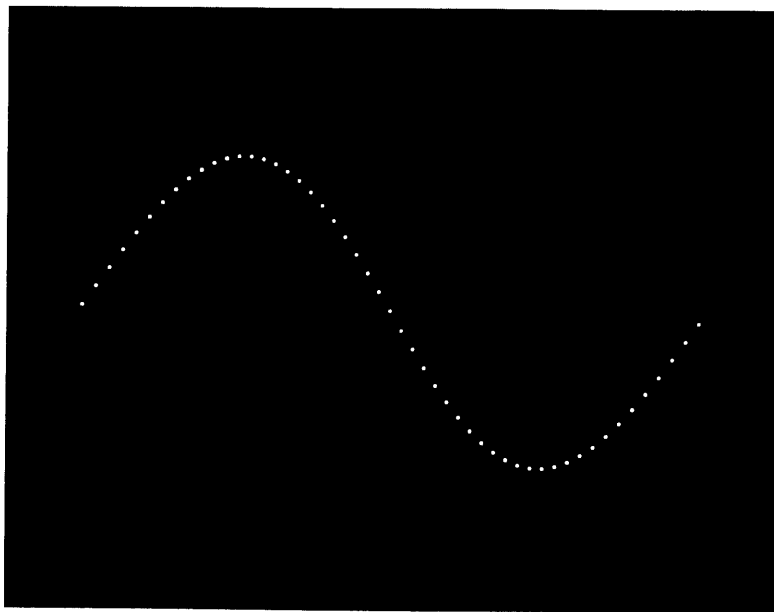
Figure 2-3 YGRA Subroutine
