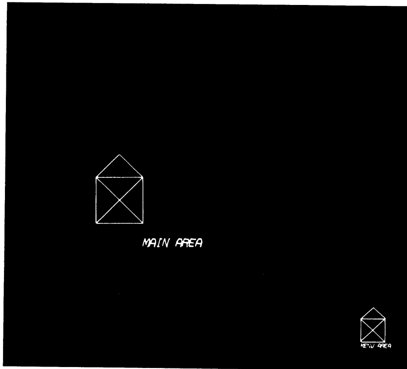
Figure 2-1 AREA Subroutine
