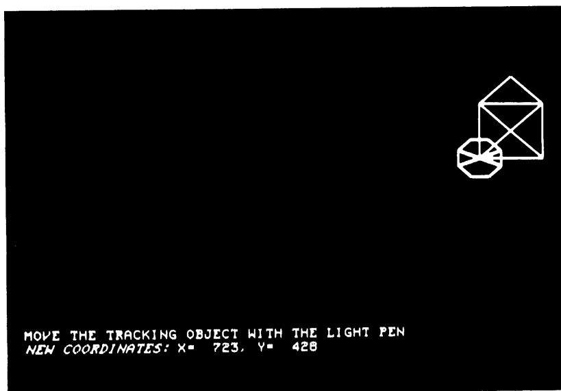
Figure 2-25 TRAKXY Subroutine
