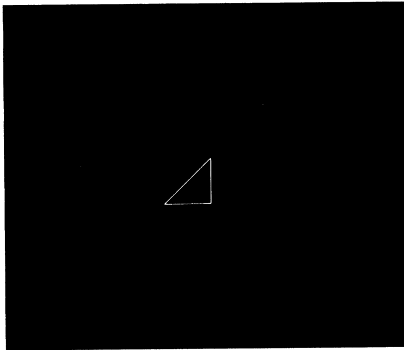
Figure 2-6 VECT Subroutine
