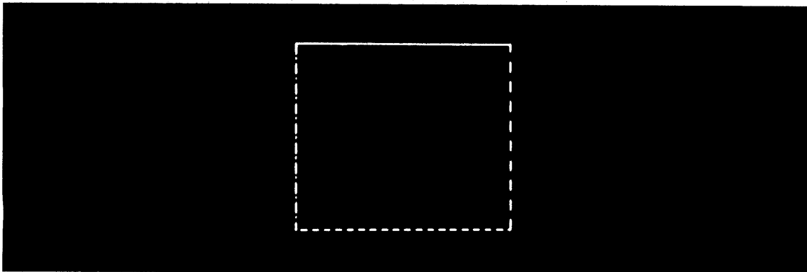
Figure 1-1 Line Types
