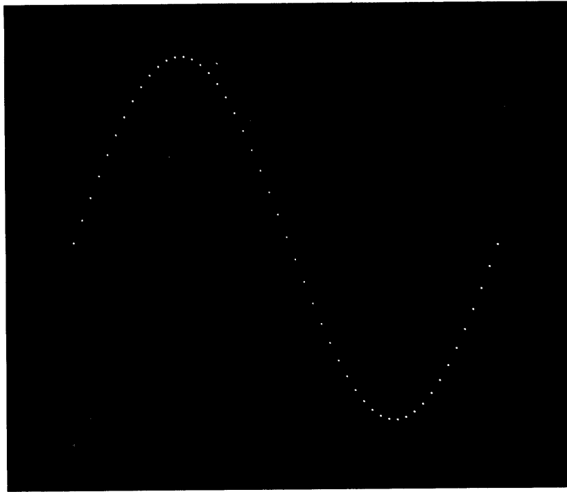
Figure 2-5 RPNT Subroutine
