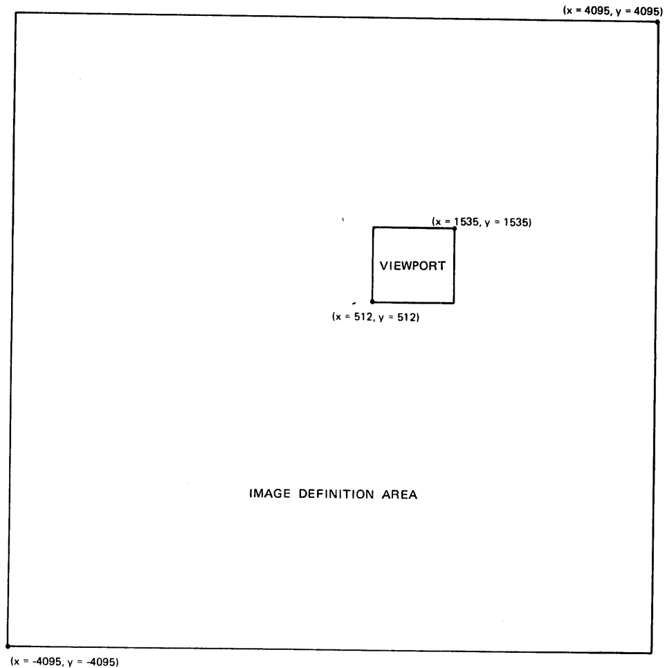
Figure 2-3 VIEWPT Subroutine
