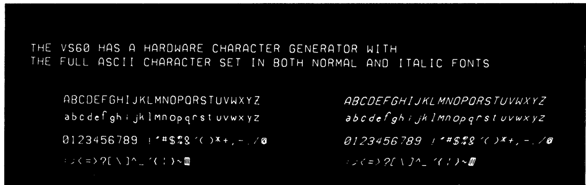
Figure 1-3 Type Fonts
