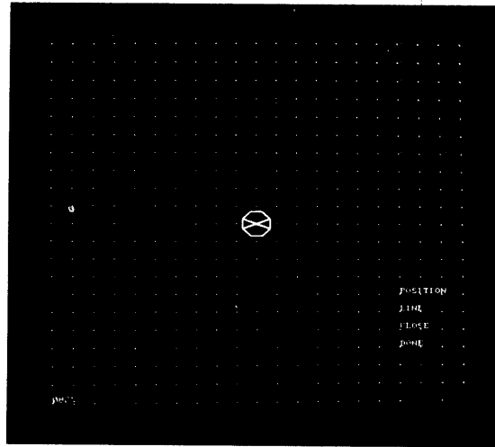
Figure 1-9 Menu Area
