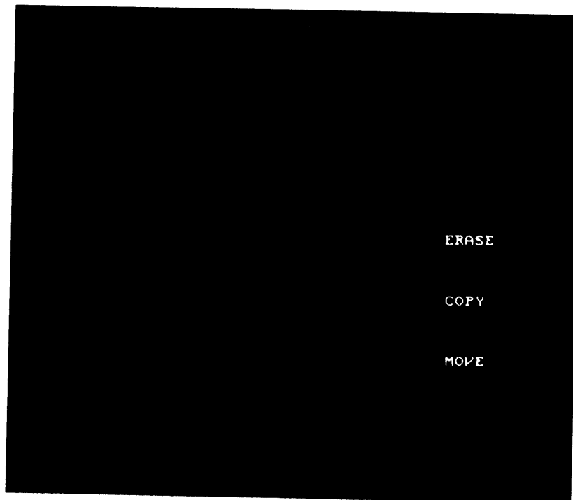
Figure 2-24 INTENS Subroutine
