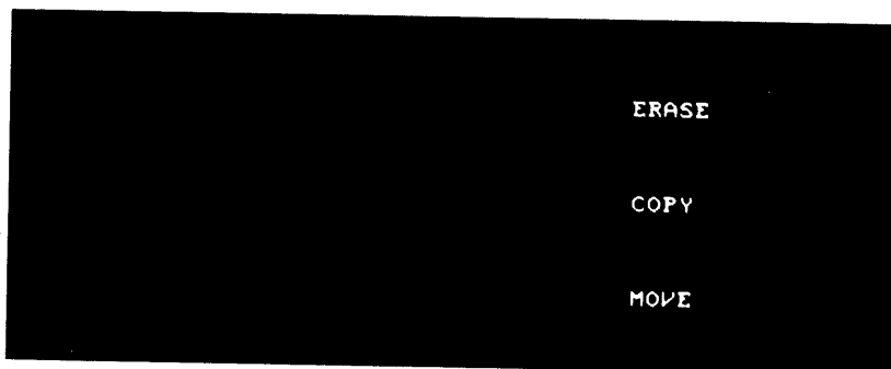
Figure 2-12 MENU Subroutine
