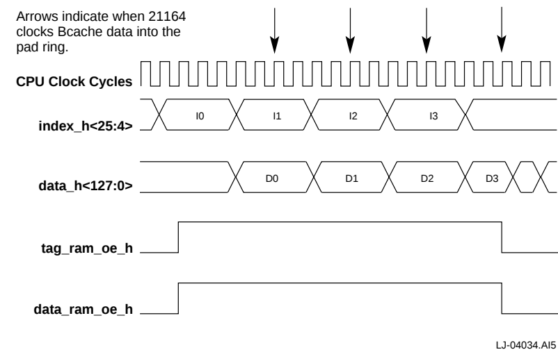
Figure 4–16 Wave Pipeline Timing Diagram
