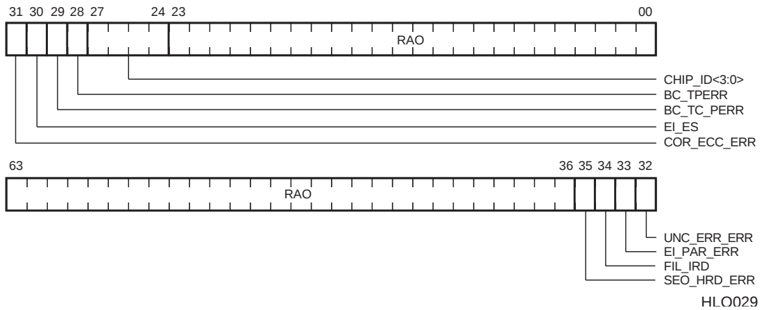
Figure 5–54 External Interface Status (EI_STAT) Register
