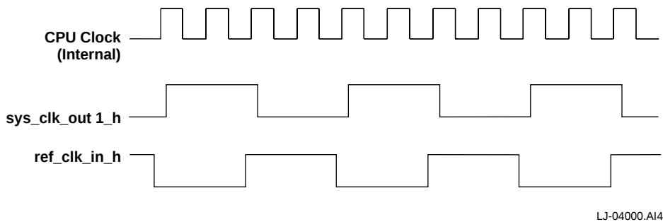
Figure 4–5 ref_clk_in_h Initially Sampled Low
