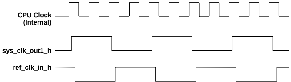
Figure 4–6 ref_clk_in_h Initially Sampled High
