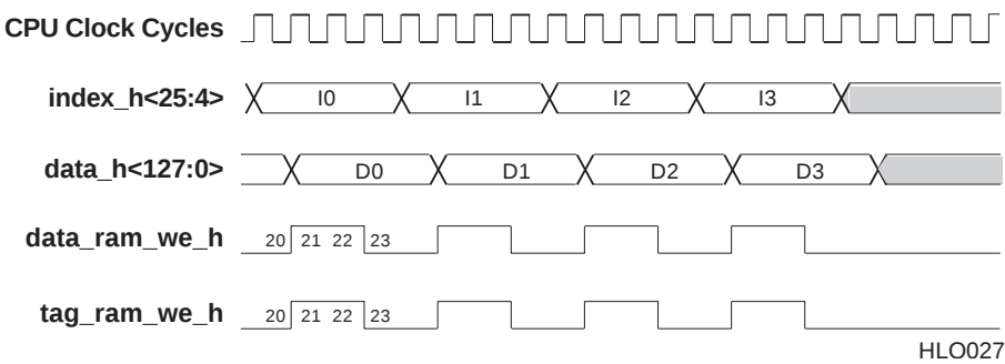
Figure 4–17 Bcache Write Transaction
