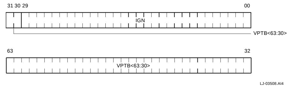
Figure 5–36 MTU Virtual Page Table Base Register (MVPTBR)
