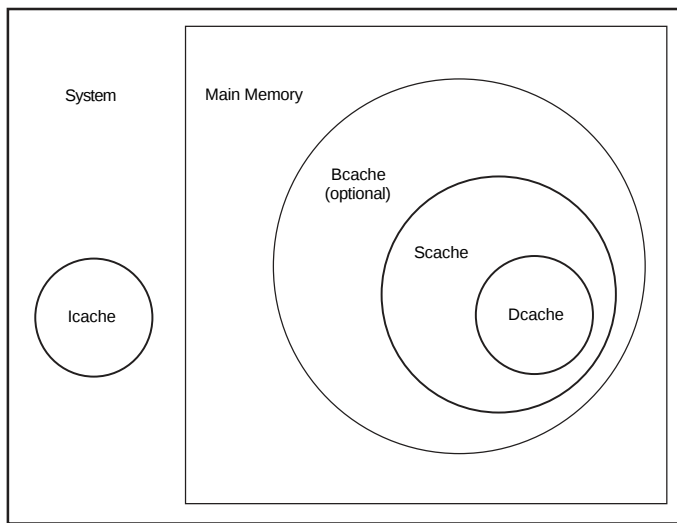
Figure 4–10 Cache Subset Hierarchy
