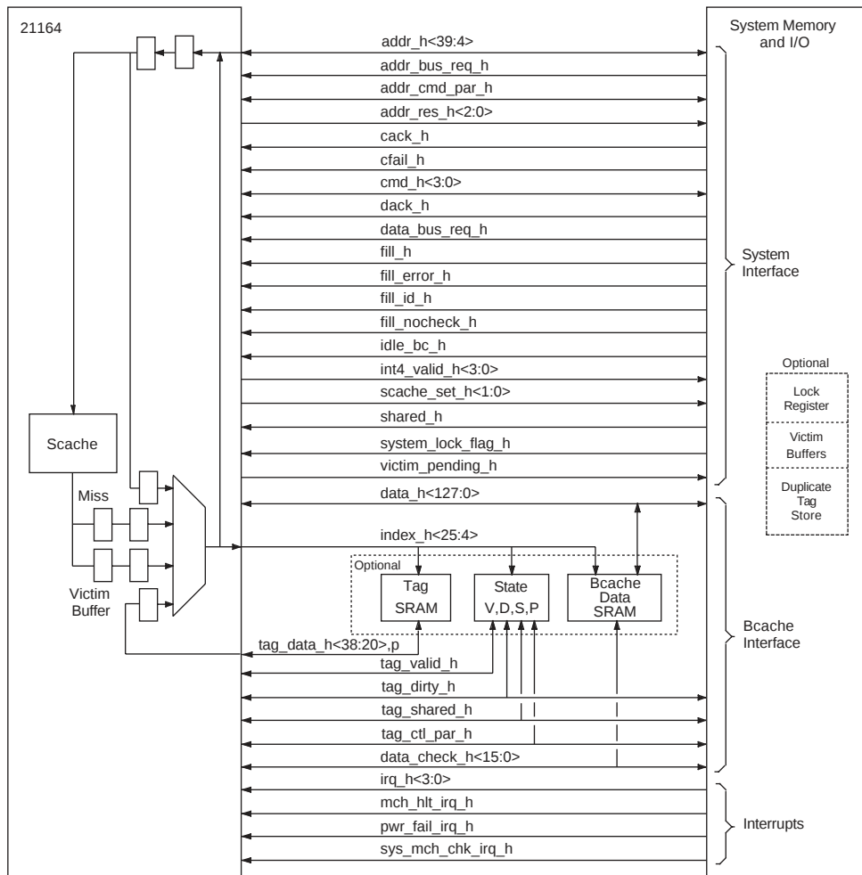
Figure 4–1 21164 System/Bcache Interface
