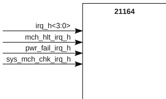
Figure 4–50 21164 Interrupt Signals
