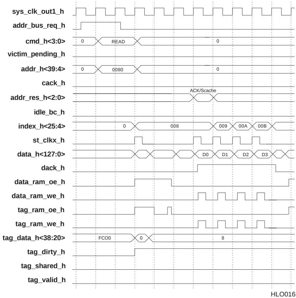
Figure 4–31 Read Timing Diagram (Scache Hit)
