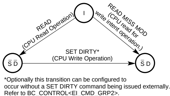
Figure 4–13 Flush-Based Protocol 21164 States
