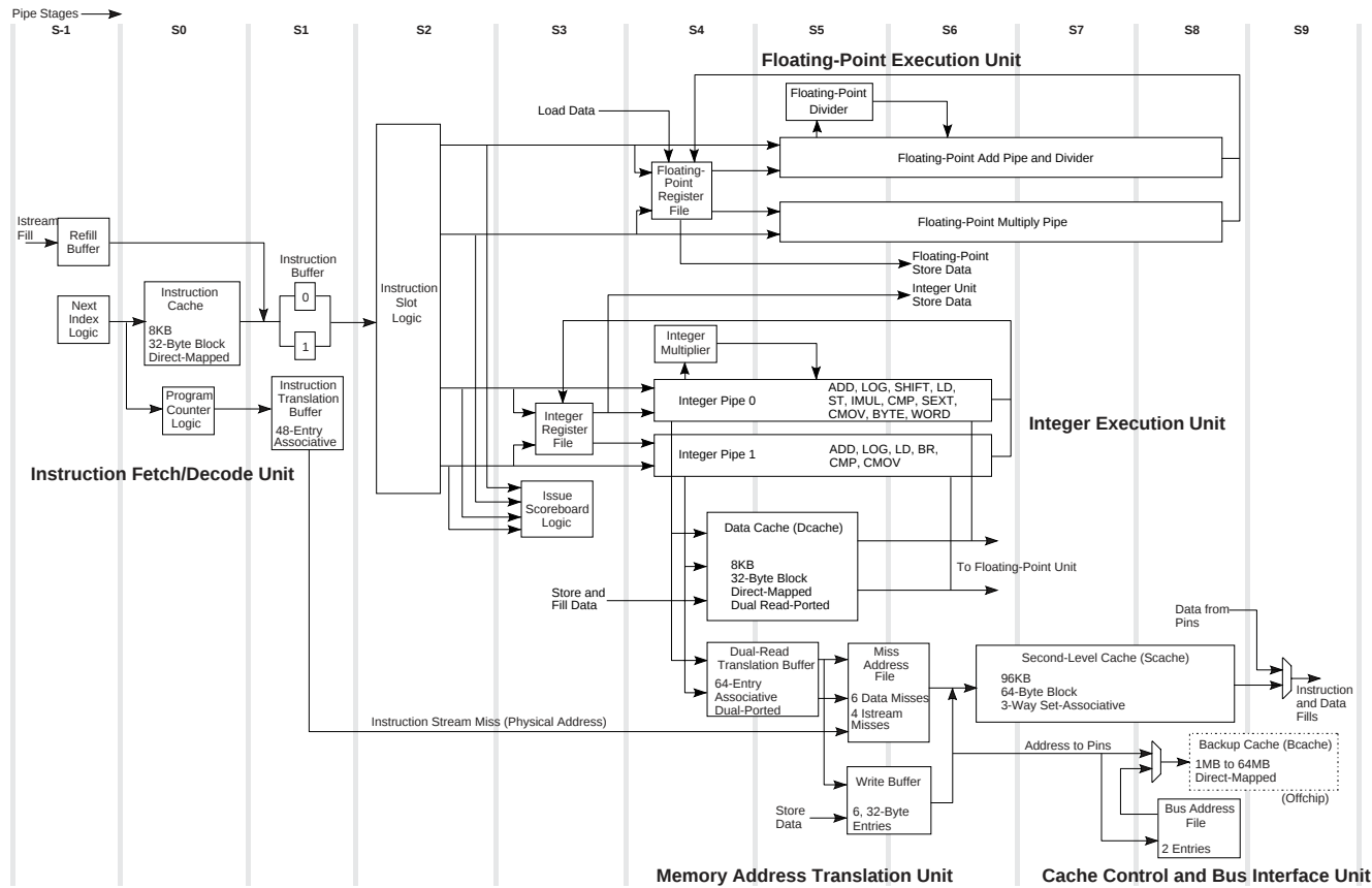
Figure 2-1 21164 Microprocessor Block/Pipe Flow Diagram
