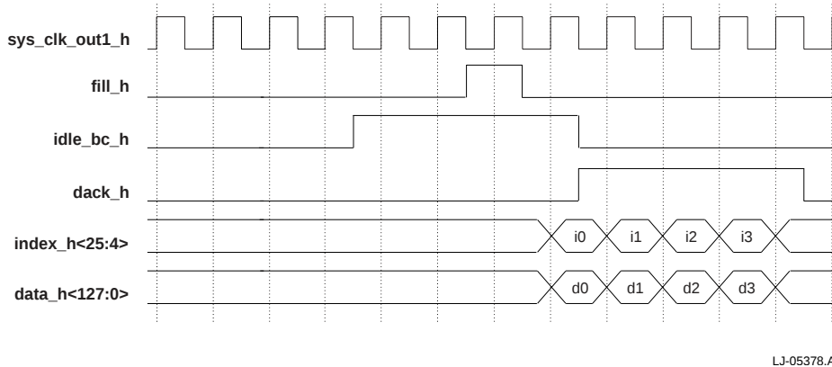
Figure 4–43 sysclk Ratio = 3
