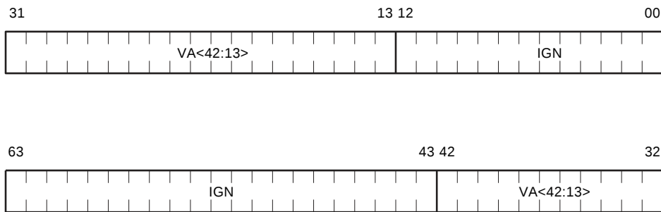
Figure 5–1 Istream Translation Buffer Tag Register (ITB_TAG)
