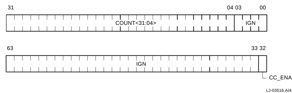
Figure 5–44 Cycle Counter Control (CC_CTL) Register
