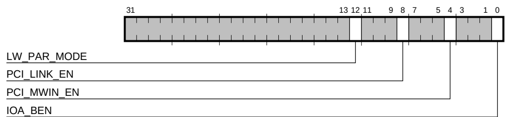
Figure 5–4 Control Register 1
