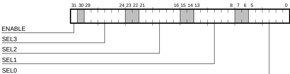
Figure 5–28 Memory Control Debug Register 1
