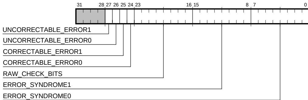
Figure 5–16 Syndrome Register
