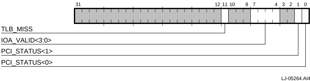
Figure 5–14 Status Register
