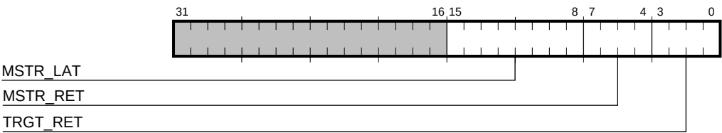
Figure 5–2 PCI Latency Register
