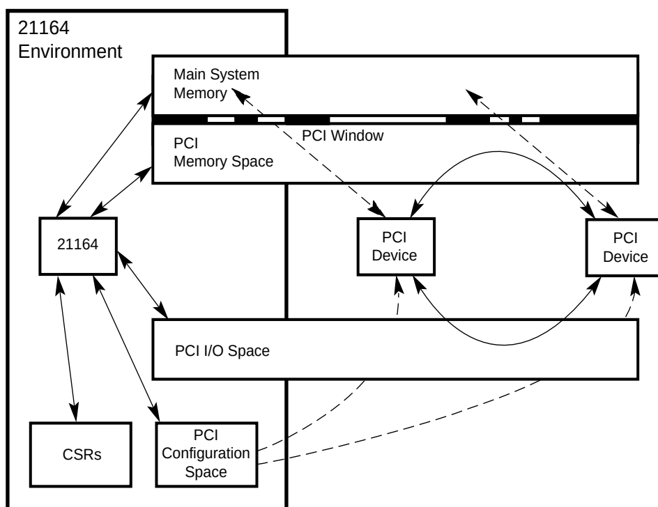
Figure 6–1 Address Space Overview
