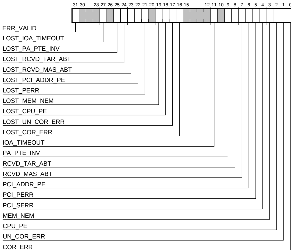
Figure 5–13 Error Register
