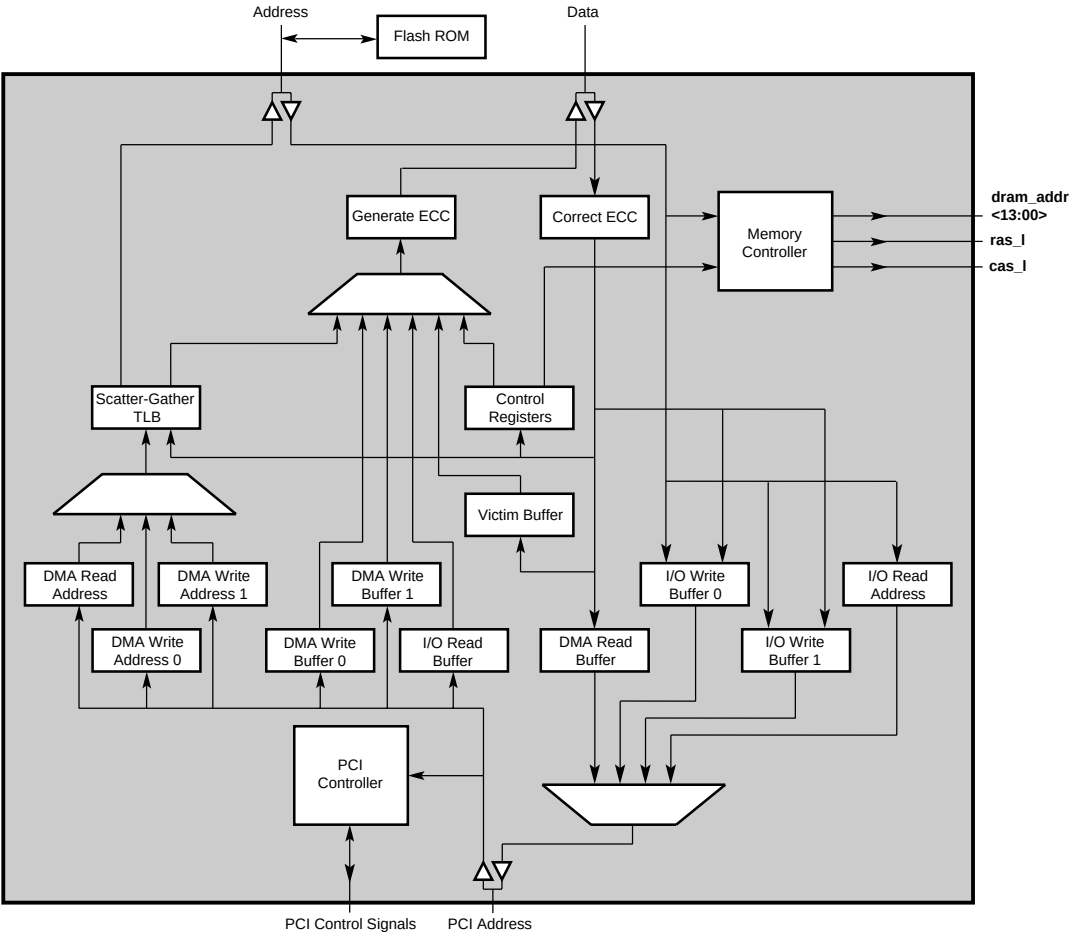
Figure 2-1 21174 Block Diagram
