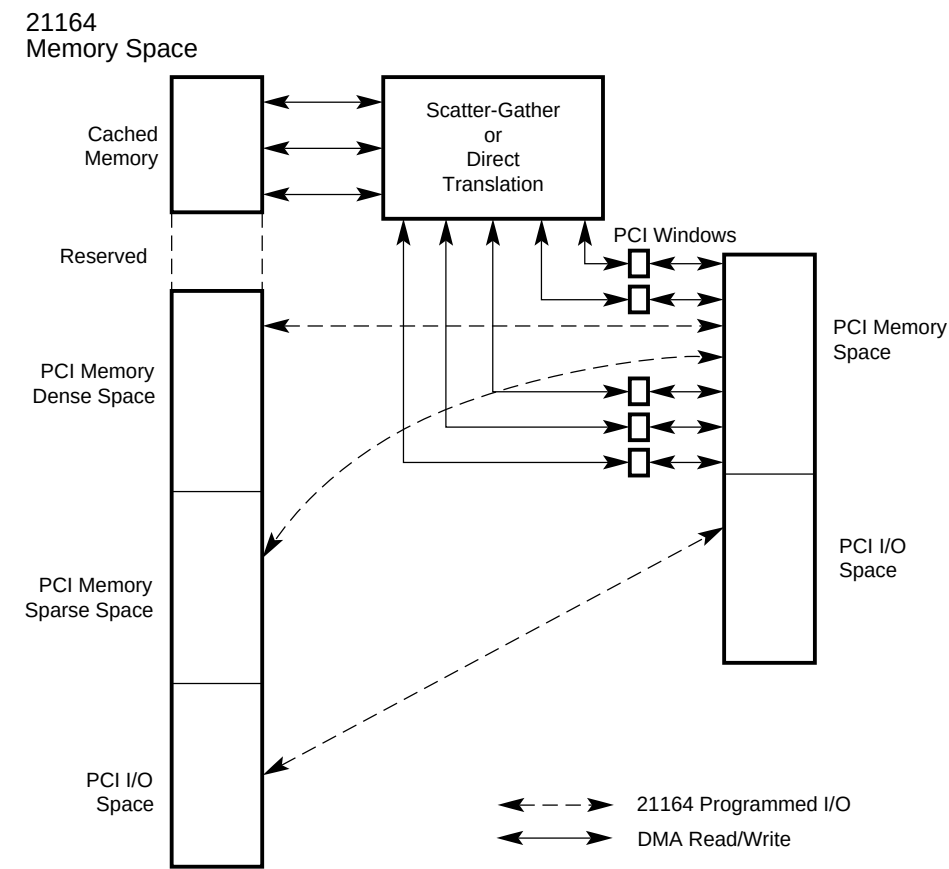
Figure 6-3 21164 Address Space Configuration
