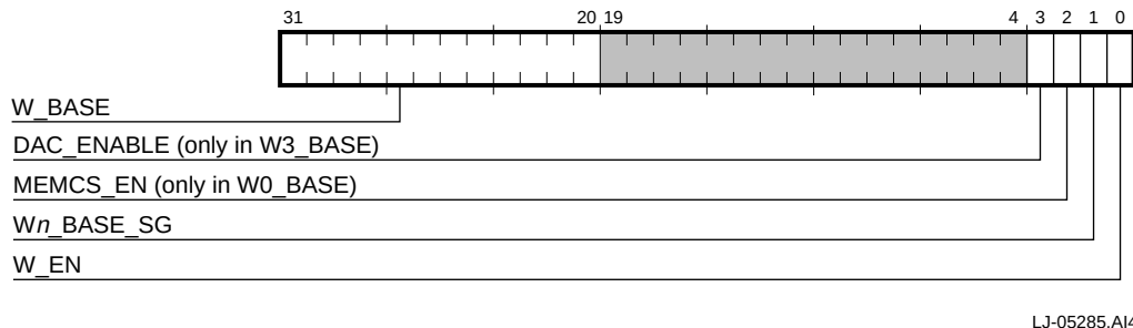
Figure 5–35 Window Base Register
