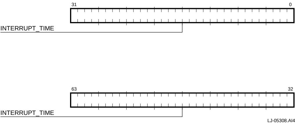
Figure 5–52 Interrupt Time Register
