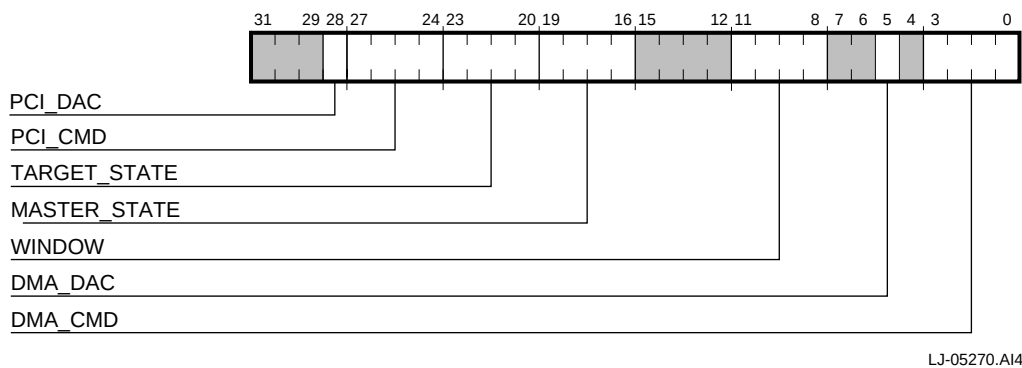
Figure 5–20 PCI Error Register 0
