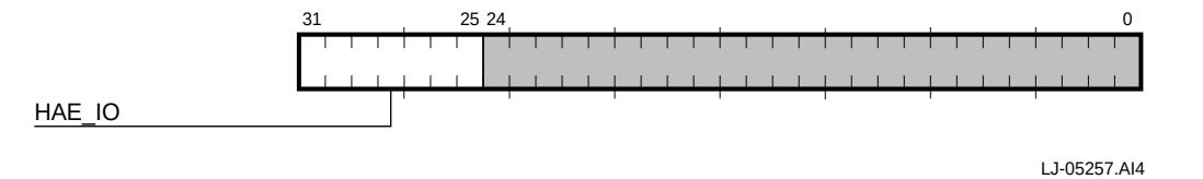
Figure 5–7 Hardware Address Extension Register (HAE_IO)
