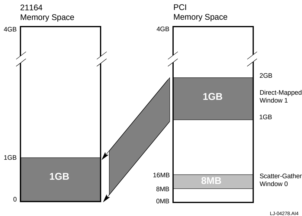
Figure 6–22 Default PCI Window Allocation
