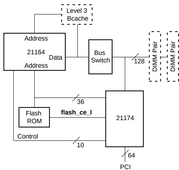
Figure 1–1 System Configuration
