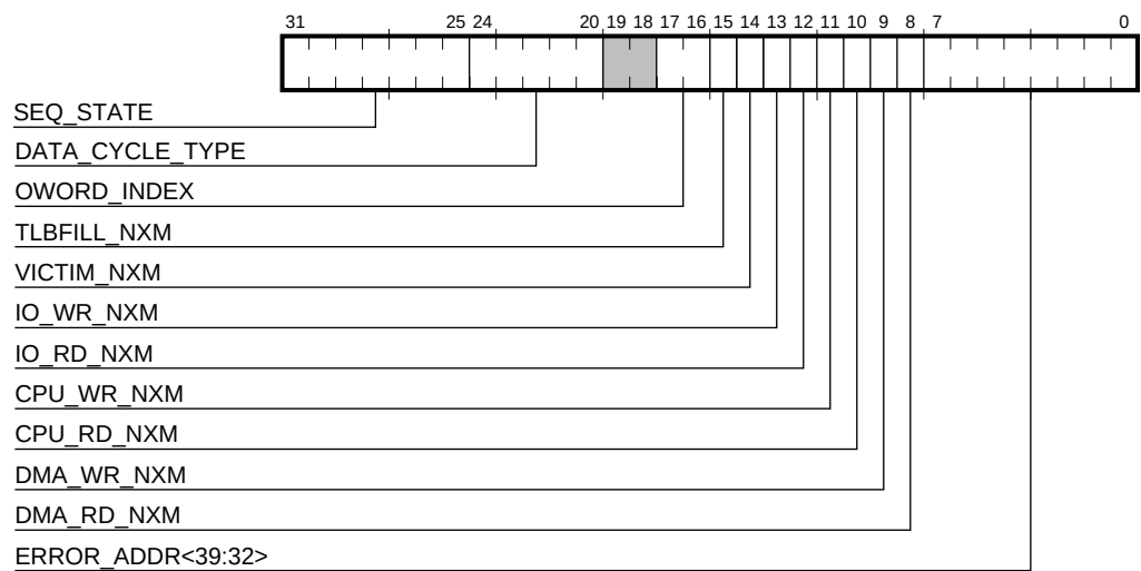
Figure 5–19 Memory Error Status Register
