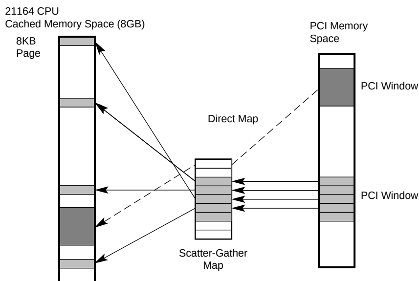
Figure 6–2 Memory Remapping
