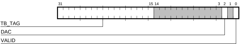
Figure 5–40 Translation Buffer Tag Register
