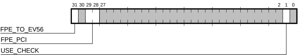
Figure 5–9 Diagnostic Control Register
