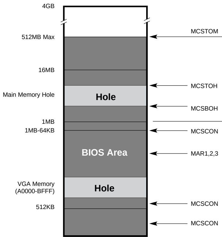
Figure 6–23 mem_cs_l Decode Area
