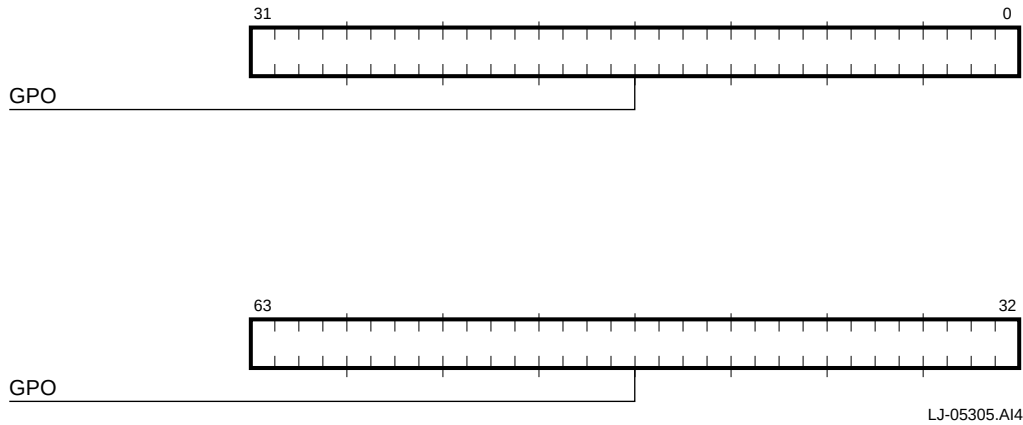
Figure 5–49 General-Purpose Output Register
