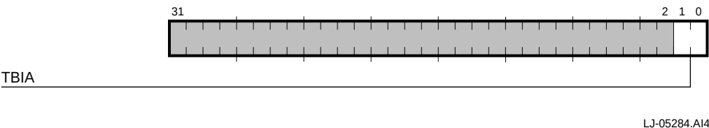
Figure 5–34 Scatter-Gather Translation Buffer Invalidate Register
