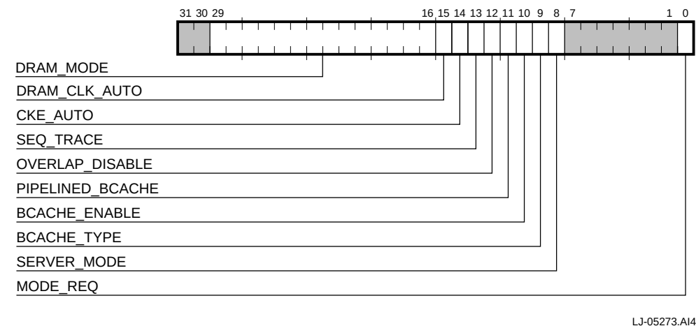
Figure 5–23 Memory Control Register
