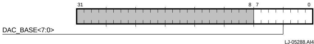
Figure 5–38 Window DAC Base Register
