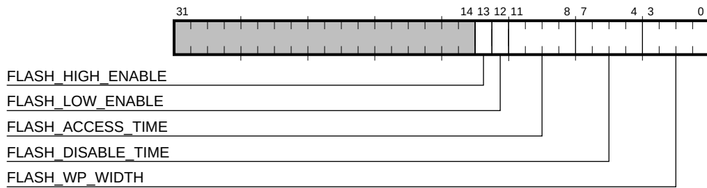
Figure 5–5 Flash Control Register
