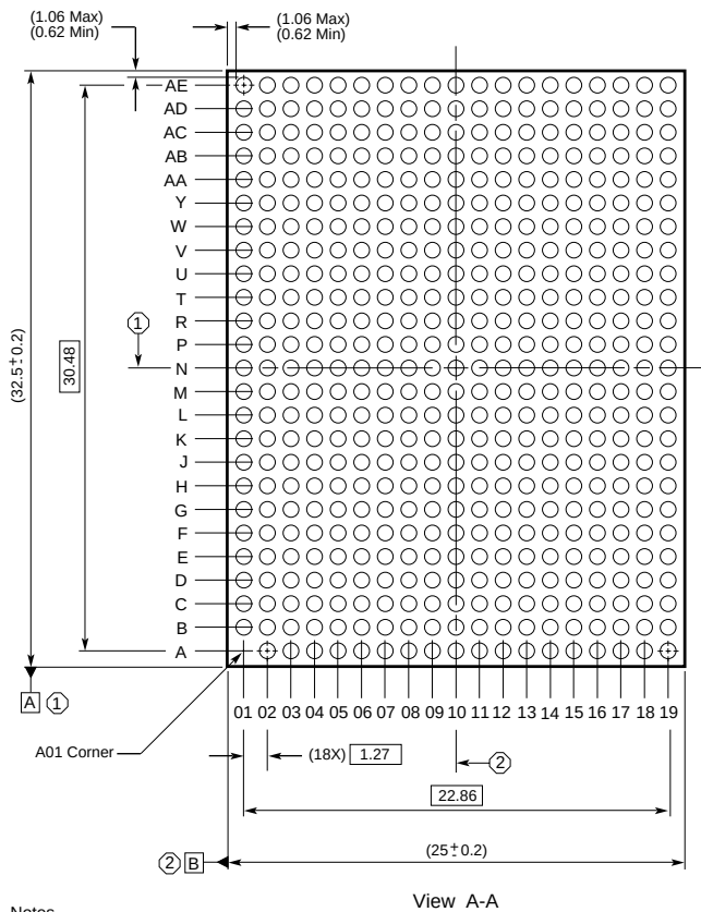
Figure 8-2 21174 Physical Specification
