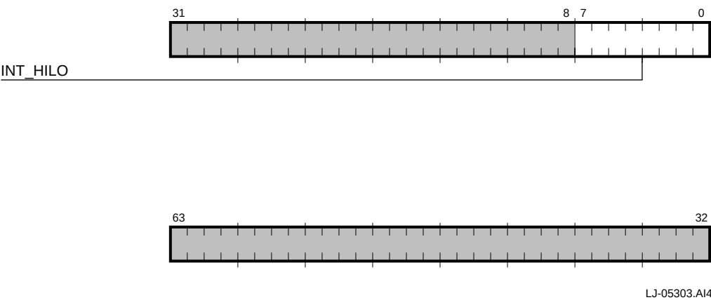
Figure 5–47 Interrupt High/Low Select Register
