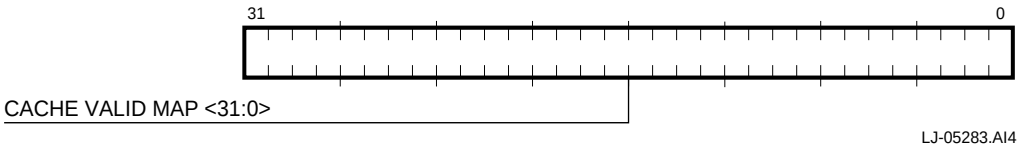
Figure 5–33 Cache Valid Map Register
