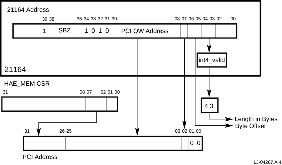
Figure 6–11 PCI Memory Sparse-Space Address Generation – Region 3
