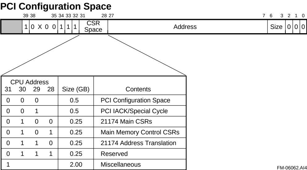
Figure 6–6 21174 CSR Space
