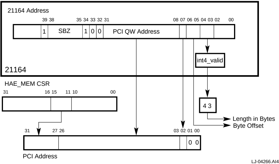
Figure 6–10 PCI Memory Sparse-Space Address Generation – Region 2
