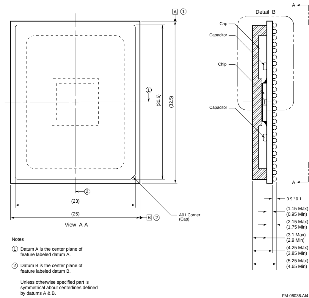
Figure 8–1 474-Pin BGA Package
