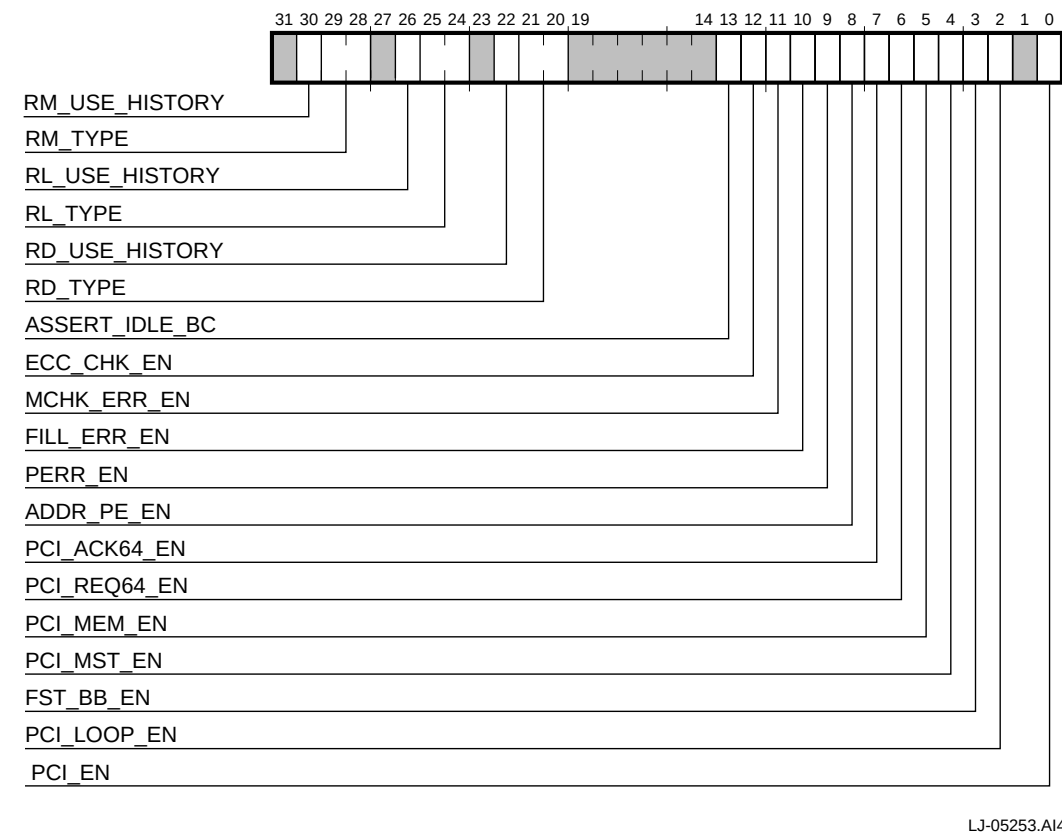
Figure 5–3 Control Register
