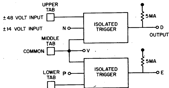
502 PHOTON COUPLED TRIGGER
