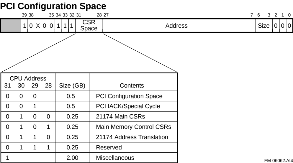
Figure A-6 21174 CSR Space
