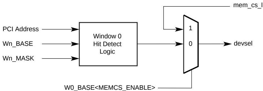
Figure A–24 mem_cs_l Logic
