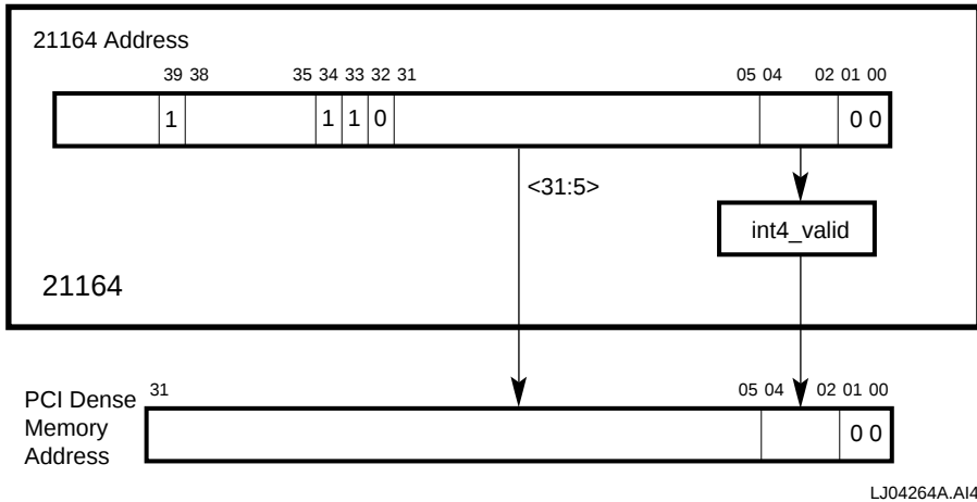
Figure A–8 Dense-Space Address Generation
