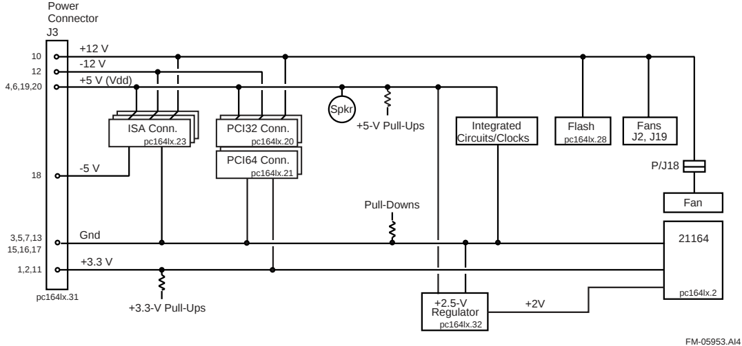
Figure 4-10 AlphaPC 164LX Power Distribution
