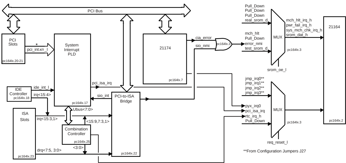
Figure 4-5 Interrupt Logic
