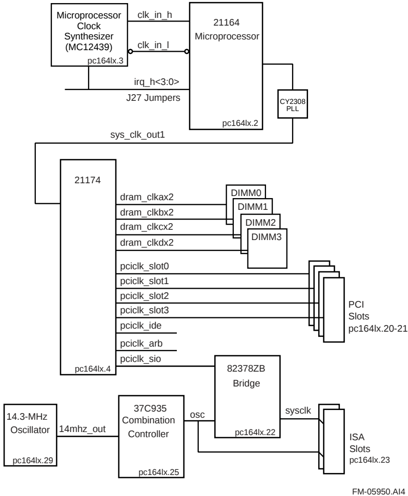
Figure 4–7 AlphaPC 164LX System Clocks
