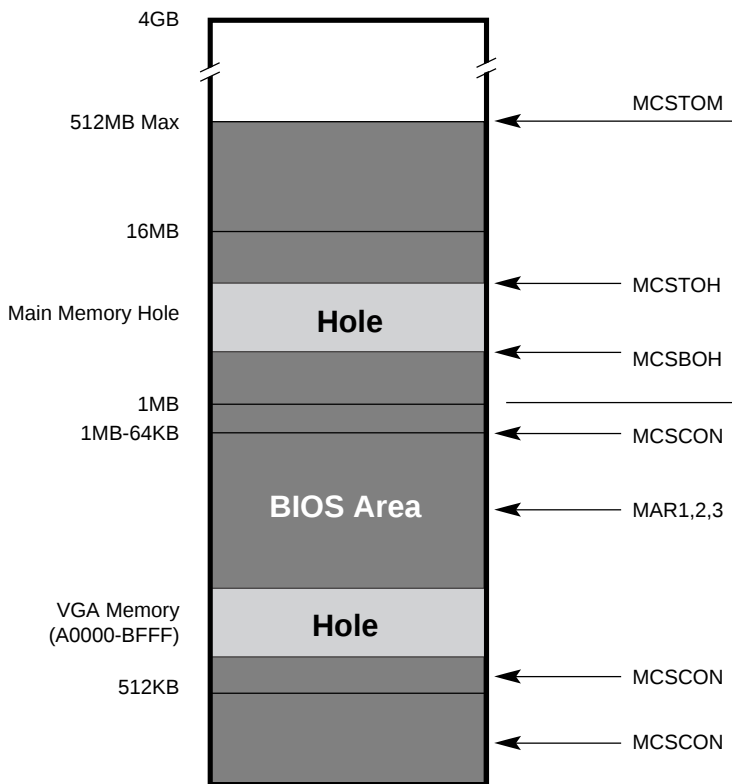
Figure A-23 mem_cs_l Decode Area
