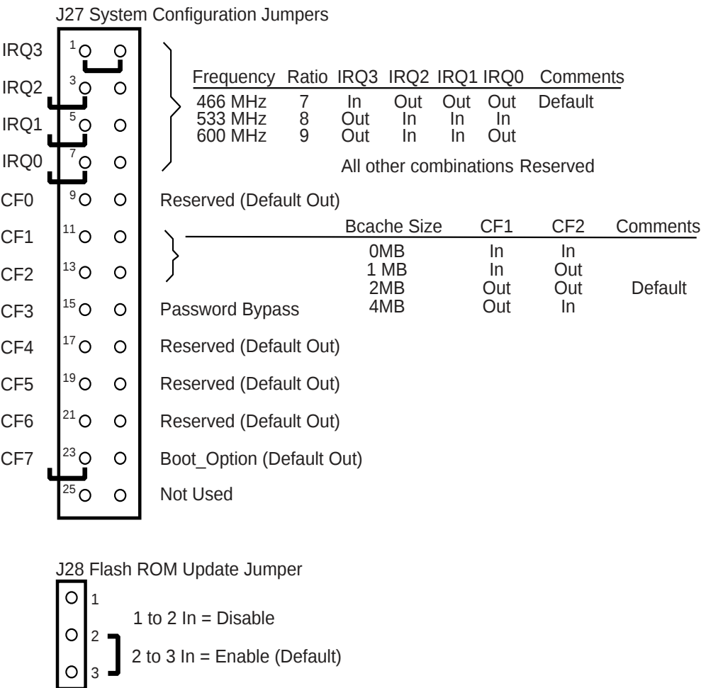
Figure 2–2 AlphaPC 164LX Configuration Jumpers
