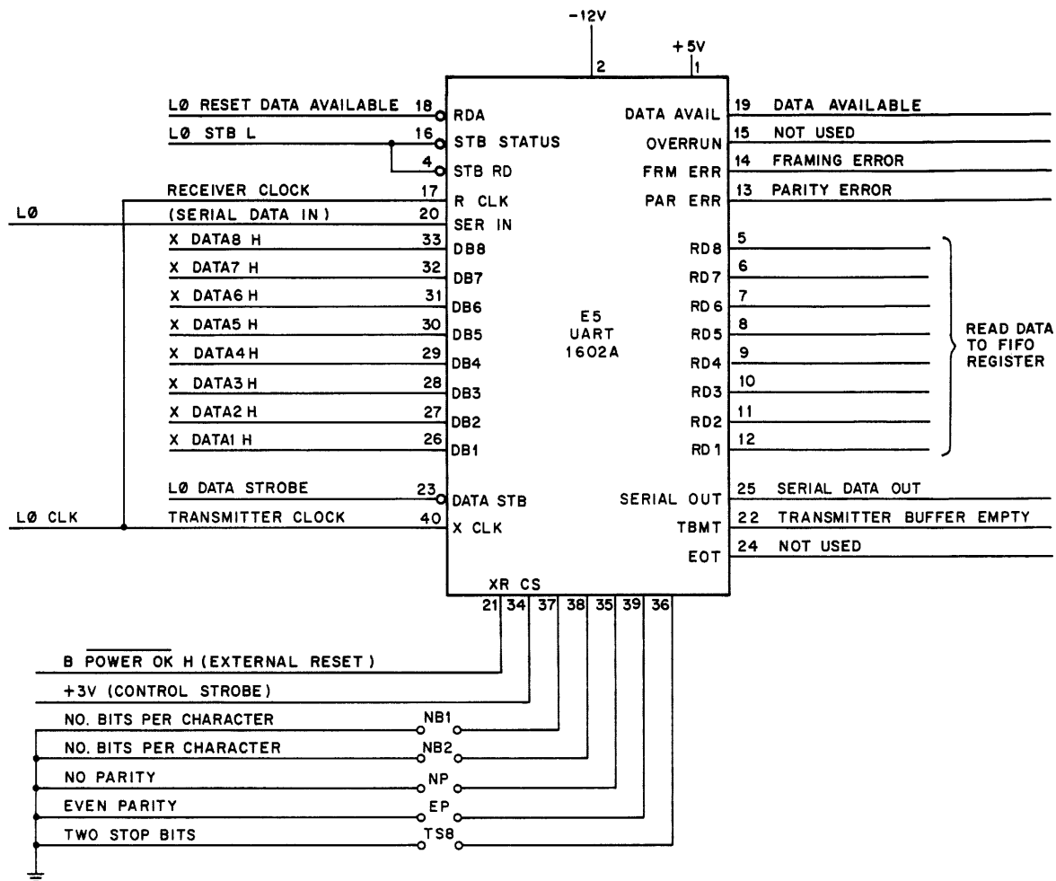
Figure 4-11 Universal Asynchronous Receiver Transmitter (UART)
