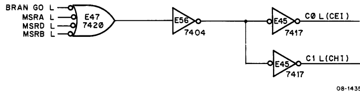
Figure 4-7 C Line Control Logic
