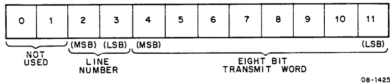
Figure 3-2 Transmit Word
