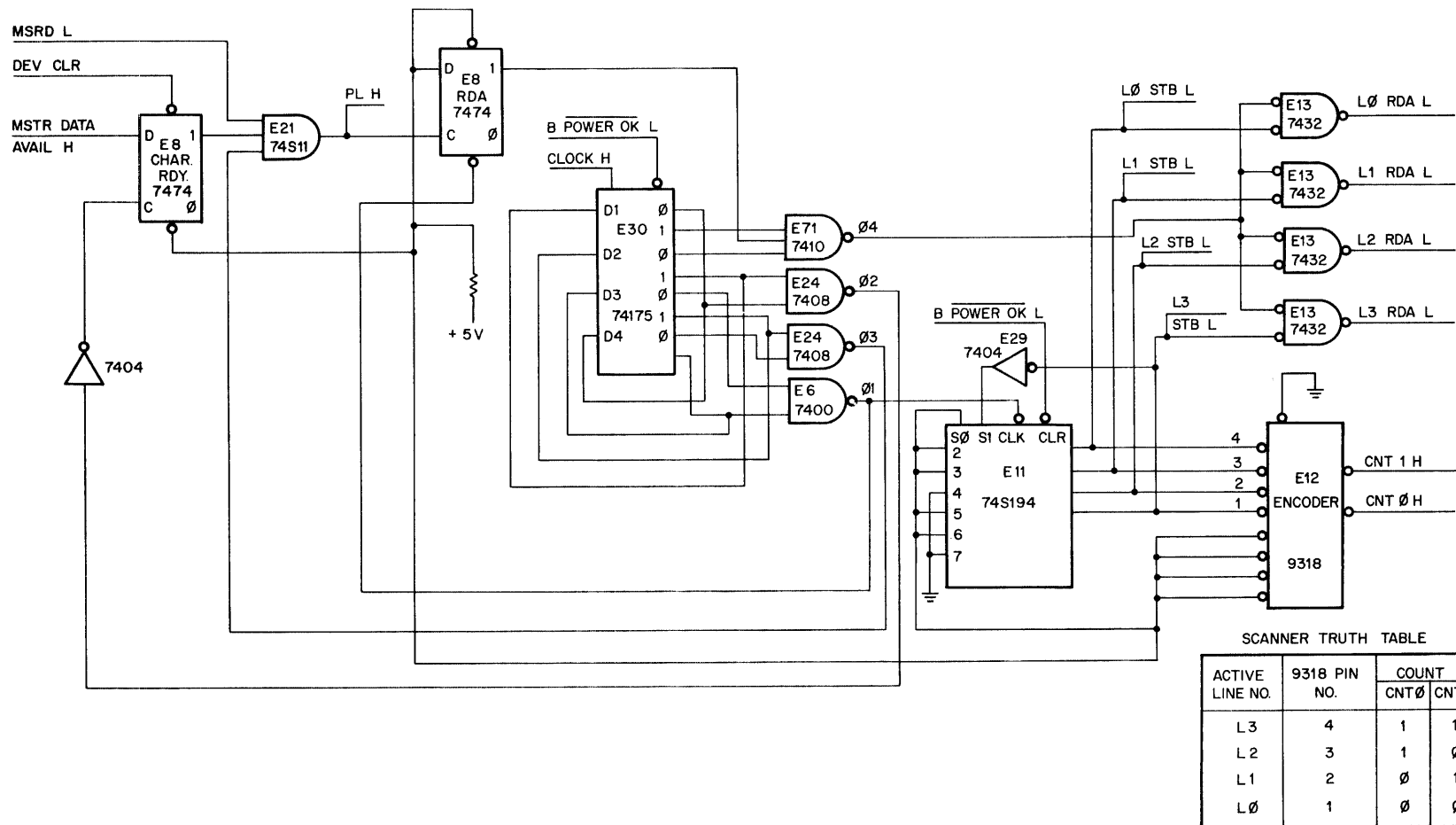
Figure 4-17 Receive Line Scanner Logic
