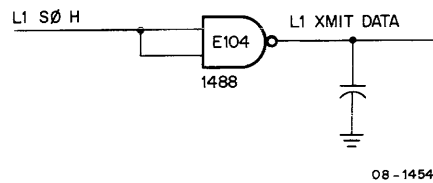
Figure 4-27 TTL To EIA Converter
