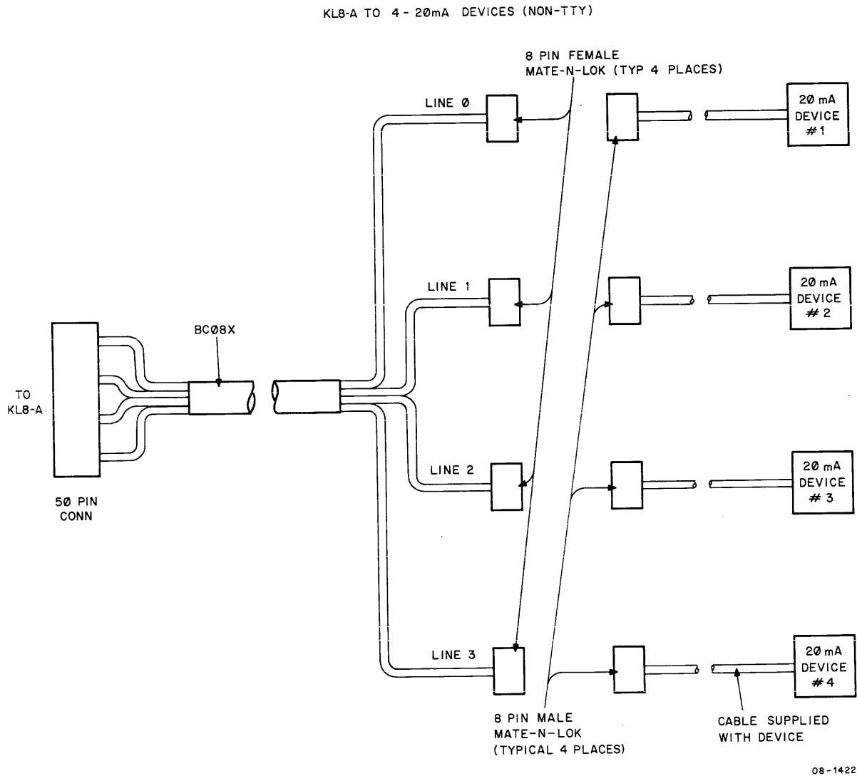
Figure 2-4 KL8-A Connected to 4 20mA Devices (Non TTY)
