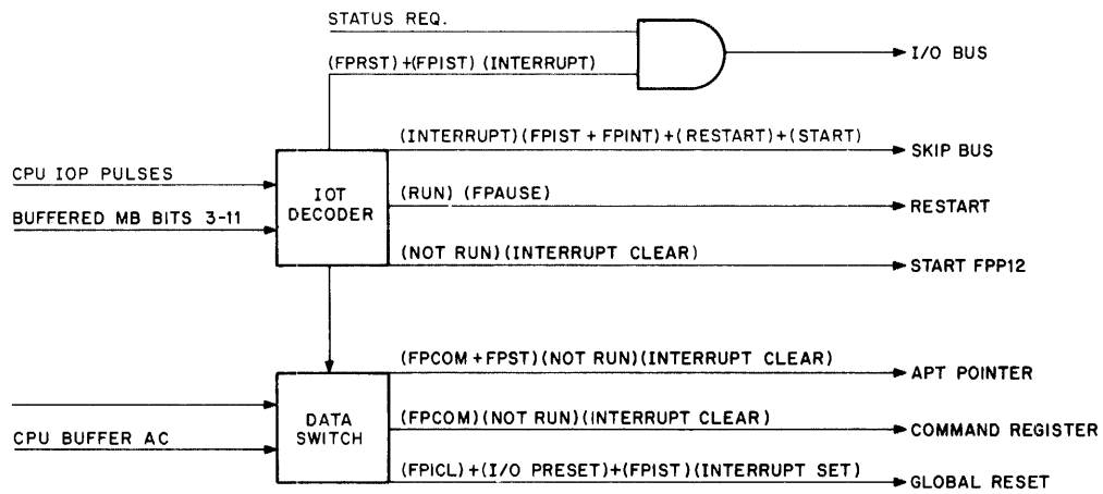
Figure 3-3 FPP12 User IOT Decoder System
