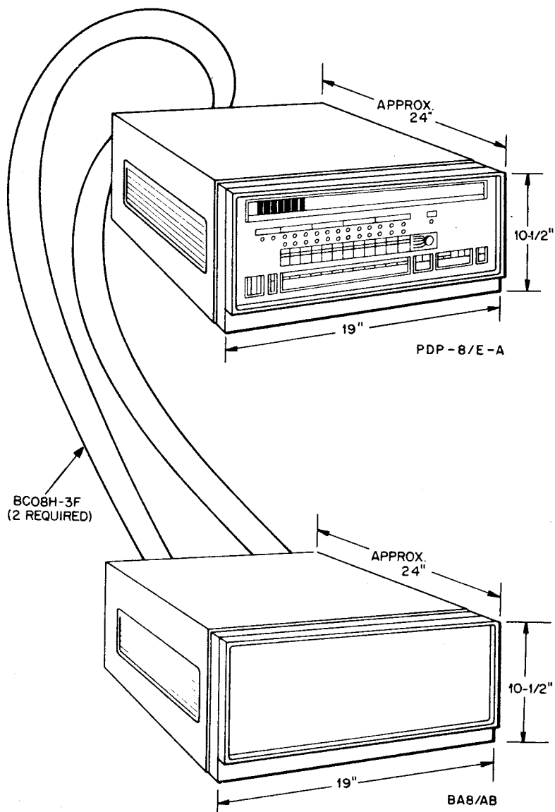
Figure 11-1 Table-Top PDP-8/E System and Expander Box
