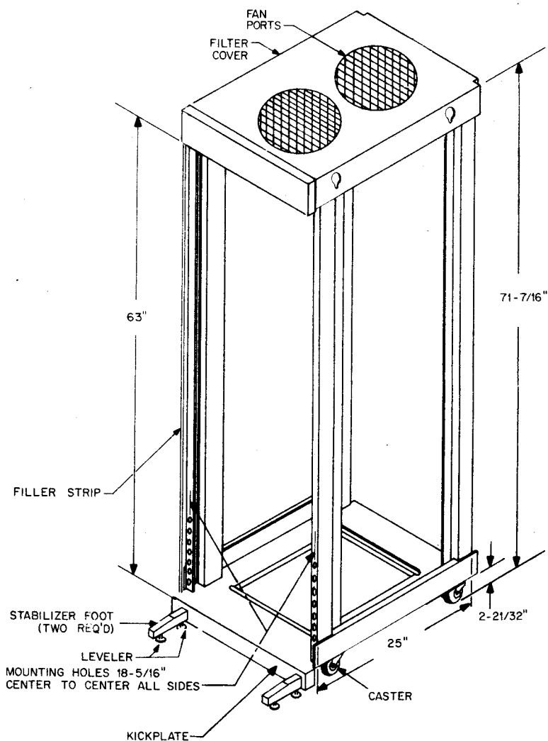
Figure 11-3 Typical H960-Series Cabinet Frame—Dimensions
