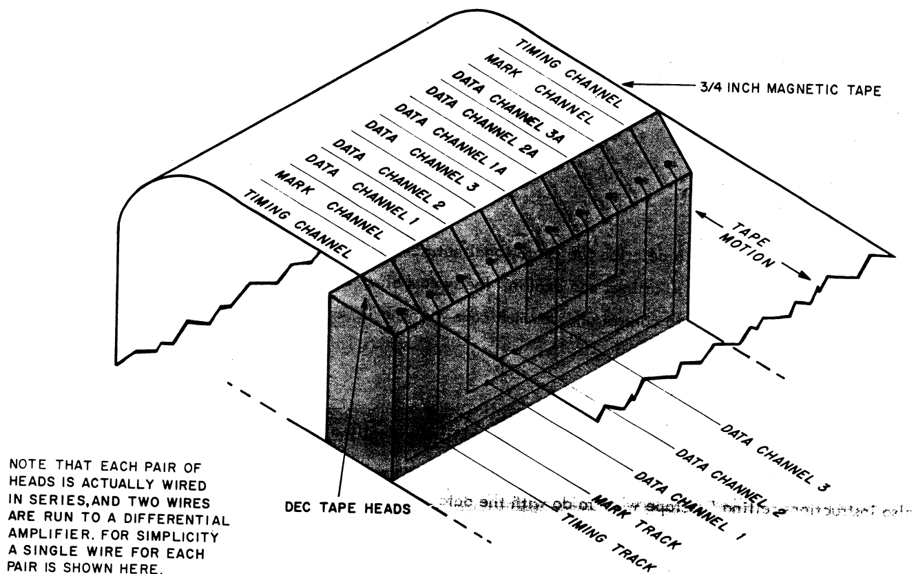
Figure 2-1 DECtape Heads and Tape Channels
