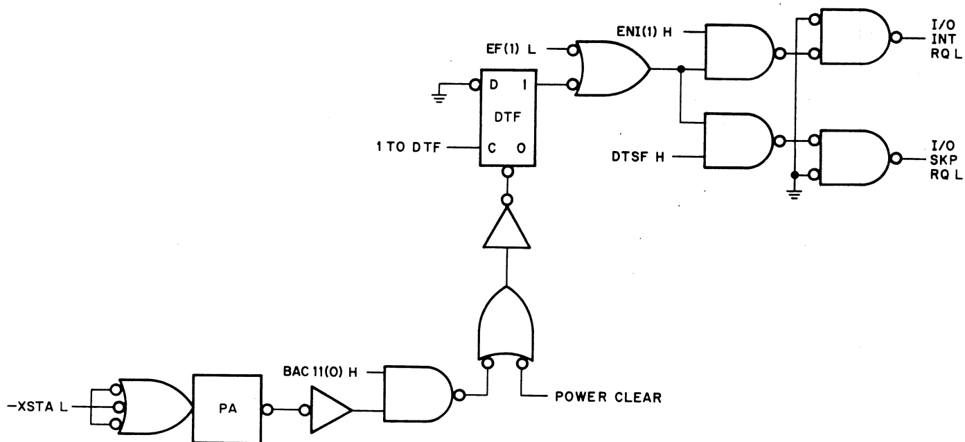
Figure 3-13 The DECtape Flag
