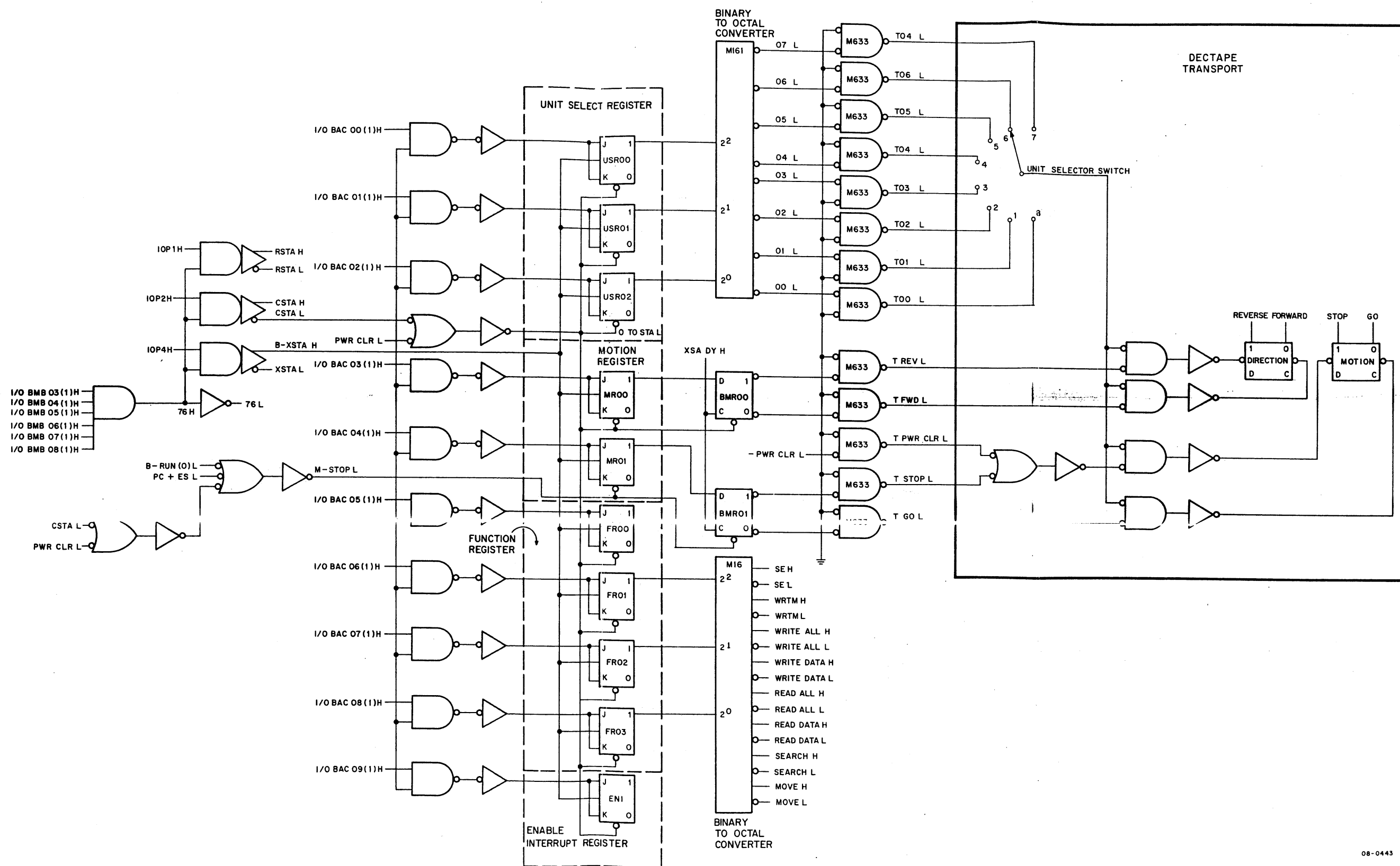
Figure 3-4 Command Register
