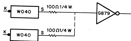
Figure 6-6 G879 Application
