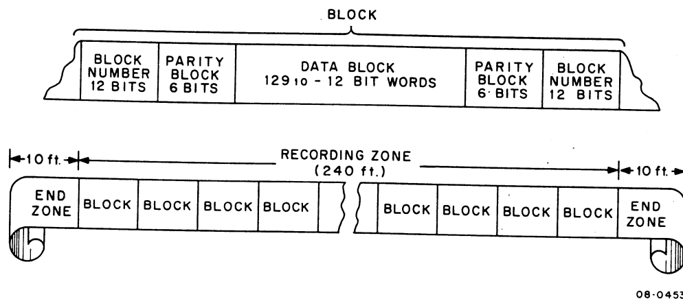
Figure 2-2 DECtape Data Blocks
