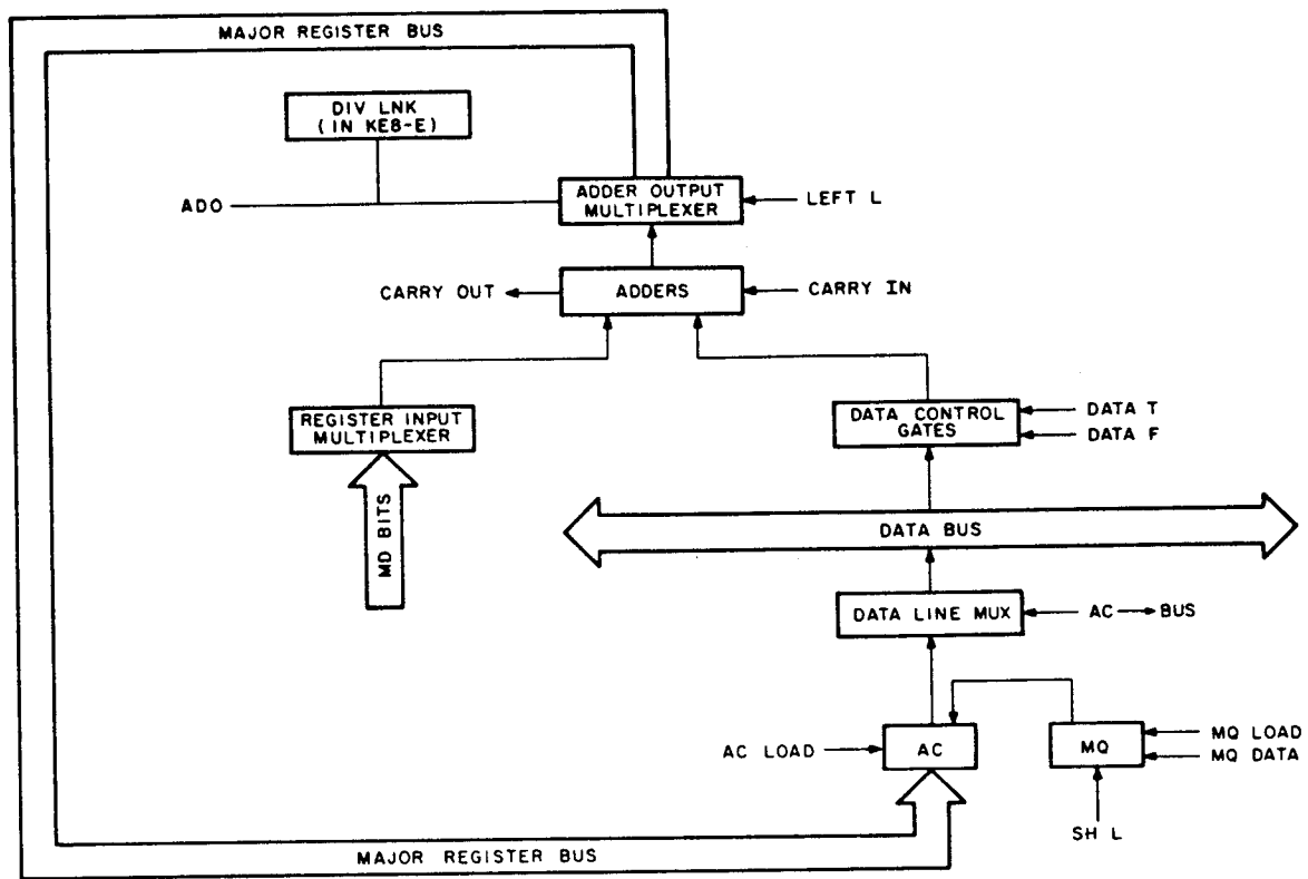
Figure 1-16 Major Registers
