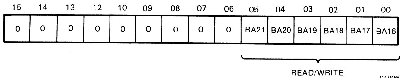
Figure 4-9 BAE Register
