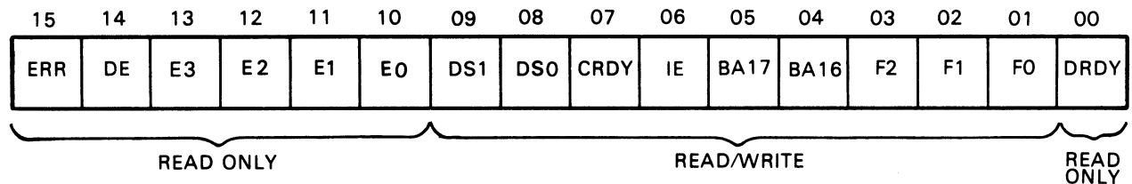
Figure 4-1 CS Register
