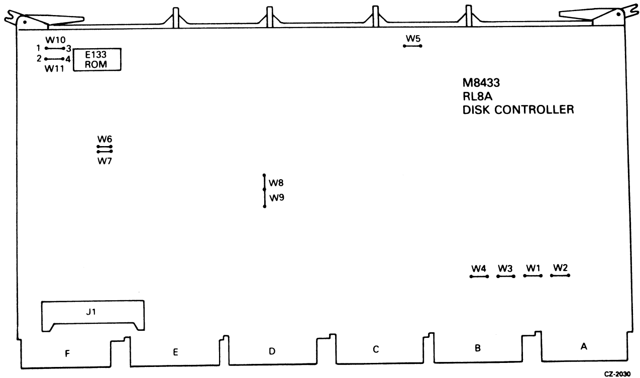
Figure 2-21 RL8A Jumpers
