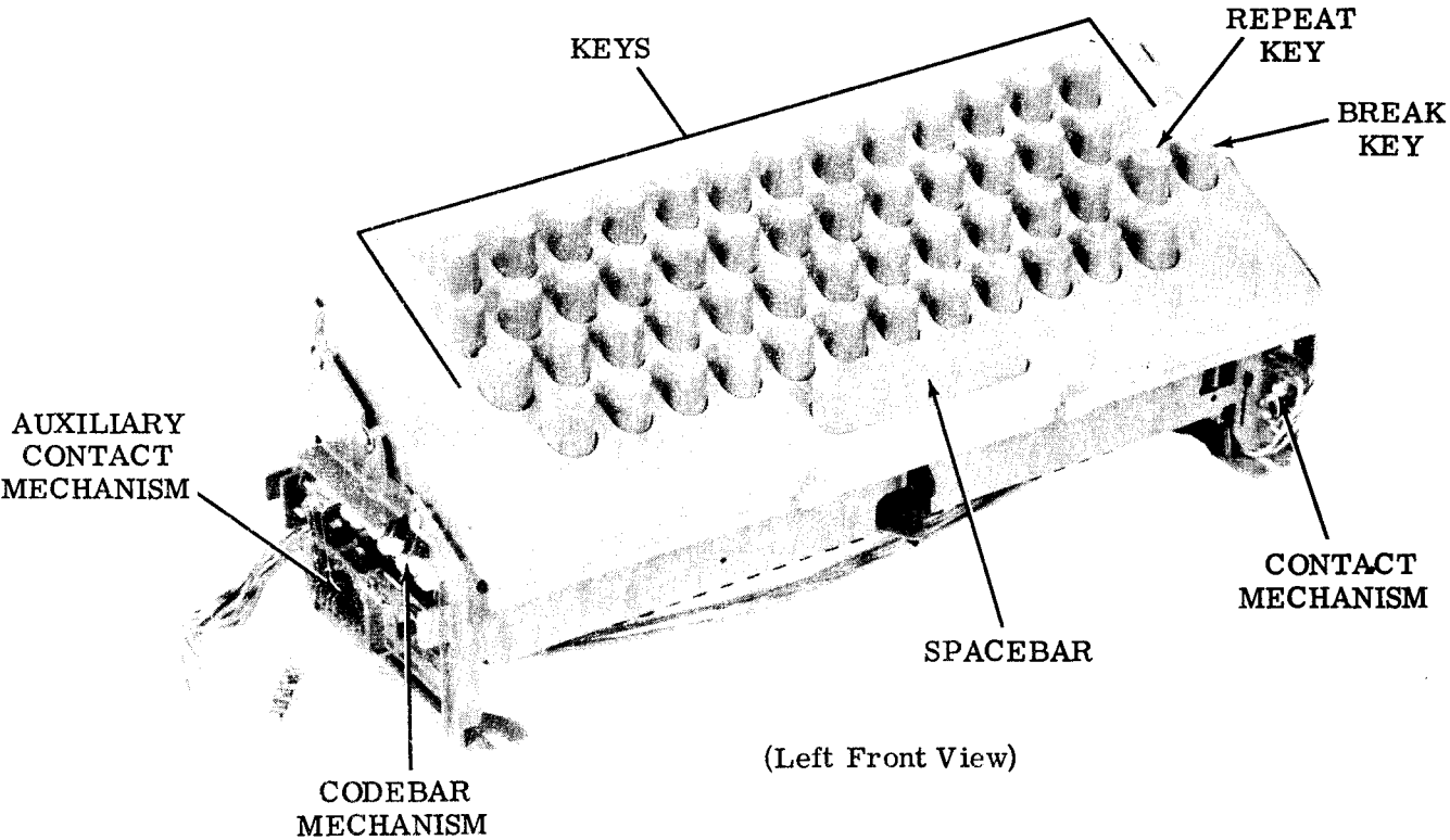
Figure 2 - Parity Keyboard
