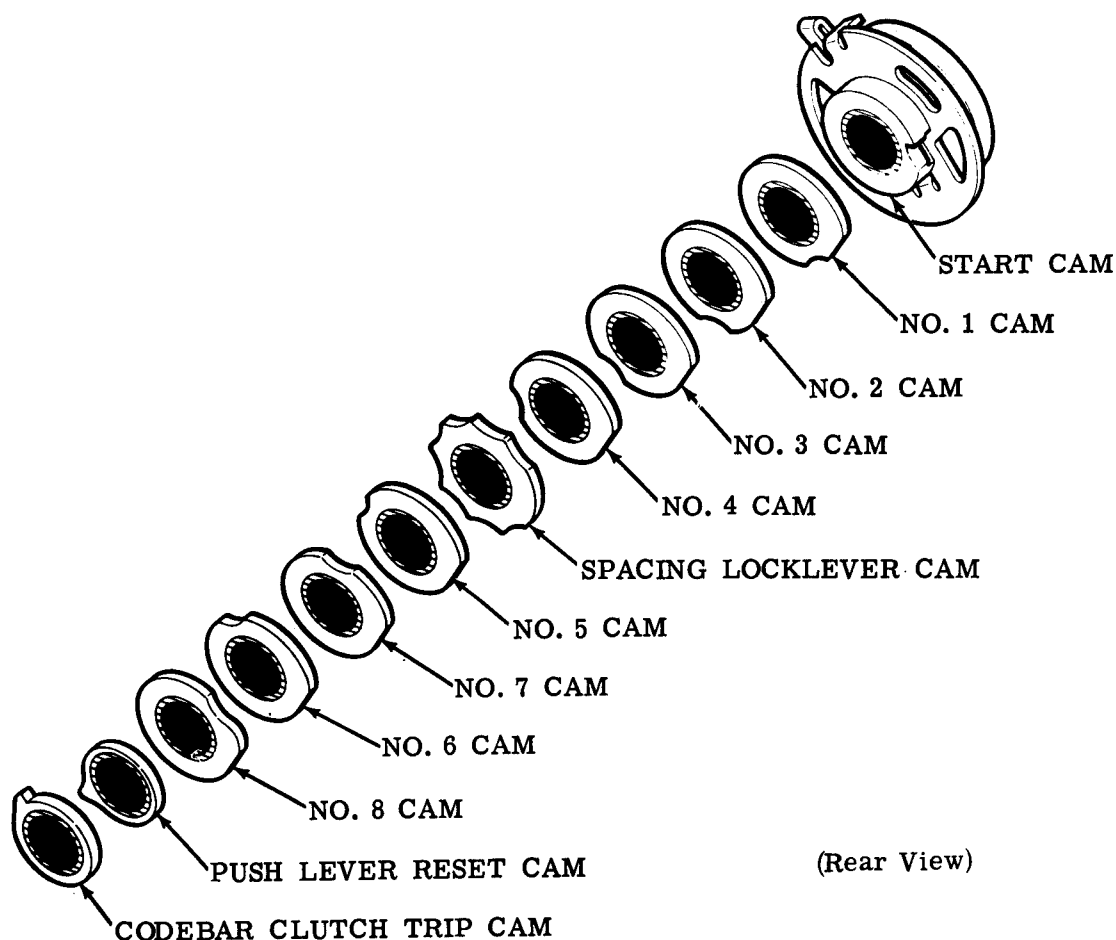
Figure 11 - Selector Cam Sleeve
