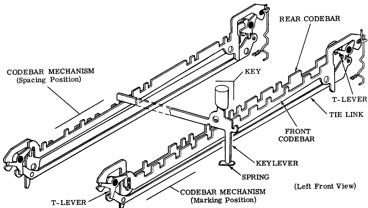
Figure 4 - Codebar Mechanism
