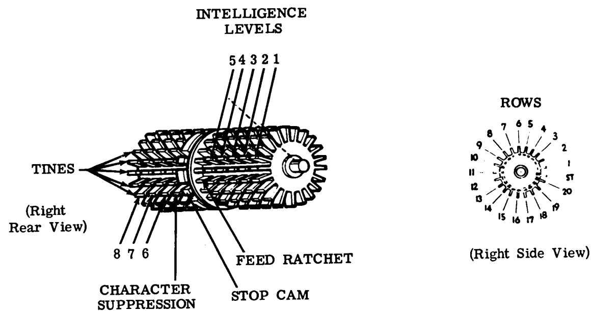
Figure 35 - Answer-Back Drum
