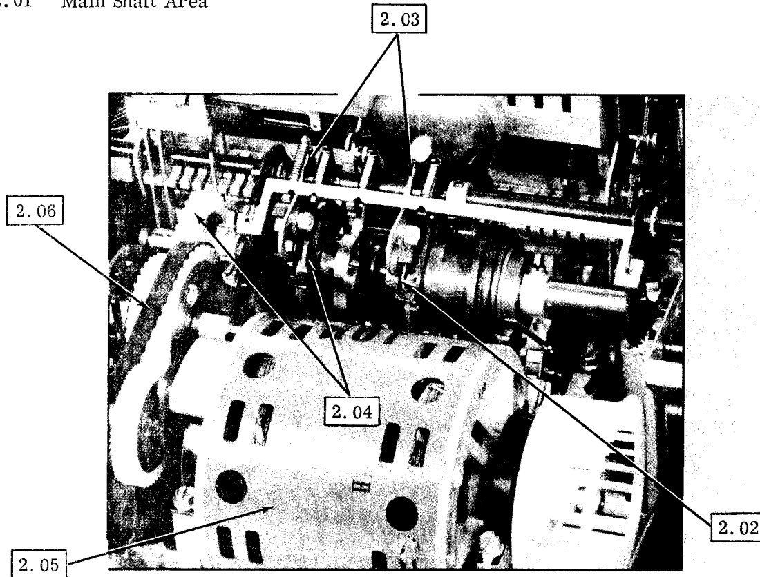
(Rear View)
