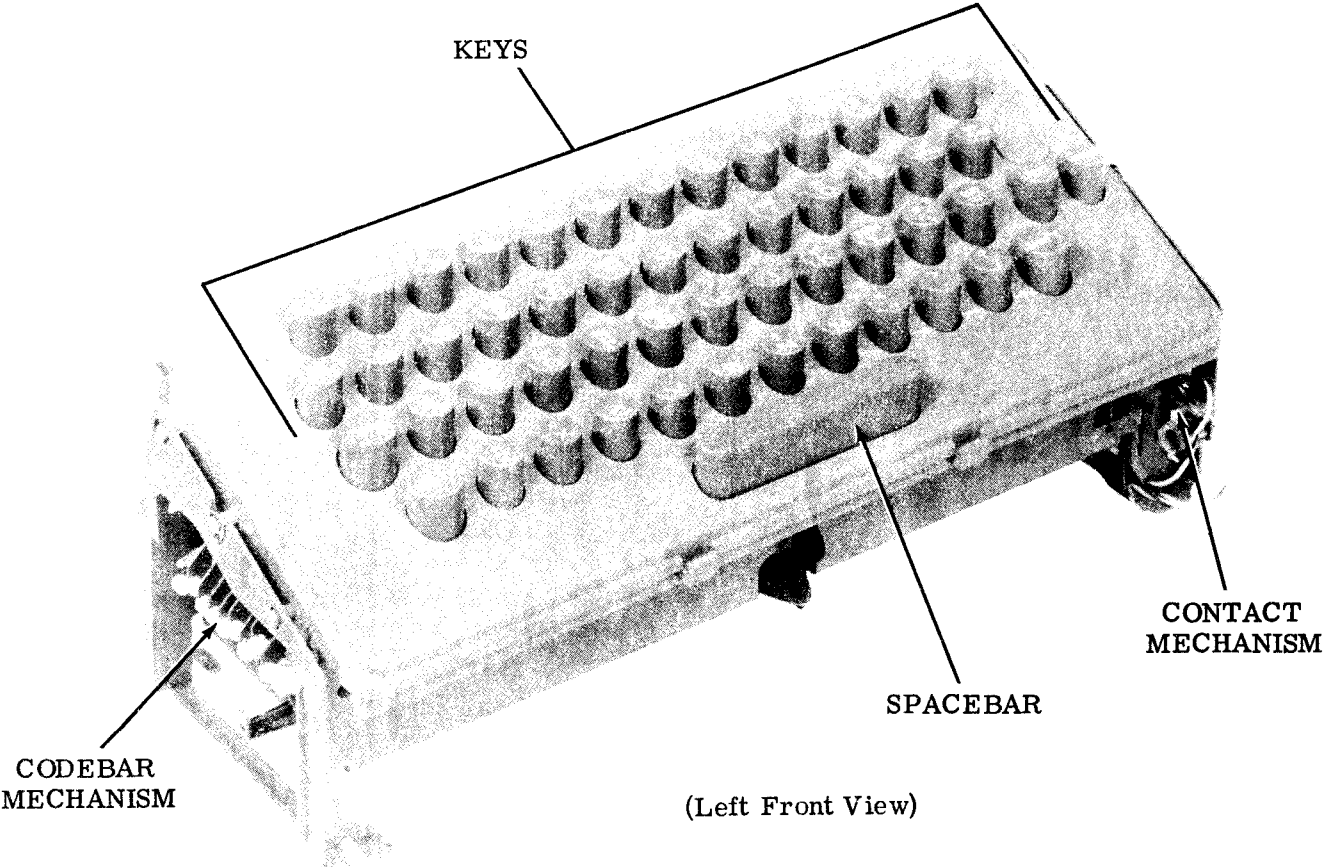
Figure 1 - Nonparity Keyboard
