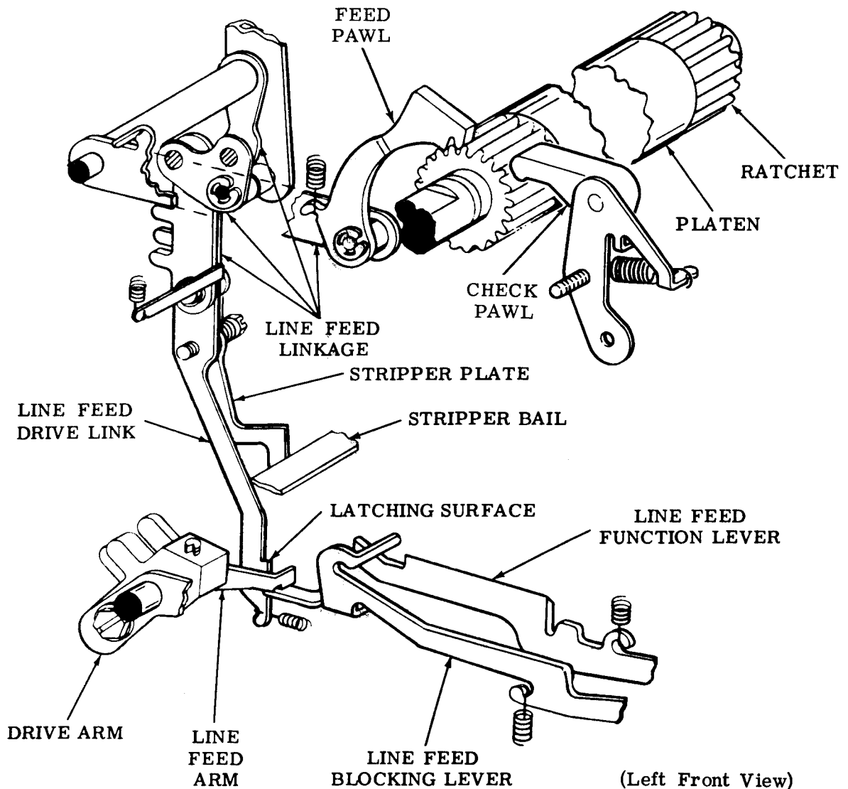
Figure 30 - Paper Feed Mechanism (Friction Feed)
