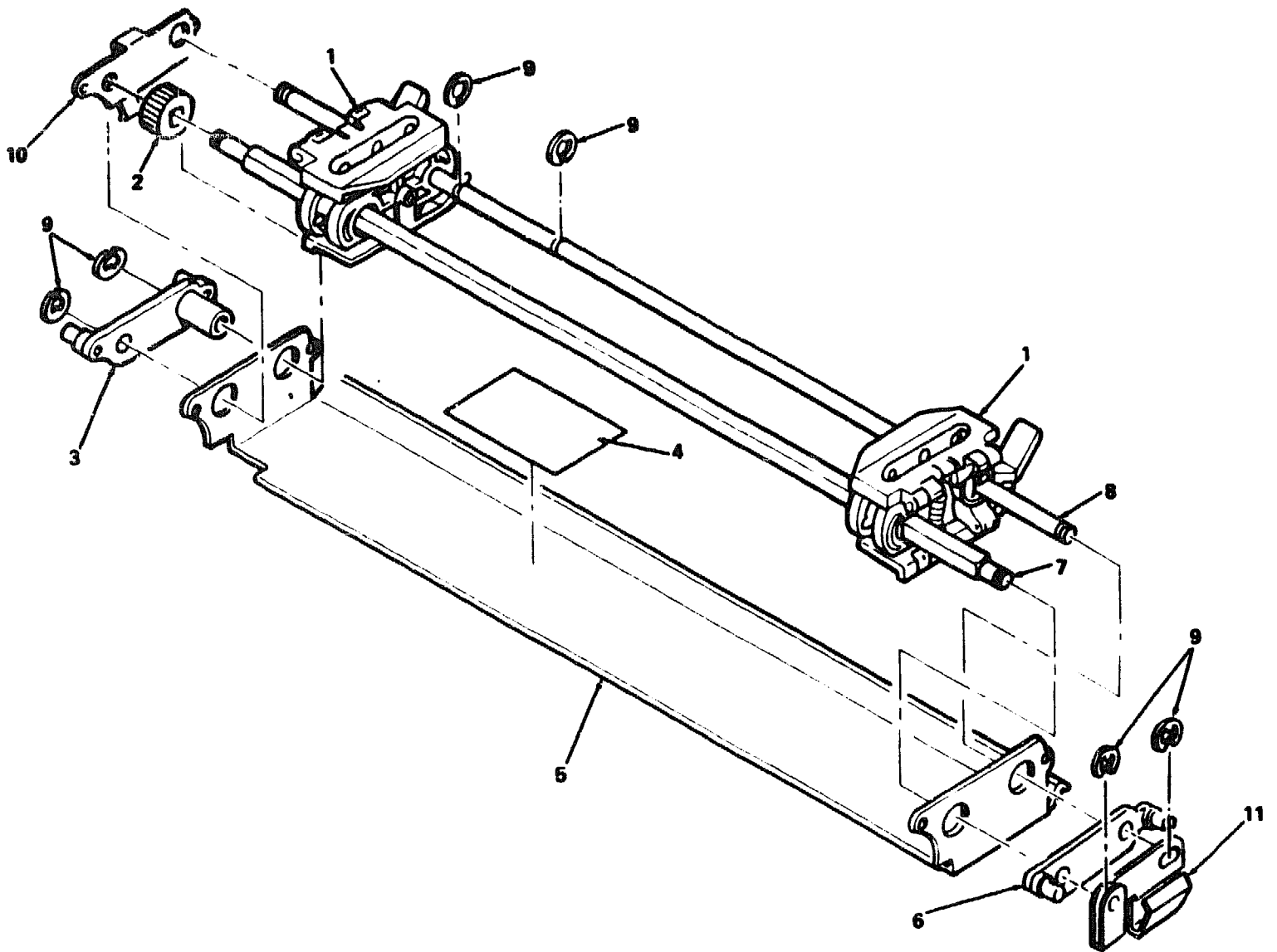
Figure 4. Tractor Assembly
