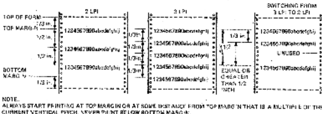
Figure 4-7 Top/Bottom Margins and Pitches
