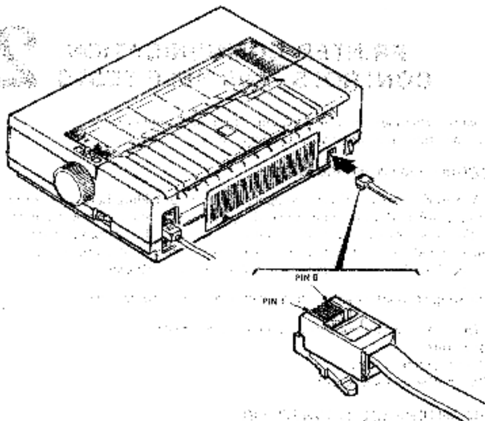
Figure 2-1 EIA MMJ Serial Interface Connector
