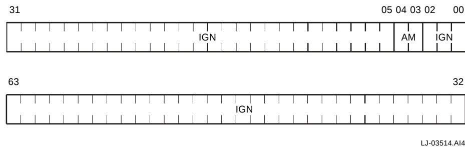
Figure 5–42 Alternate Mode (ALT_MODE) Register
