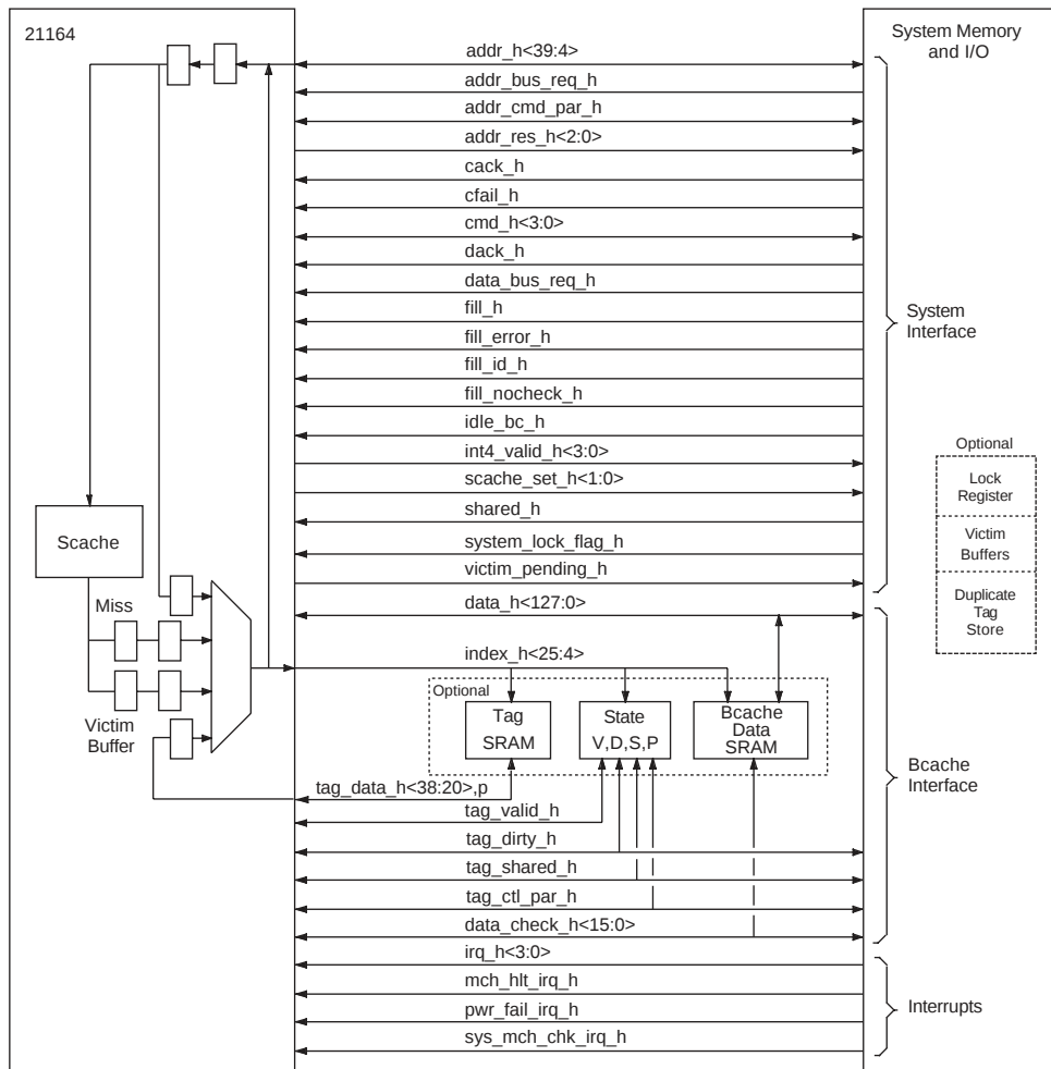
Figure 4–1 21164 System/Bcache Interface
