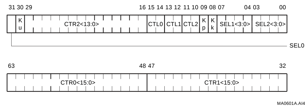
Figure 5–26 Performance Counter (PMCTR) Register
