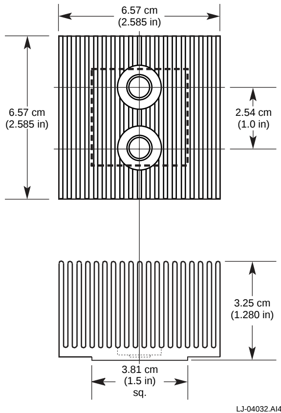
Figure 10–1 Type 1 Heat Sink
