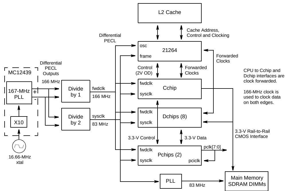
Figure 4–2 Clock Distribution
