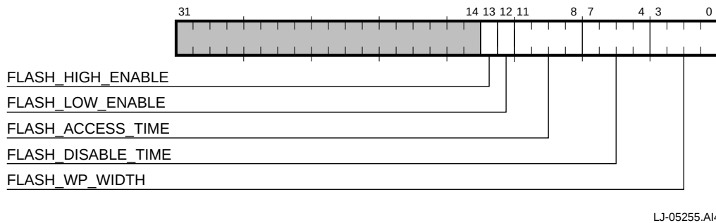
Figure 5–5 Flash Control Register
