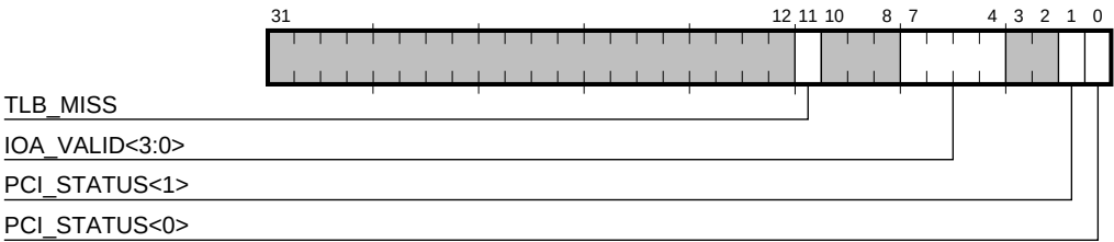
Figure 5–14 Status Register
