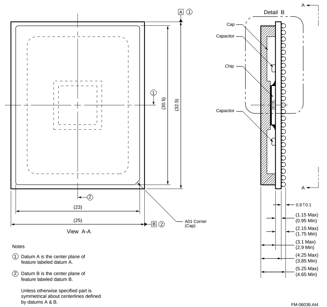
Figure 8–1 474-Pin BGA Package
