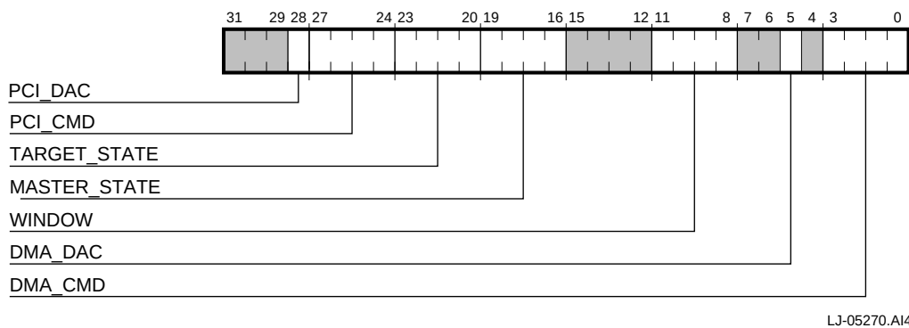
Figure 5–20 PCI Error Register 0
