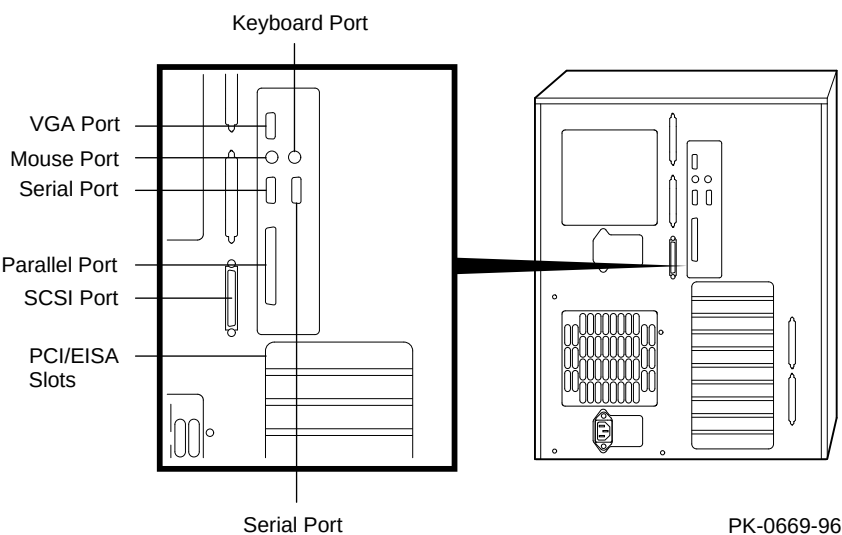
Figure 7 AlphaServer 1000A Pedestal System Rear View
