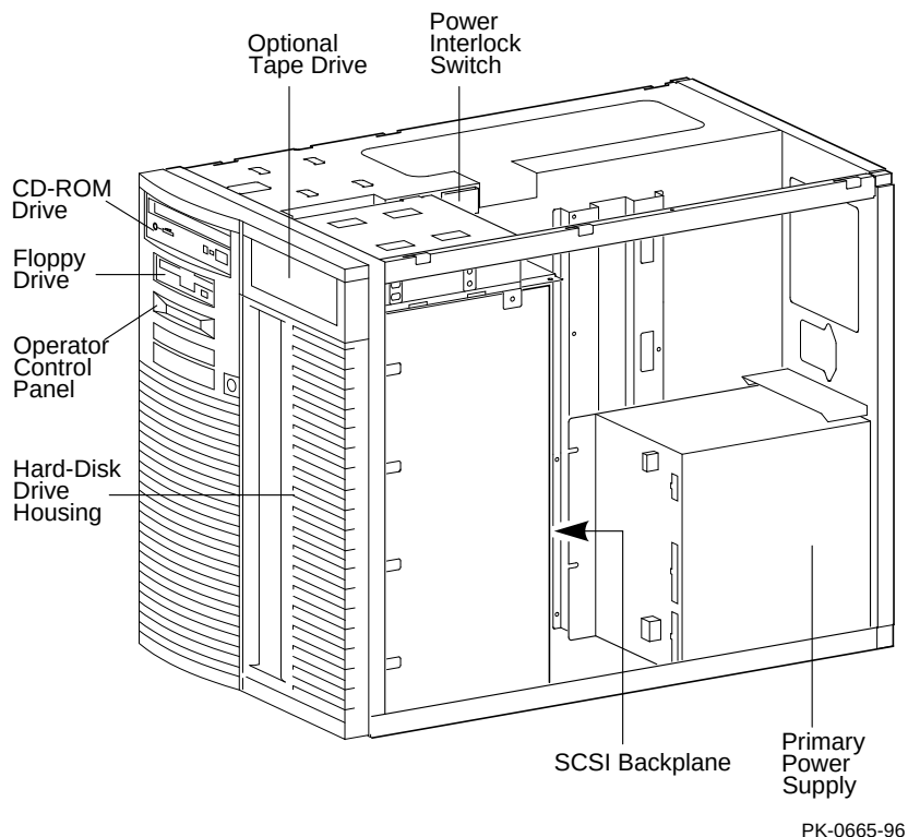
Figure 5 AlphaServer 1000A Pedestal System Front View
