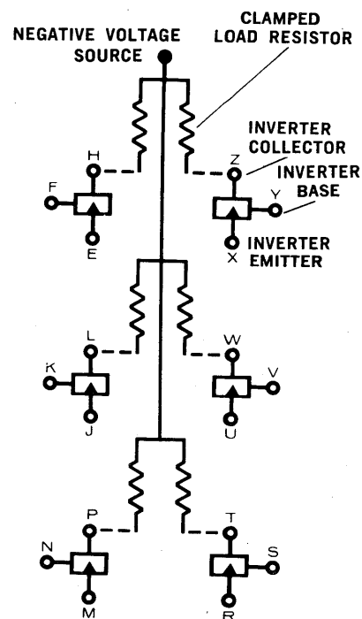
4106 INVERTER
