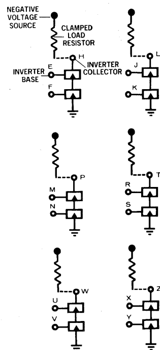
6123 INVERTER
