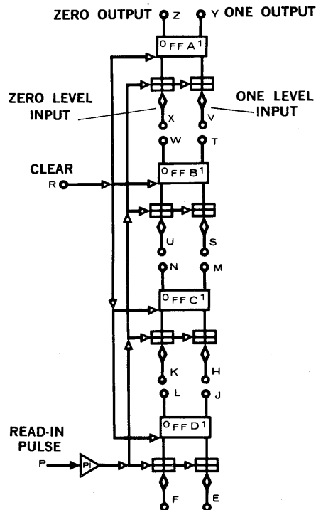
4218 SET-RESET FLIP-FLOPS
