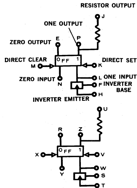
1209 DUAL FLIP-FLOP
