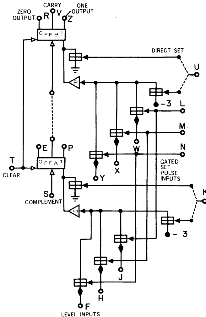
4204 BUFFER
