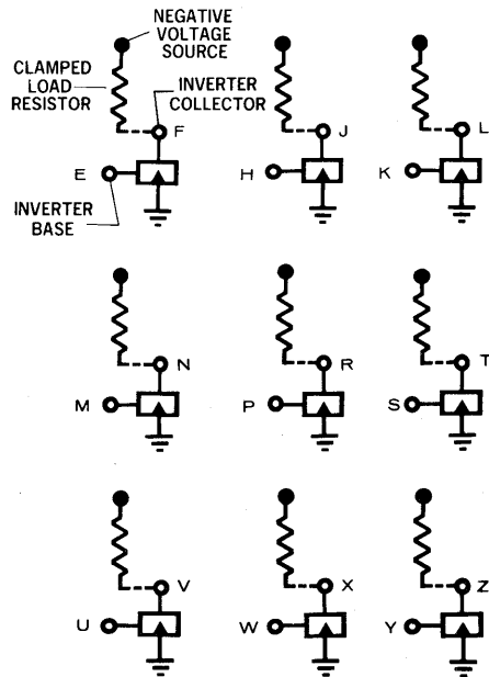
6102 INVERTER
