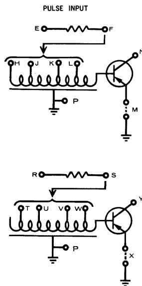
1311 DELAY LINE (UP TO 200 NANoseconds)
