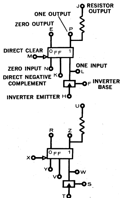
1204 DUAL FLIP-FLOP
