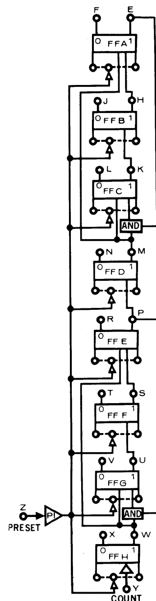
4225 AS A BCD COUNTER
