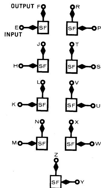
1703 SWITCH FILTER
