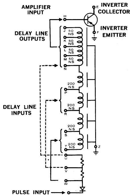
1310 DELAY LINE (UP TO 1 MICROSECOND)
