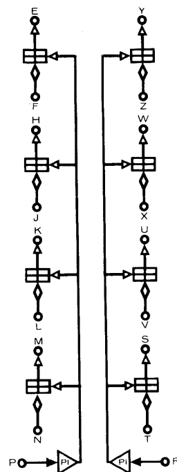
4128 CAPACITOR-DIODE GATE
