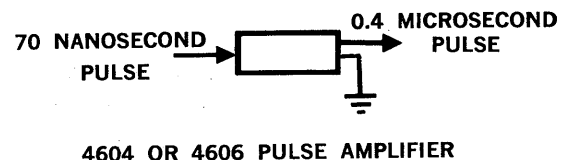
4604 OR 4606 PULSE AMPLIFIER
