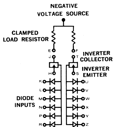
1110 NEGATIVE DIODE NOR
