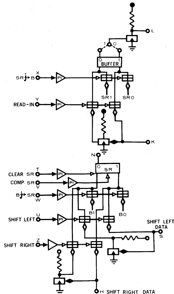
42281 ASSEMBLER
