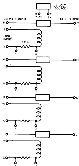
1804 RELAY PULSER
