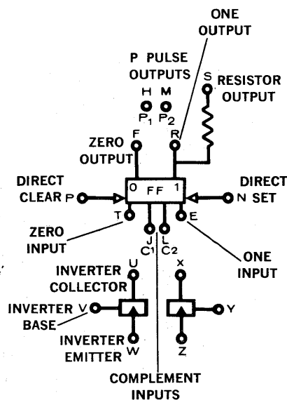
6202 FLIP-FLOP
