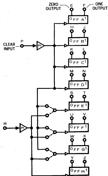
6227 — UNBUFFERED FLIP-FLOPS
