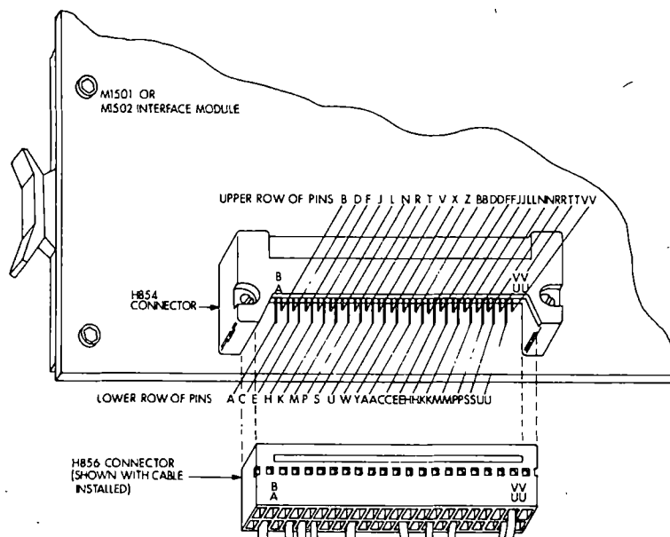
Figure 3-12. Input/Output Connector Pin Layout
