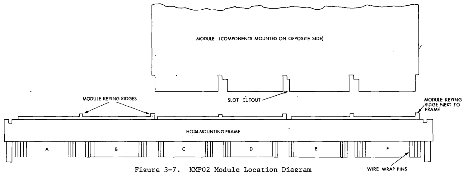
Figure 3-7. KMP02 Module Location Diagram
