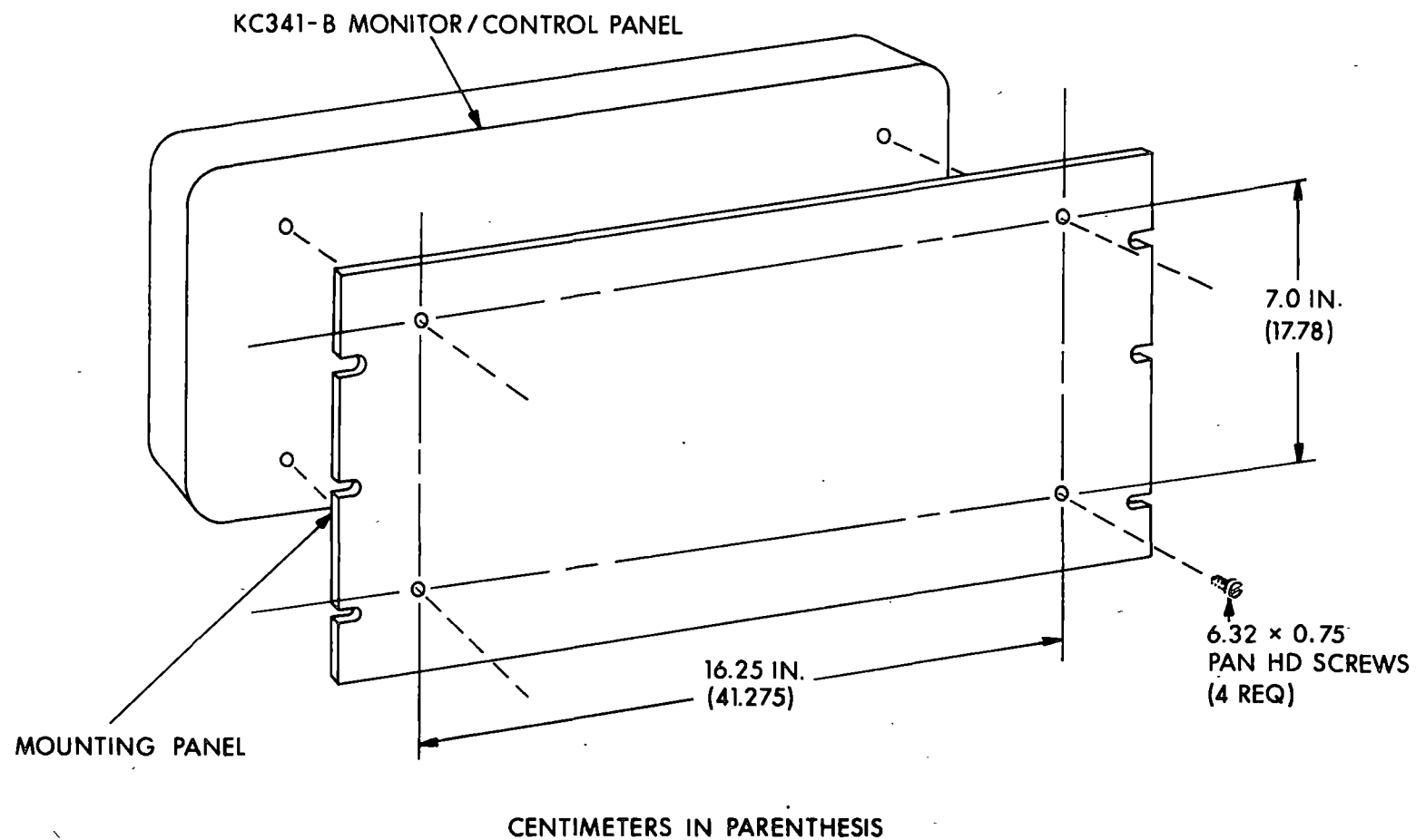
Figure 3-6. KC341-B Mounting Panel Hole Dimensions
