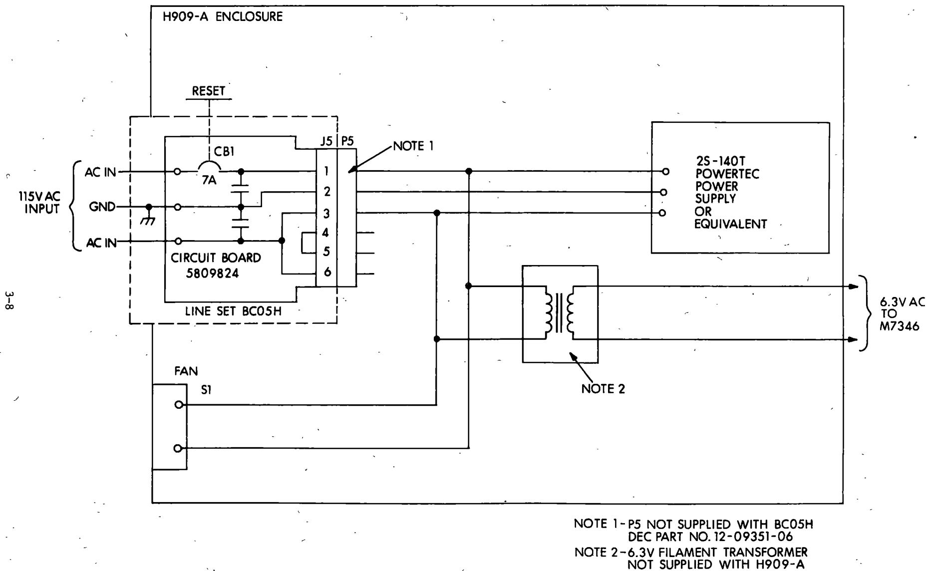
Figure 3-4. H909-A Enclosure Typical AC Wiring Diagram
