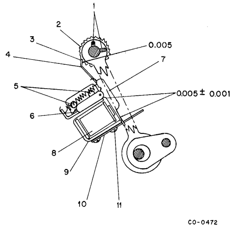
Figure 5-14 Forward Index Magnet Armature
