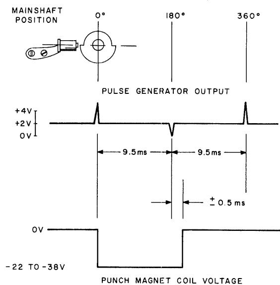
Figure 5-12 Electrical Parameters
