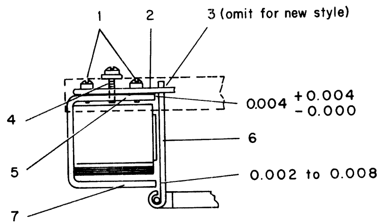
Figure 5-15 Punch Magnet
