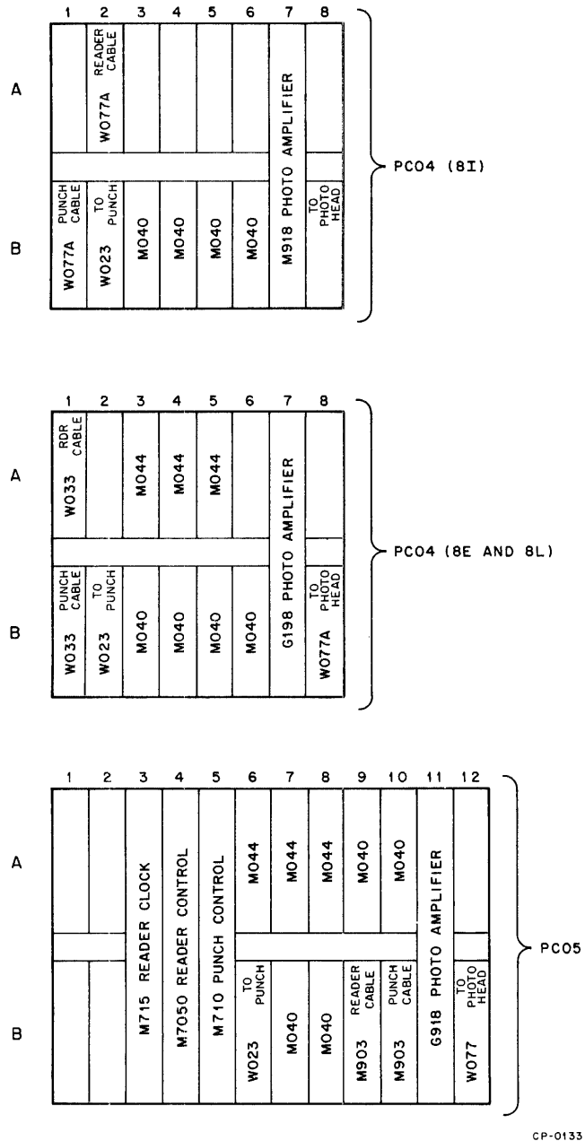
Figure 2-1 PC04/PC05 Module Locations
