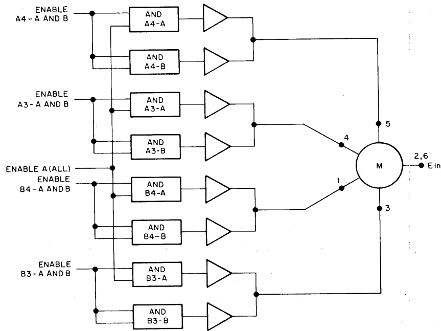
Figure 3 Motor Drive Circuit, Simplified Block Diagram
