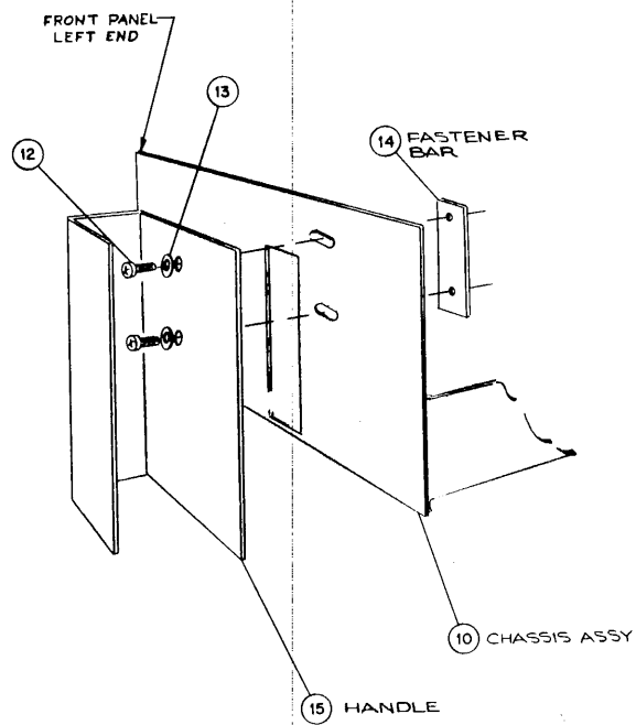
Figure 12 Handle Assembly
