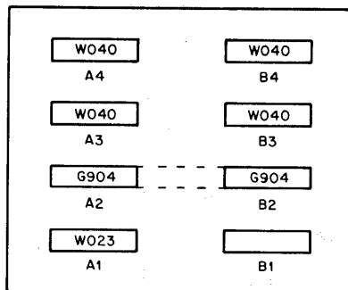
Figure 6 FLIP CHIP Module Connector Block
