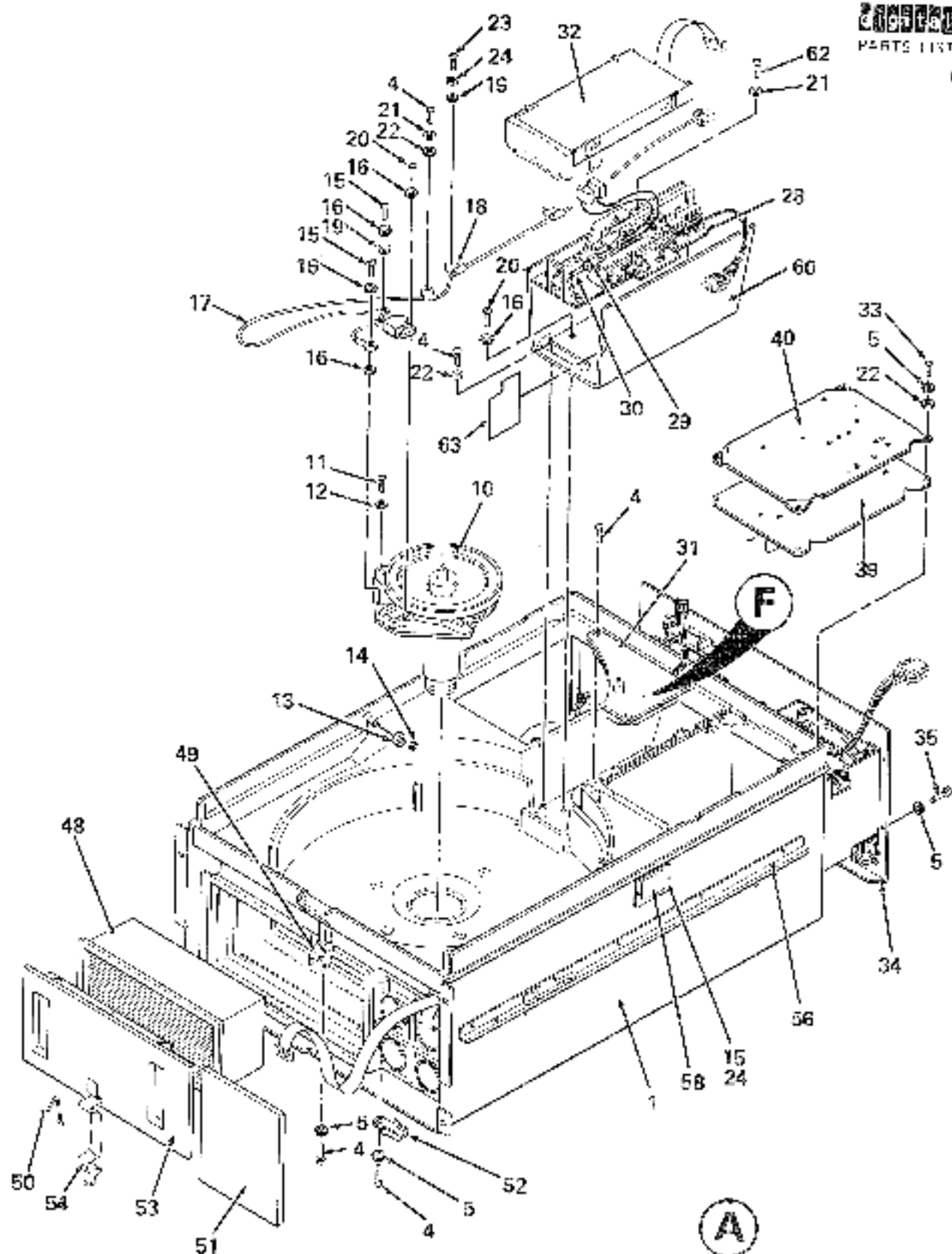
Figure 3. RLD1 Disk Drive Assembly (Sheet 2 of 7)
