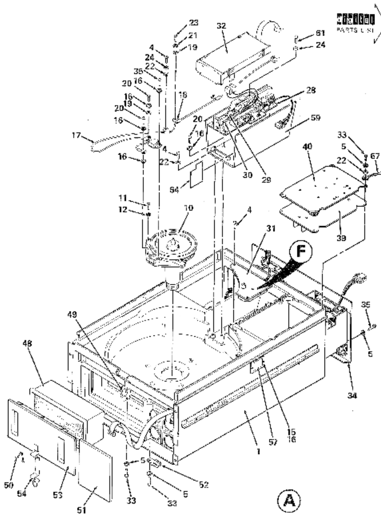
Figure 3. RL02 Disk Drive Assembly (Sheet 2 of 7)
