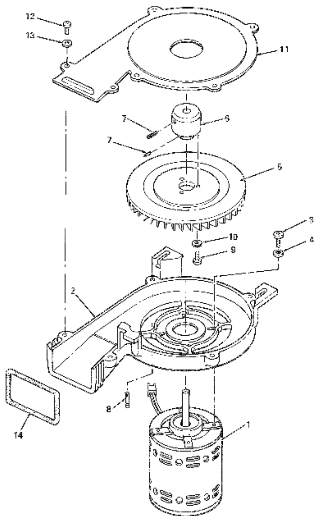
Figure 4. Disk Motor Assembly
