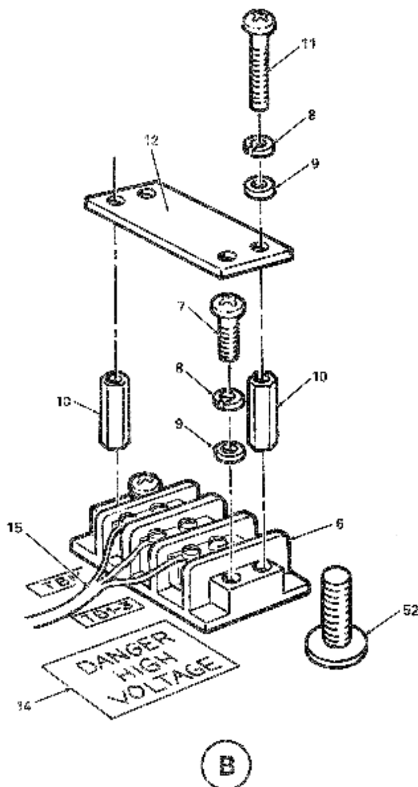
Figure 7. Enclosure Assembly (Sheet 3 of 6)
