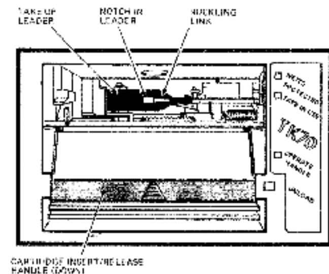
Figure 3-2: Inspecting the Drive Leader
