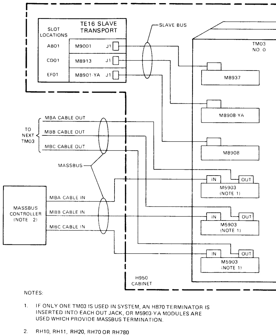
Figure 3-2 TM03 Cabling to a TE16 Slave Transport in an H950 Cabinet
