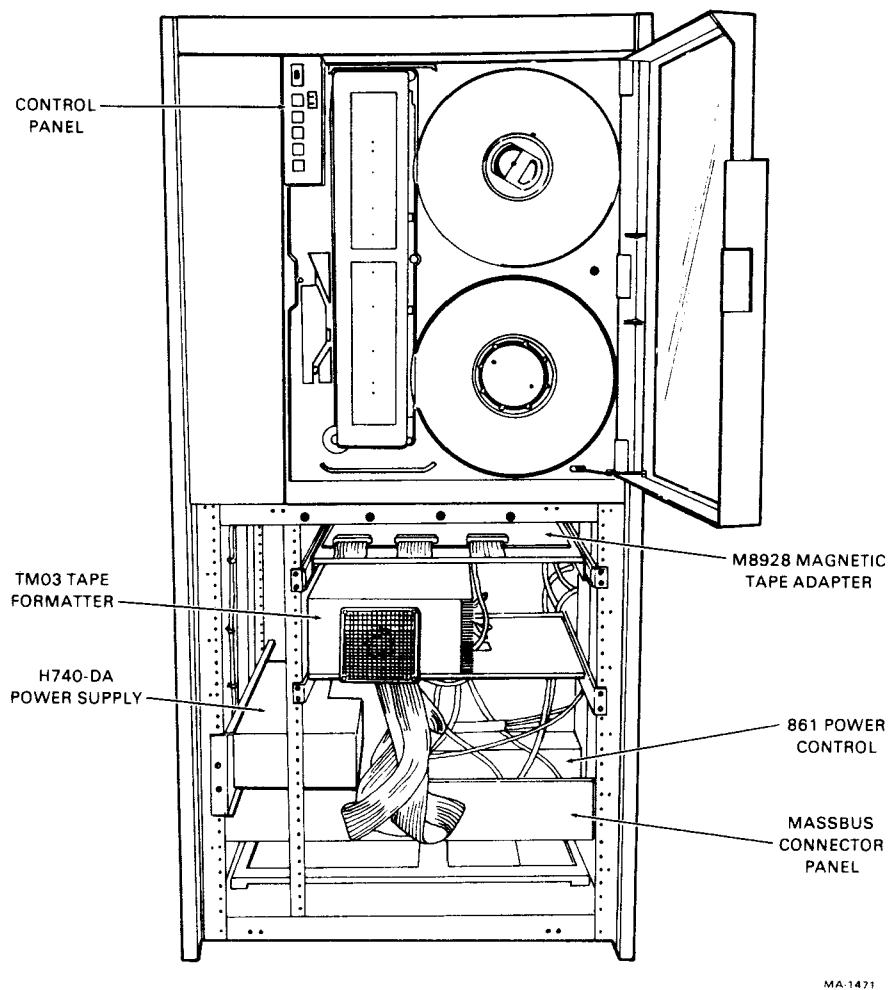
Figure 1-3 TM03 with TU45 Tape Transport in H9500 Corporate Cabinet
