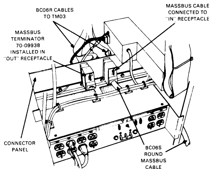
a. Connector Panel in TU45 Transport
