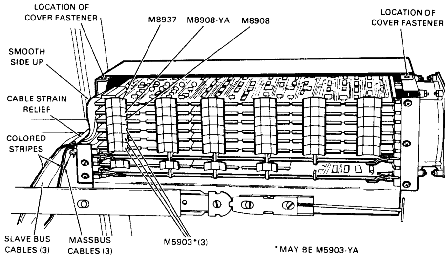
Figure 3-1 TM03 Formatter with Cover Removed
