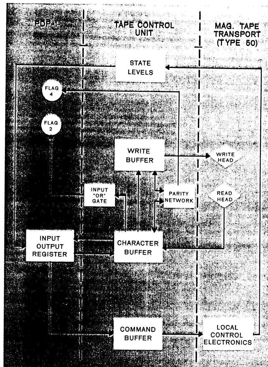
Magnetic Tape Control Block Diagram
