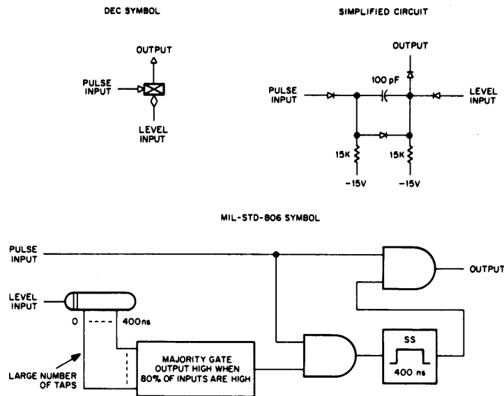
Figure 3-5 DCD Gate
