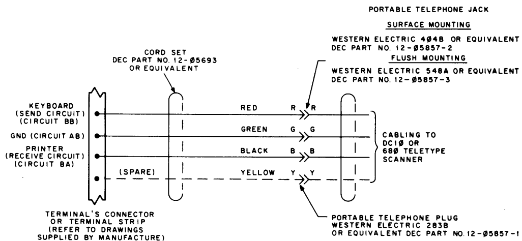
Figure 6-2 EIA Interface
