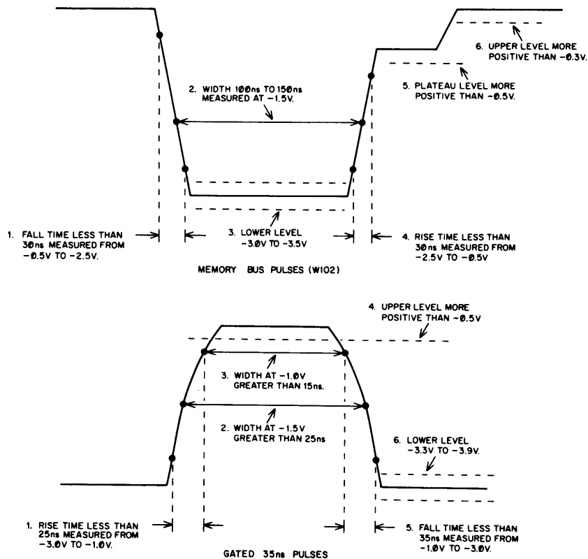
Figure 11-3 Pulses
