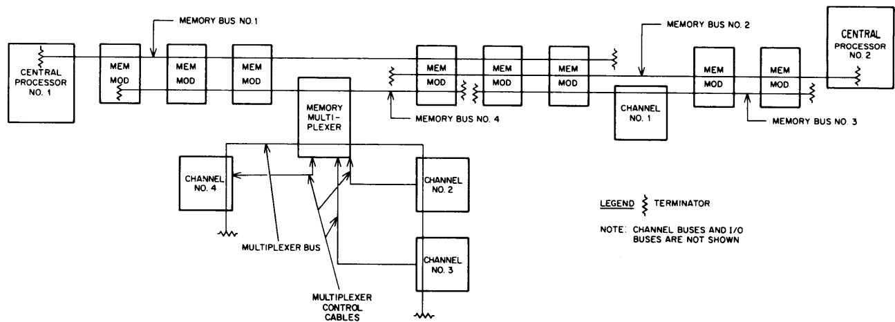
Figure 7-1 Possible Memory Bus Arrangement
