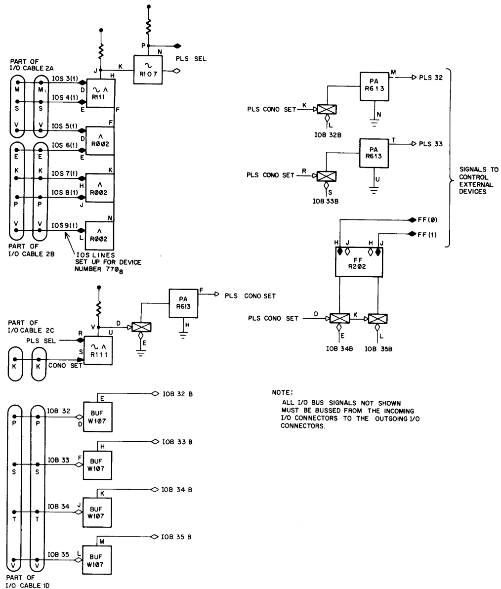
Figure 2-7 Control Device
