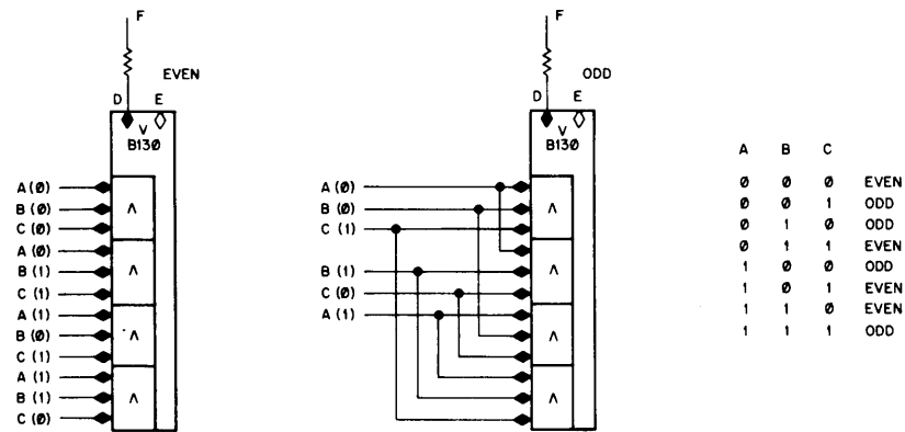
Figure 4-3 B130 Connections, Odd and Even Parity
