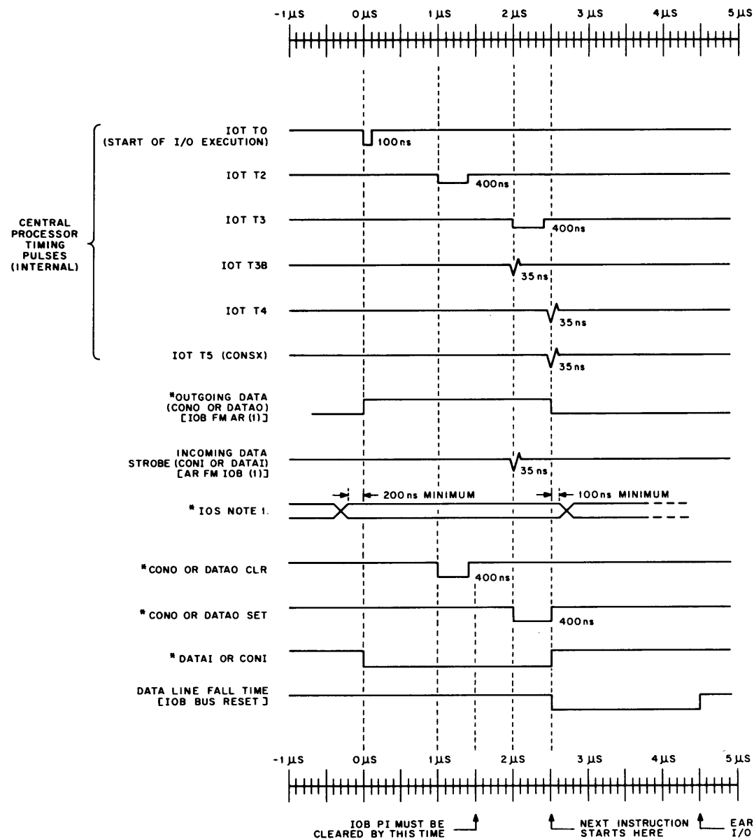
Figure 2-4 I/O Bus Timing
