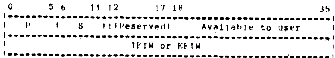
Two-word global byte pointer format
