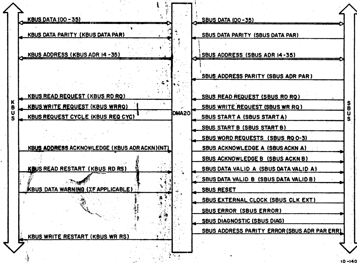
Figure 2-2 External Memory System Interface
