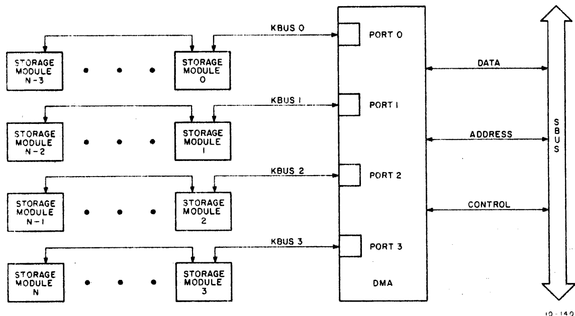
Figure 1-1 Typical System Configuration
