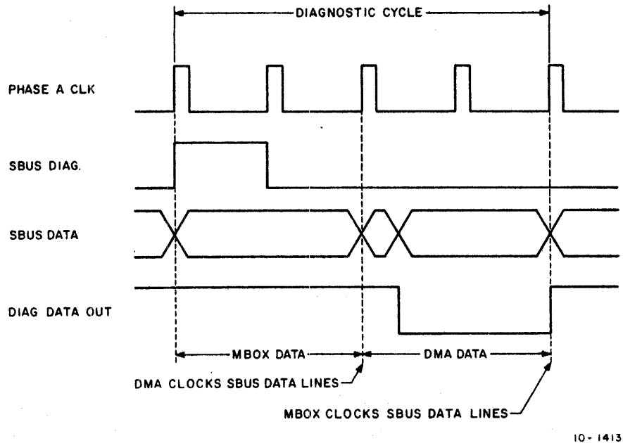
Figure 2-11 Diagnostic Cycle Timing
