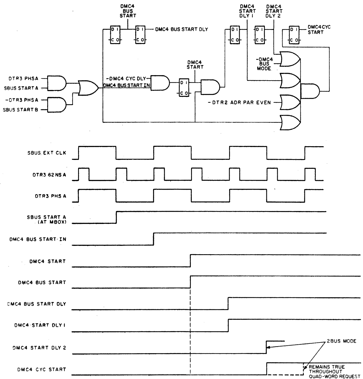
Figure 3-7 Start Logic and Timing
