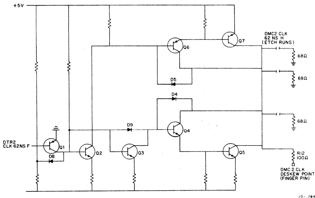
Figure 3-2 Simplified Clock Driver and Etch Runs
