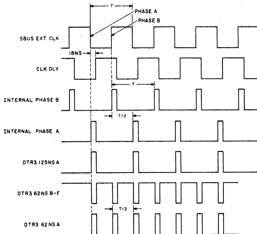
Figure 3-1 Clock Logic and Timing
