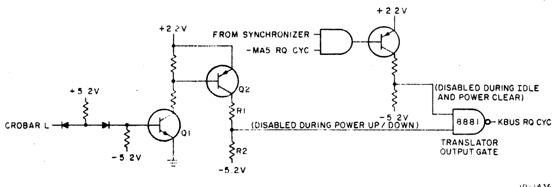
Figure 3-13 Simplified Crobar Logic
