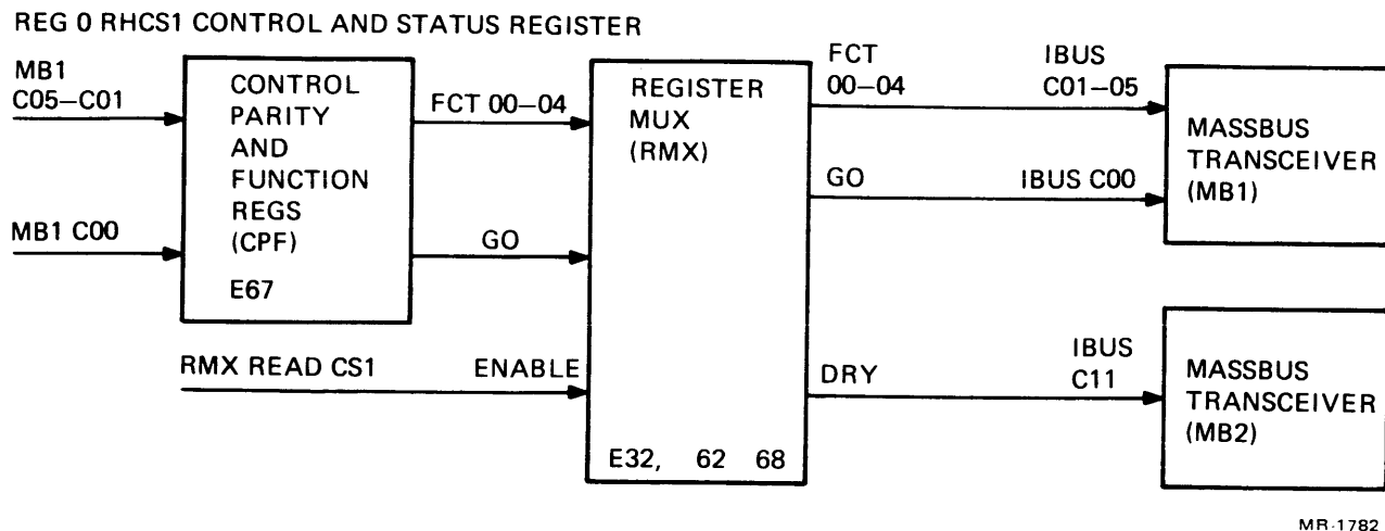
Figure 5-4 REG 0 (RHCS1) Control and Status Register Circuit Block Diagram
