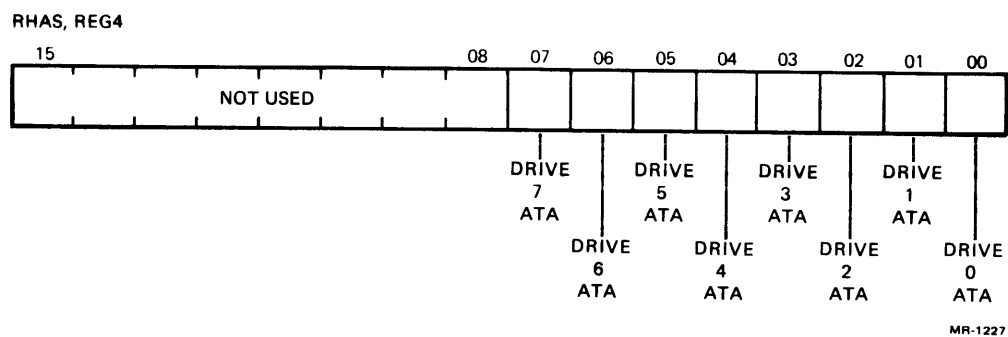
Figure 4-7 RHAS (REG 4) Bit Map
