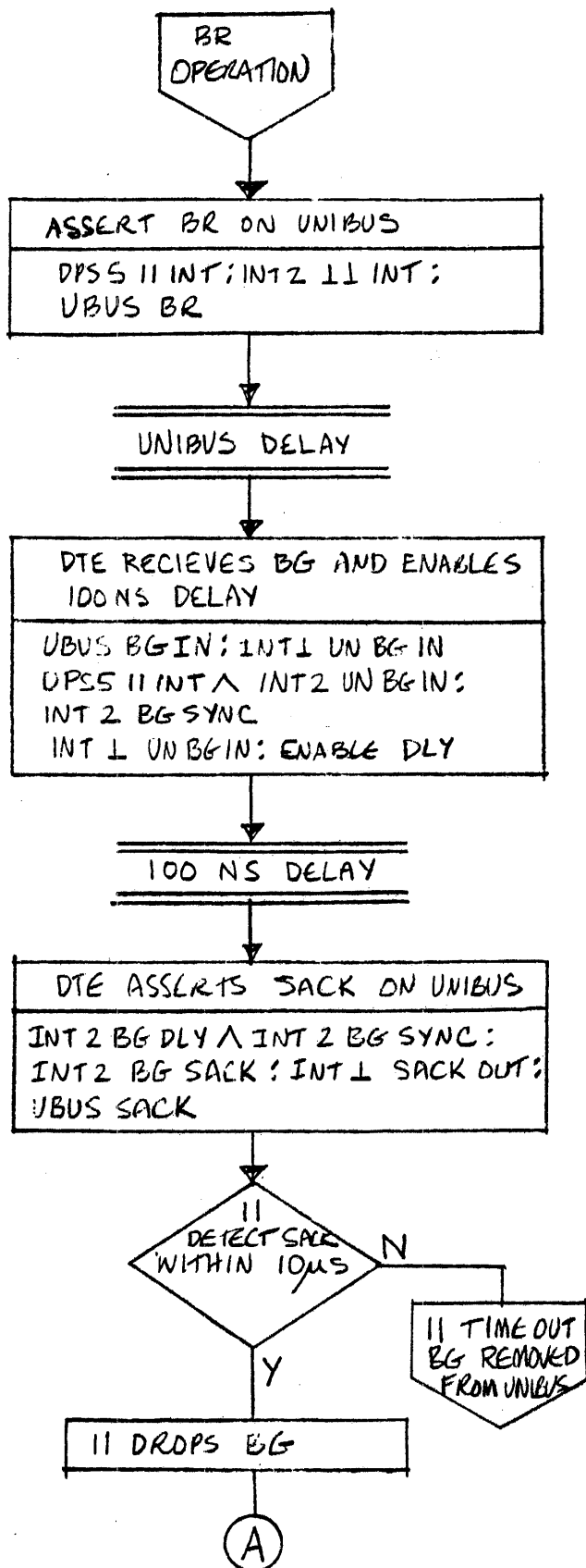
FIGURE 3, BR REQUEST OPERATION SH 1 OF 1
