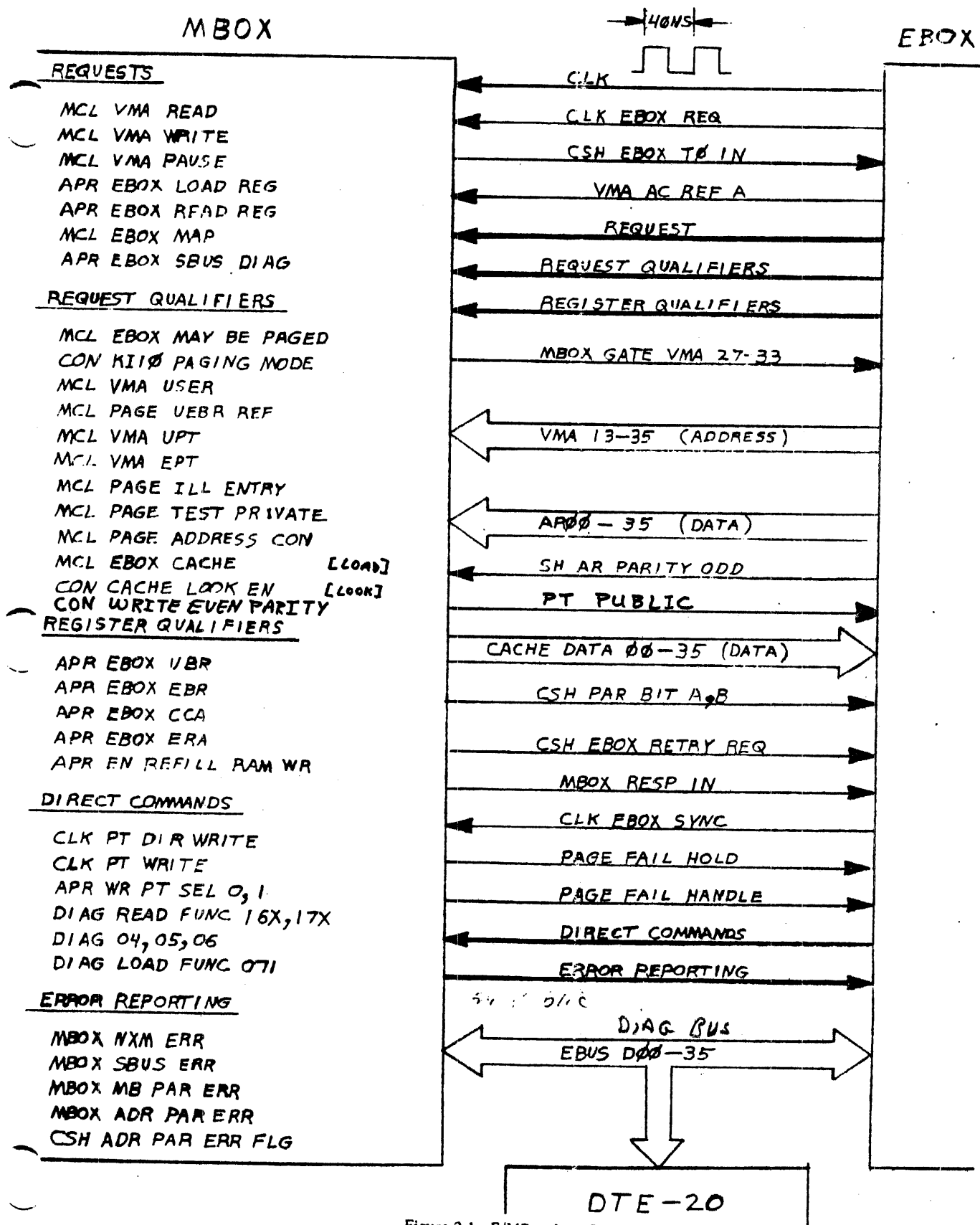
Figure 2-1 E/MBox Interface
