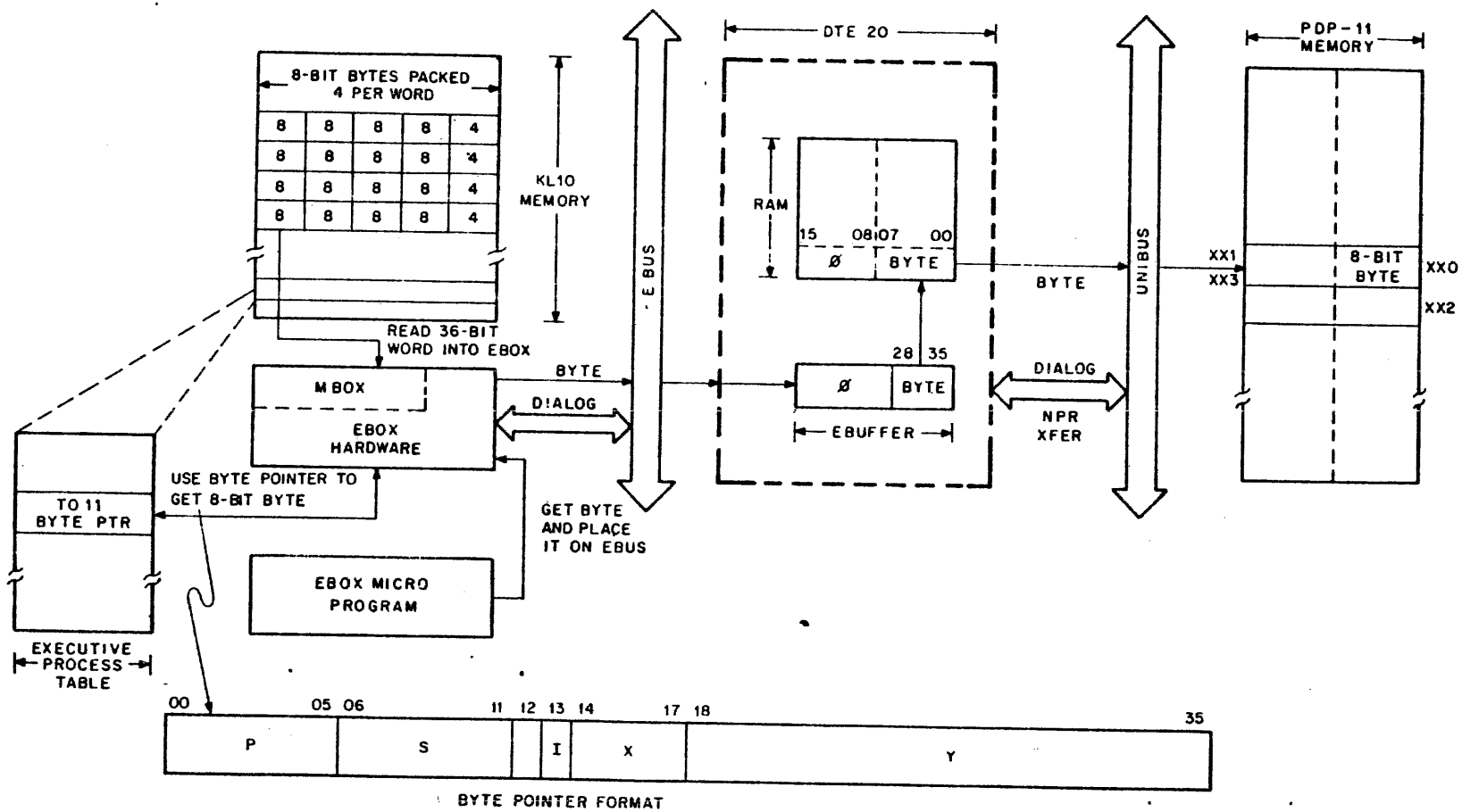
Figure 1-6 TO11 Byte Transfer Overview
