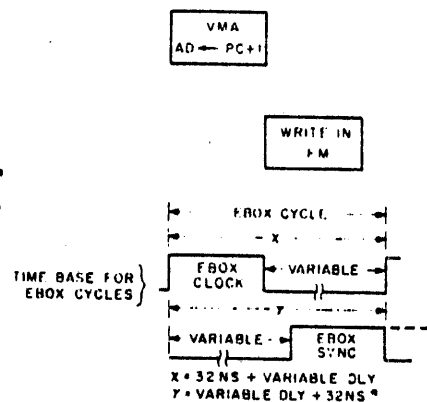
Basic Machine Cycle Overview (Sheet 1)
