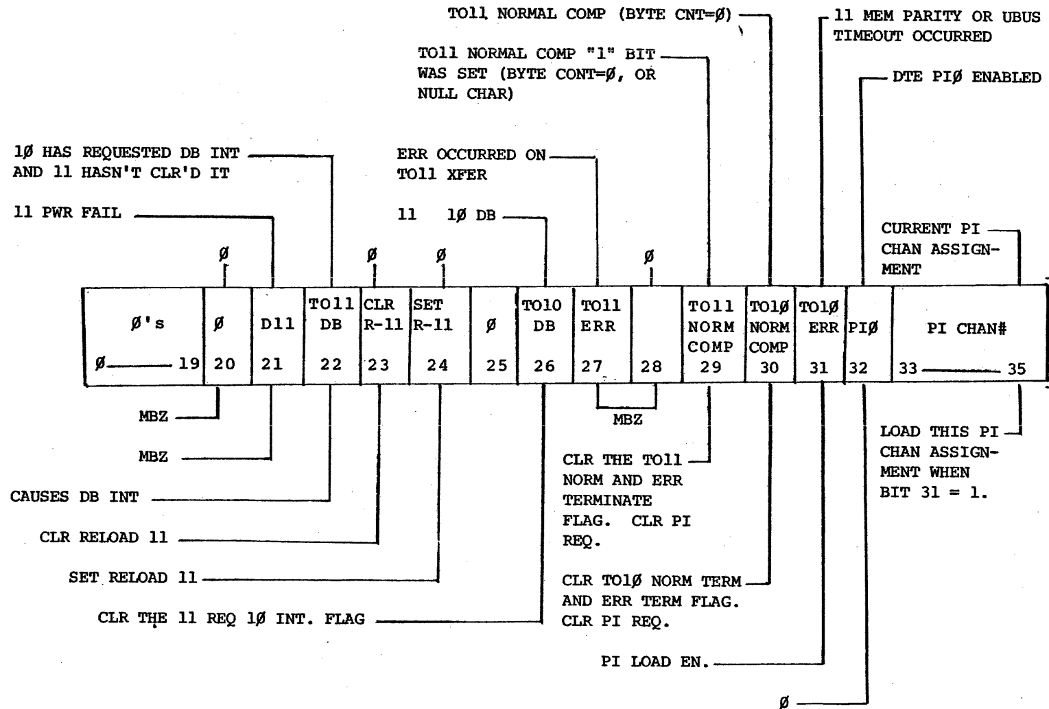
FIGURE 5, KL10 CONO, CONI FORMATS
