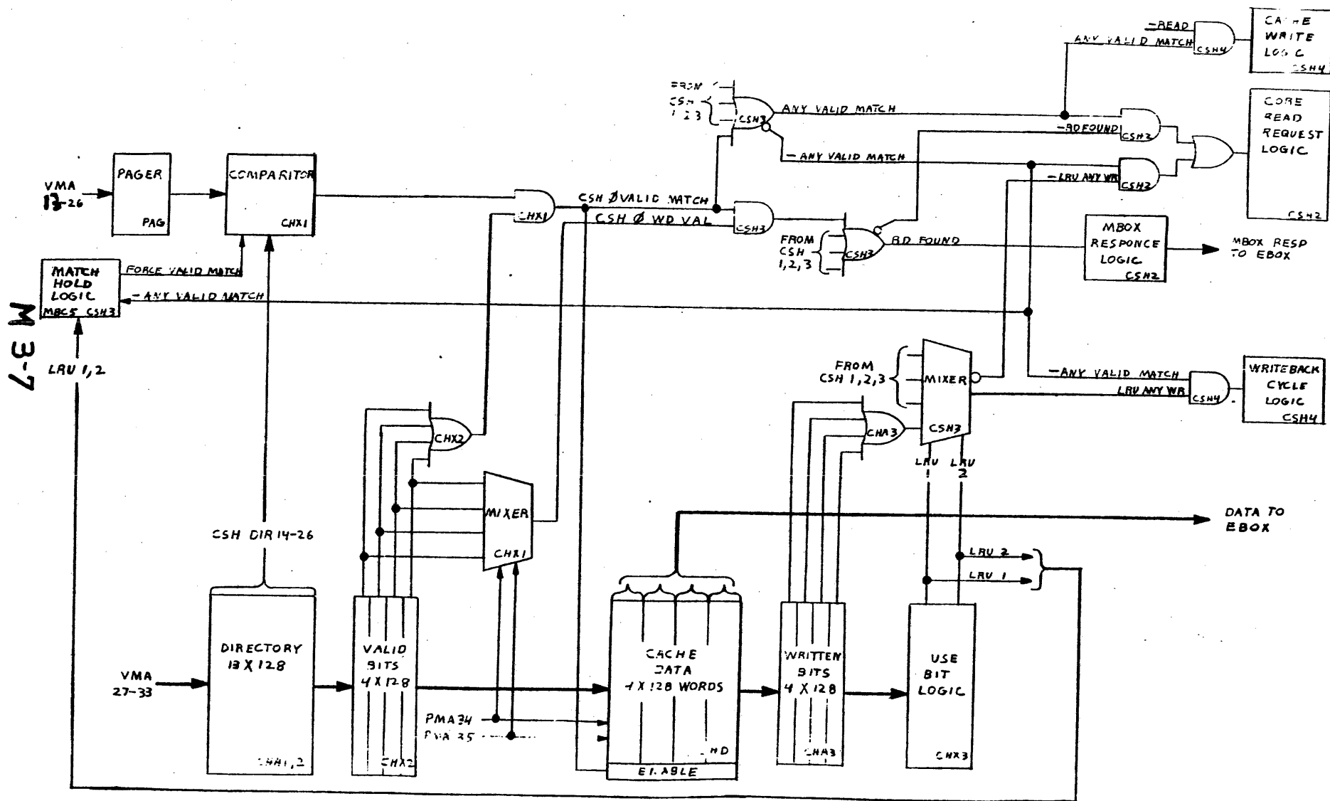
Figure 3-3 Memory Reference Decision Paths
