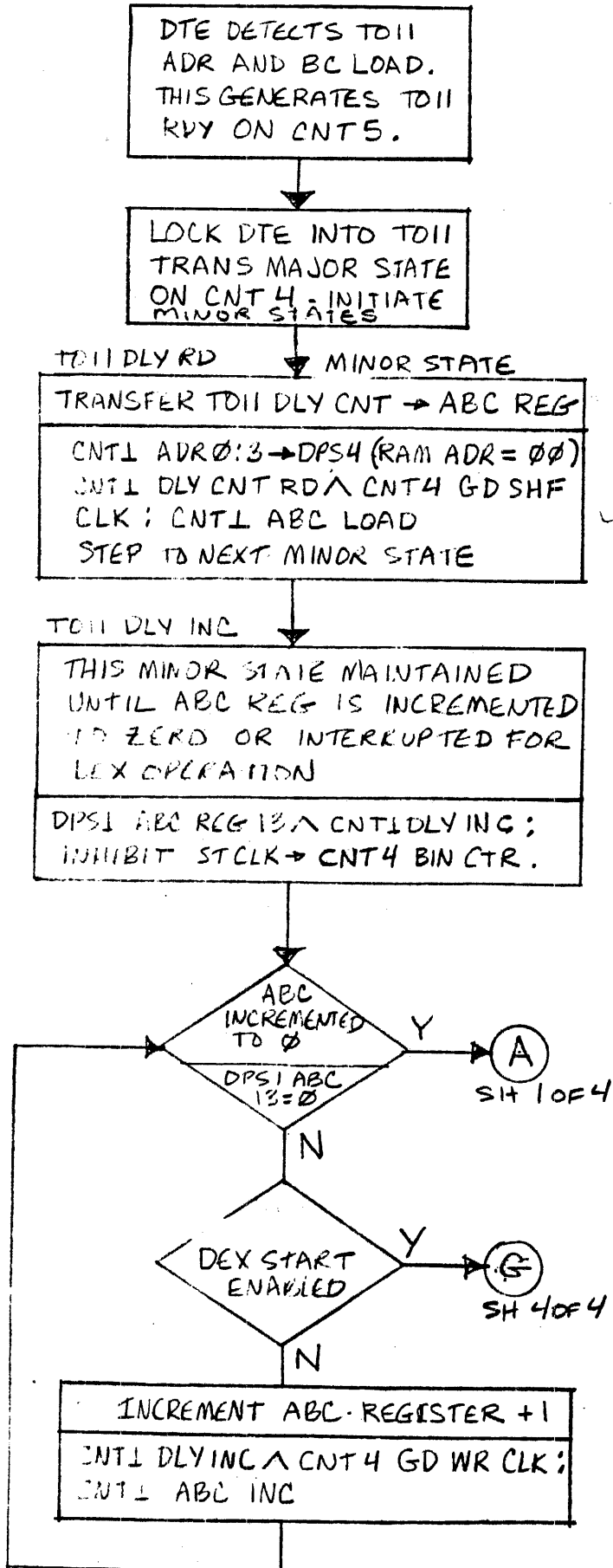
FIGURE 1, TOII TRANS SHEET 1 OF 4
