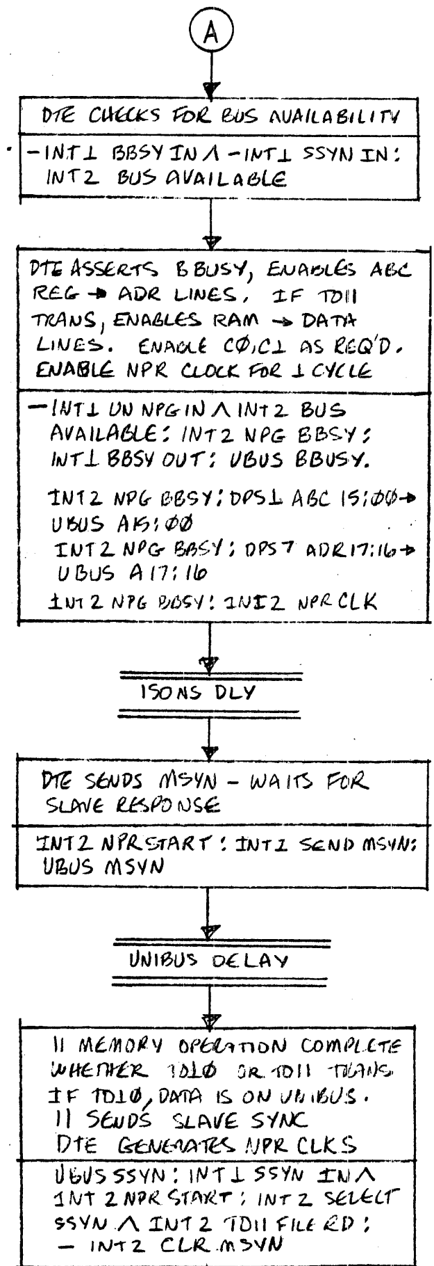
NO ITE FIGURE 4, NPR OPERATION SHEET 1 OF 2 D 2-24
