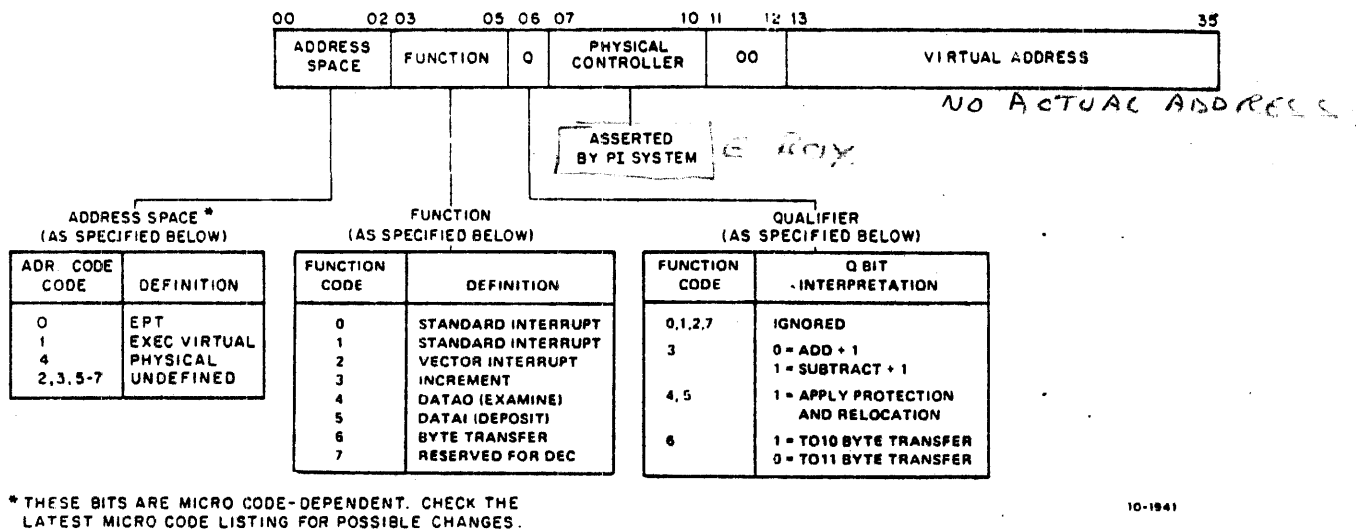
Figure 1-2 API Word Format
