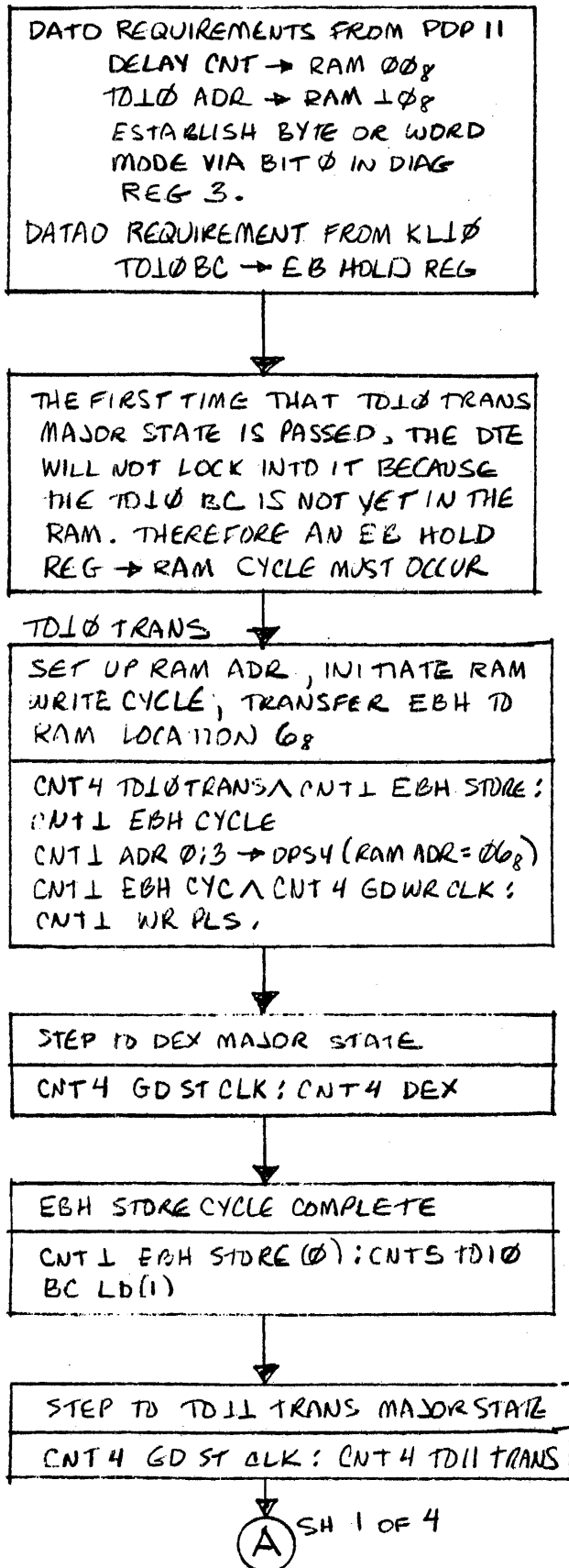
FIGURE 2. TD10 TRANS SHEET 1 OF 4
