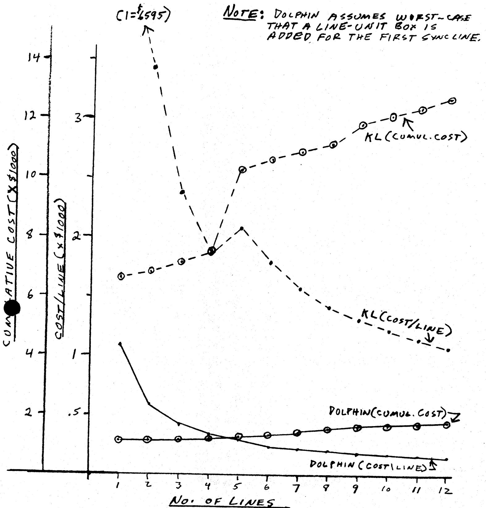
FIG 9 SYNCHRONOUS LINE COST COMPARISON KL / DOLPHIN
