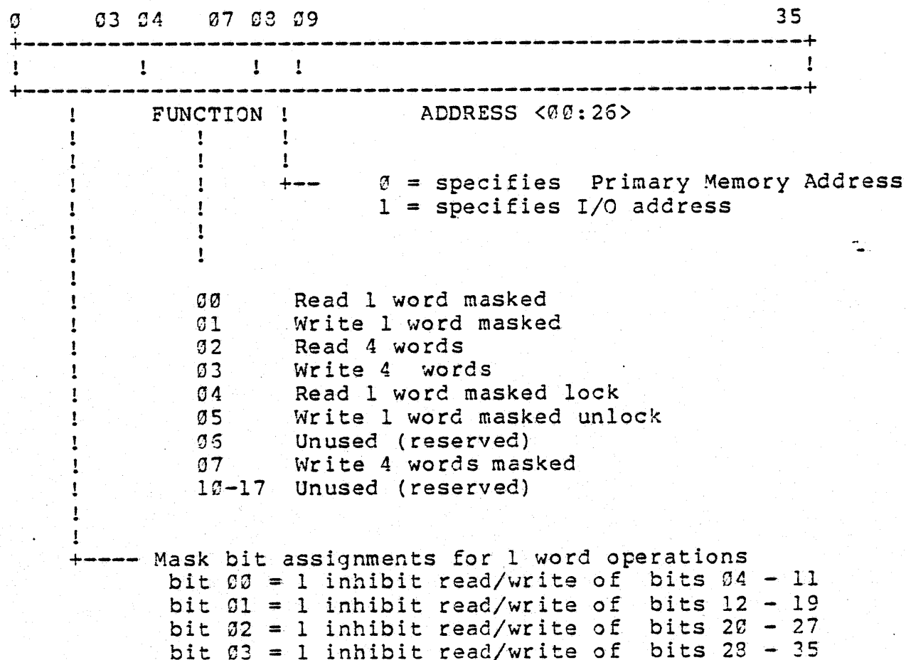
Figure 1 Data Line Interpretations for Command Tag (Dolphin)
