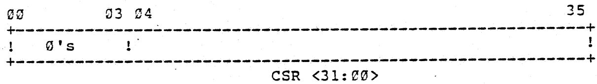
Figure 6 Format of a CSR
