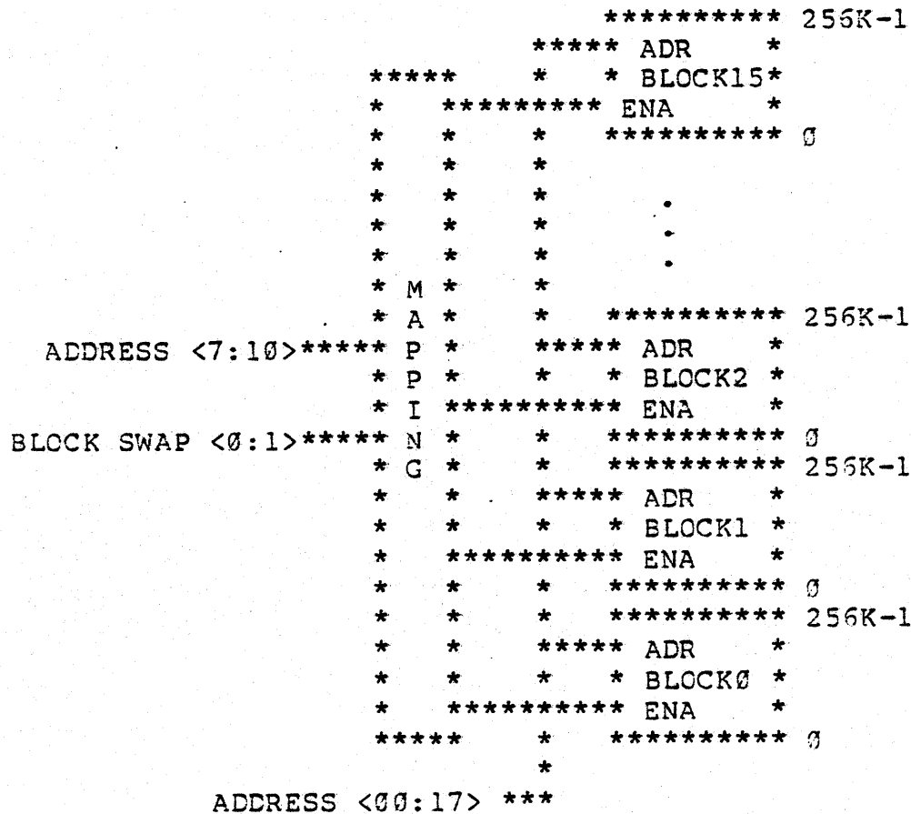
FIGURE 5 MAPPING OF PRIMARY MEMORY ADDRESS ONTO PHYSICAL MEMORY
