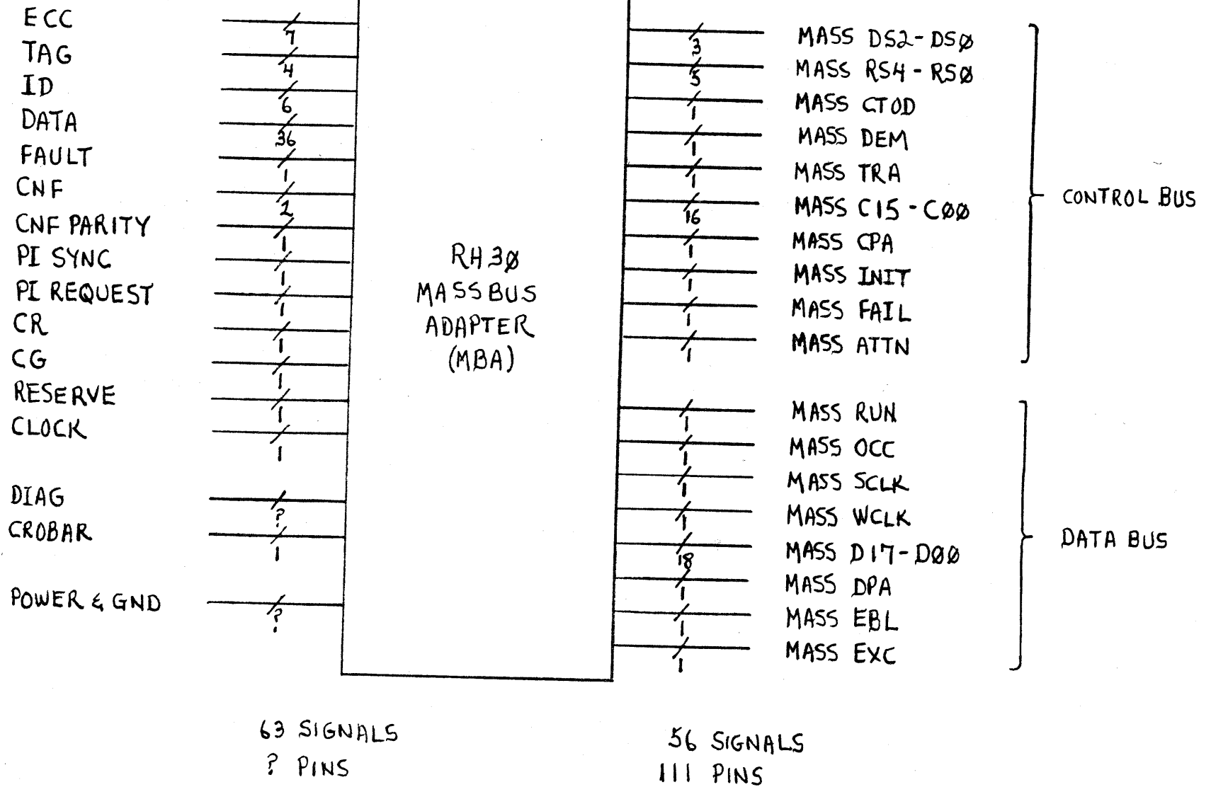
RH30 MASSBUS ADAPTER INPUT/OUTPUT SIGNALS
