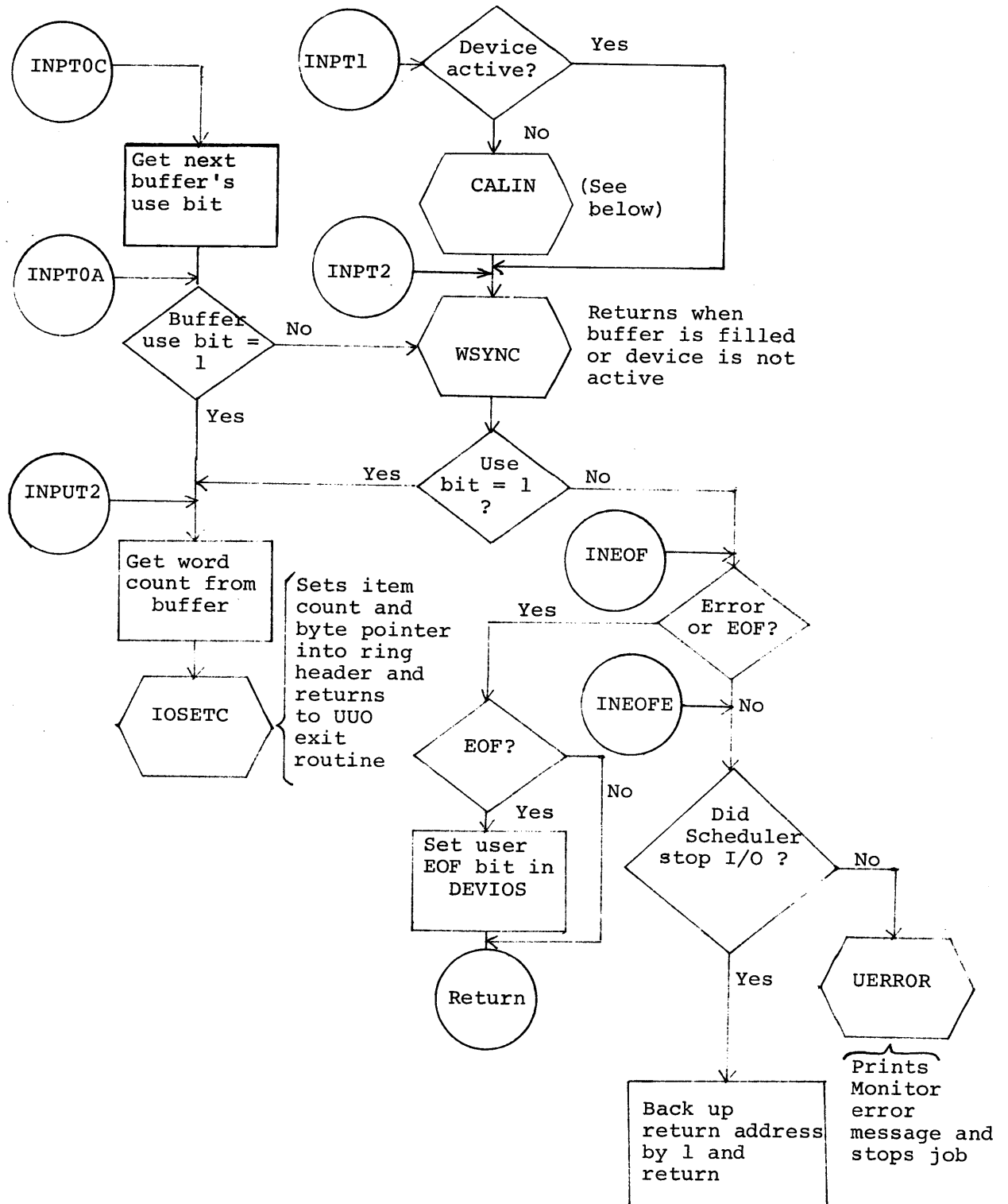
Figure 5 (Cont.) Flow Chart of INPUT Operator
