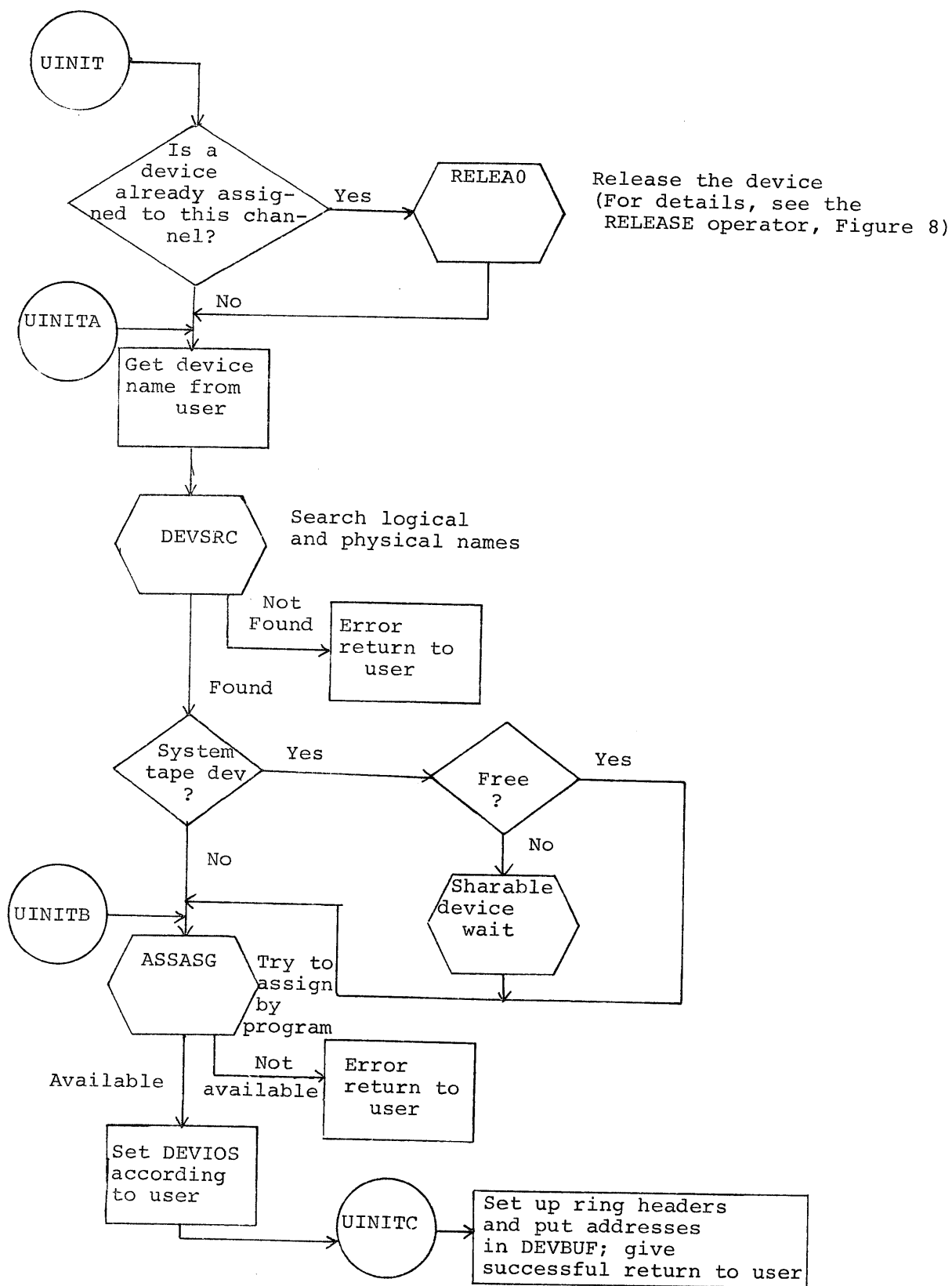
Figure 3. Flow Chart of INIT
