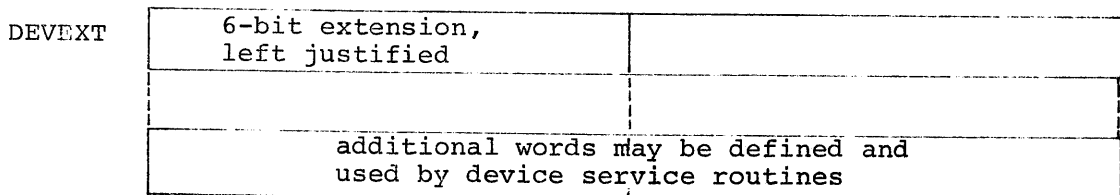
Figure 10. Device Data Block (DDB)
