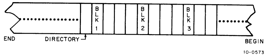
Figure 6-2 Format of a File on Tape
