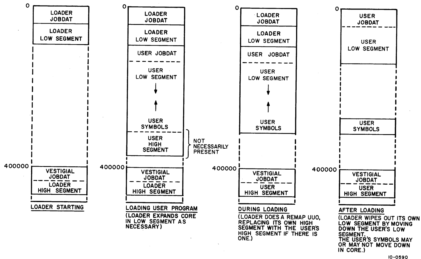
Figure 3-2 Loading User Core Area
