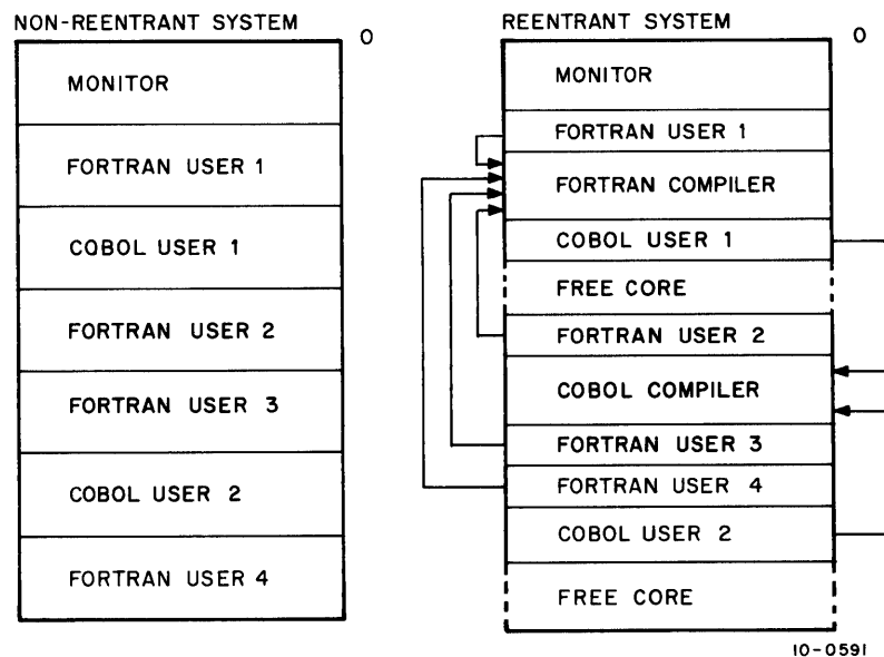
Figure 1-1 Core Management
