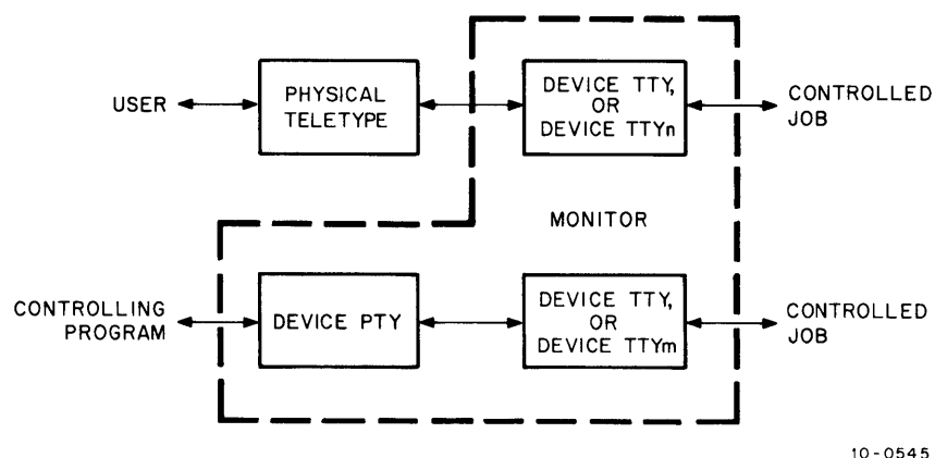
Figure 5-1 Pseudo-Teletype
