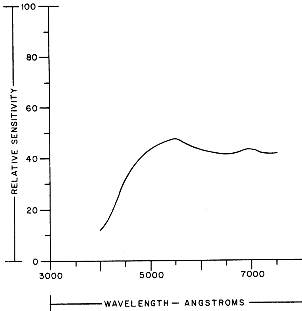
Figure A-2 Transmission Curve for Four Foot Length of Standard Light Guide
