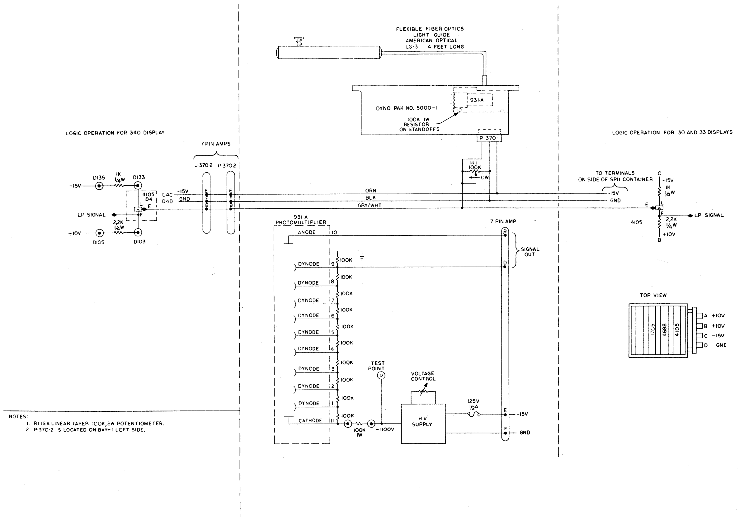
Figure A-5 Interconnection Wiring and Logic D-370-0-2
