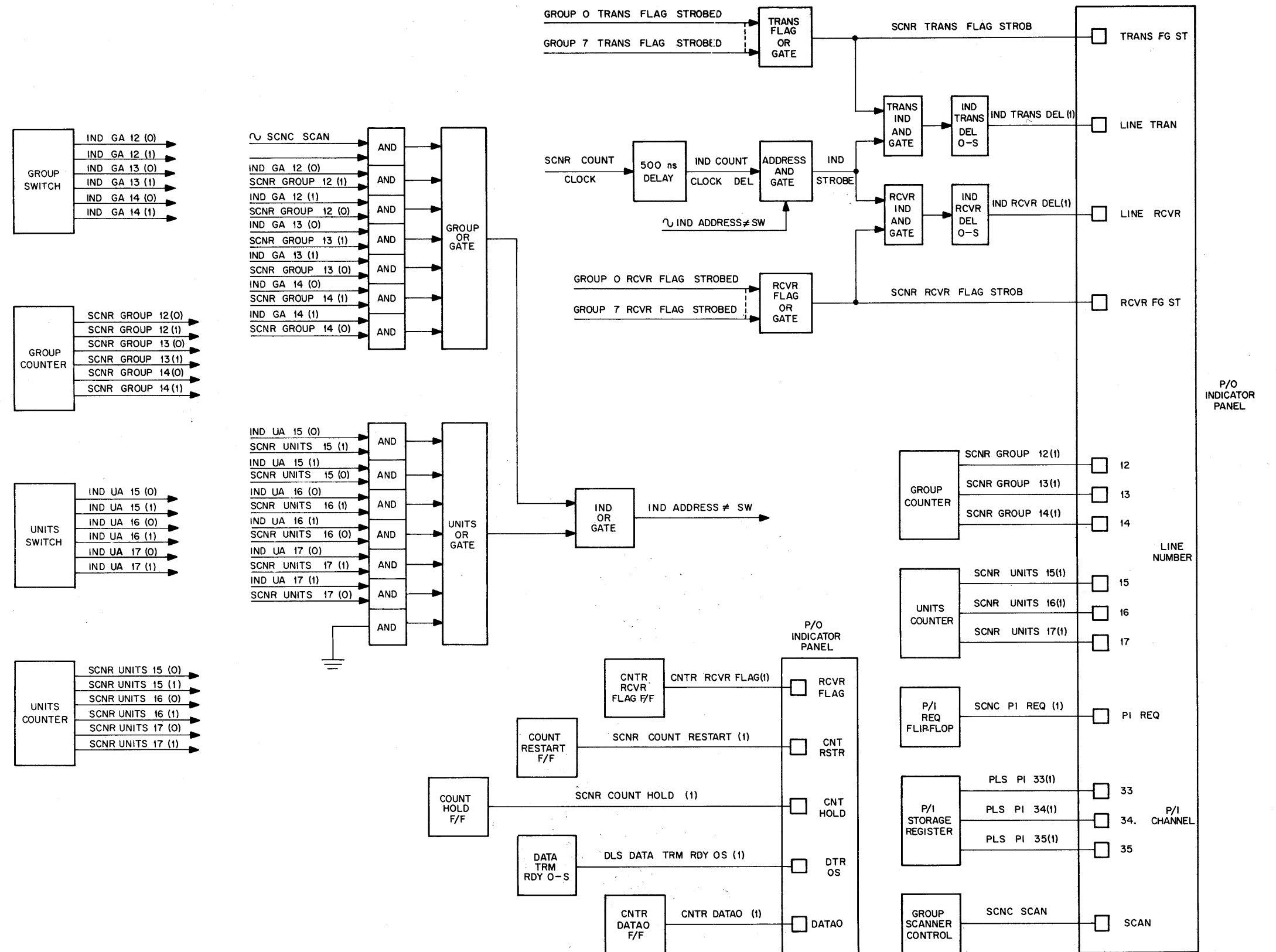
Figure 3-10 Indicator Circuit
