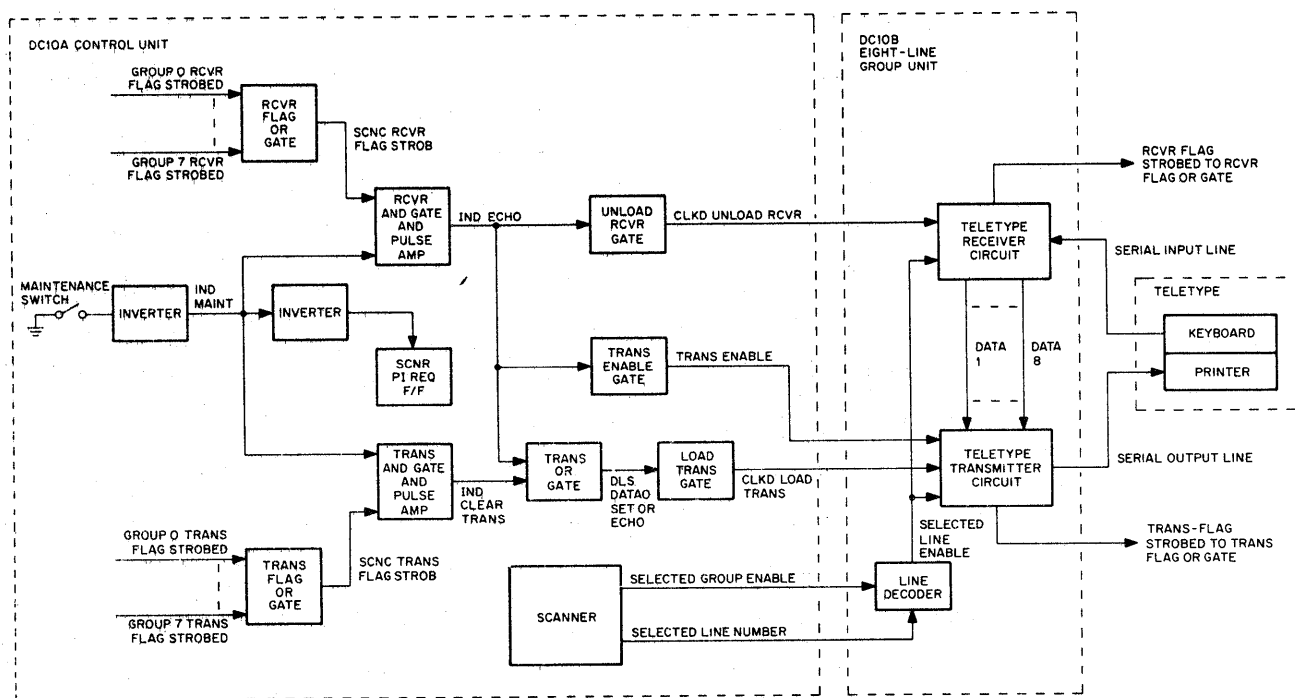
Figure 3-11 Echo Circuit
