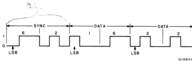
Figure 1-4 DS10 Serial Message Format for 6-Bit Characters
