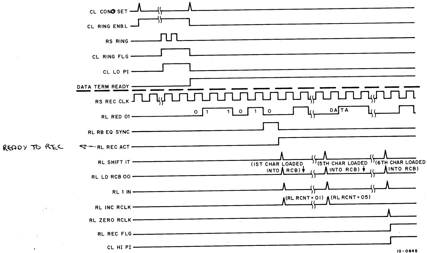
Figure 4-3 Receive Timing Diagram
