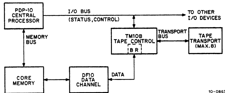
Figure 1-4 TM10B Tape Control Configuration
