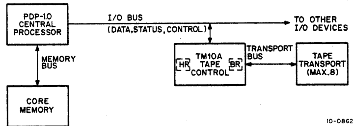
Figure 1-3 TM10A Tape Control Configuration
