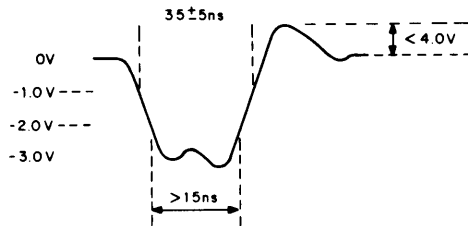
Figure 5-3 B-Series Pulse
