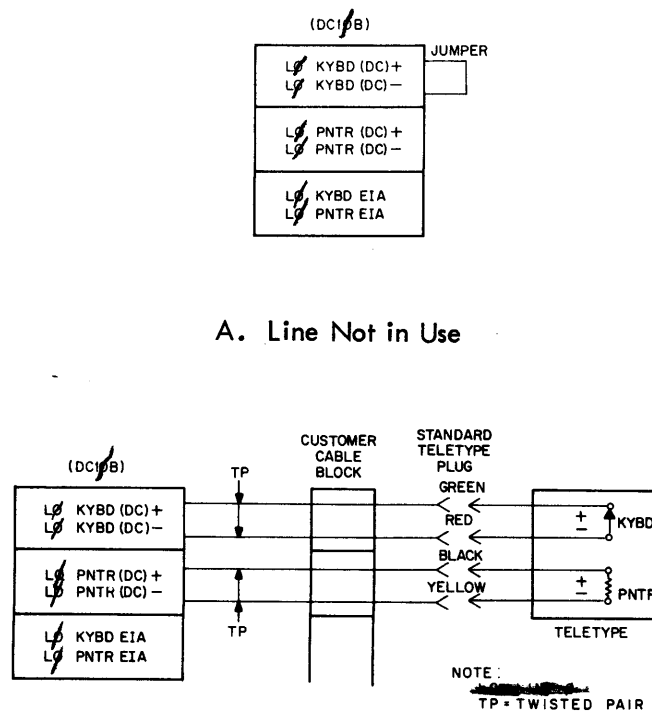
B. Local Line - Current Mode - Full Duplex Model 33 or 35 Teletype
