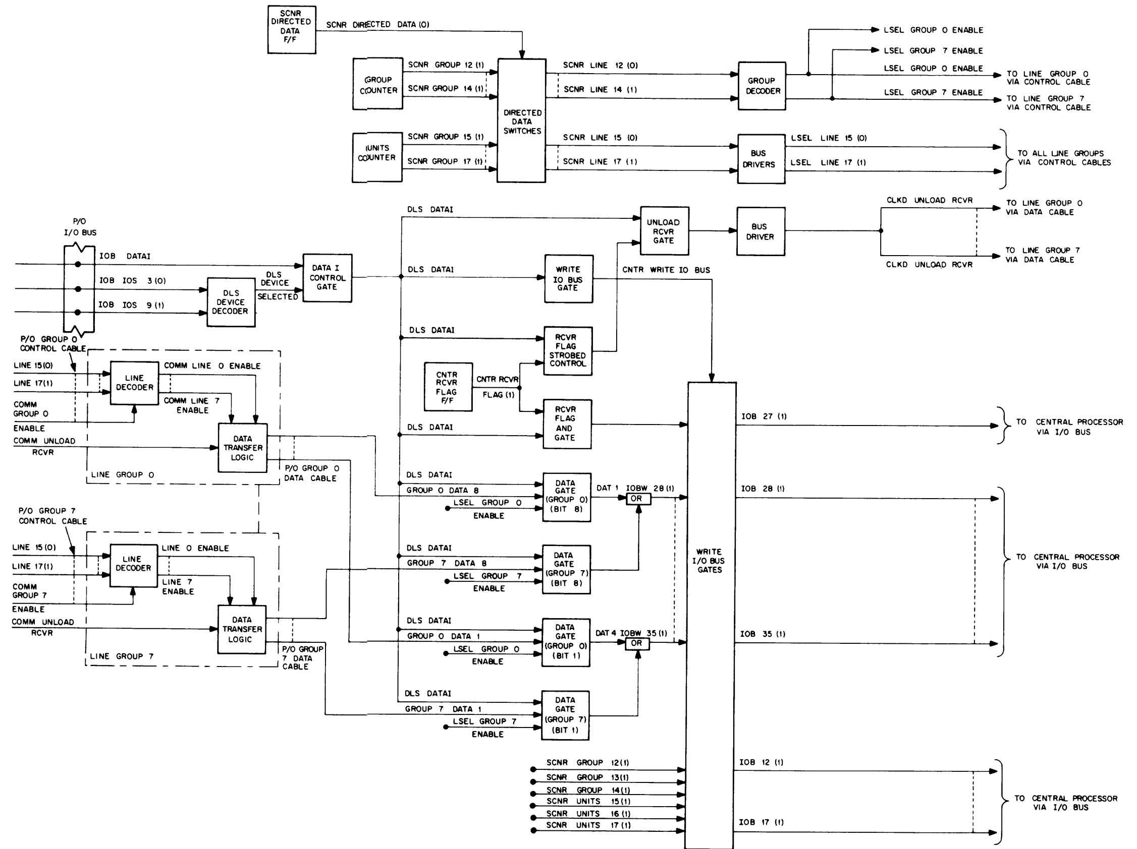
Figure 3-7 Control Unit DC10A, Block Diagram DATAI Instruction
