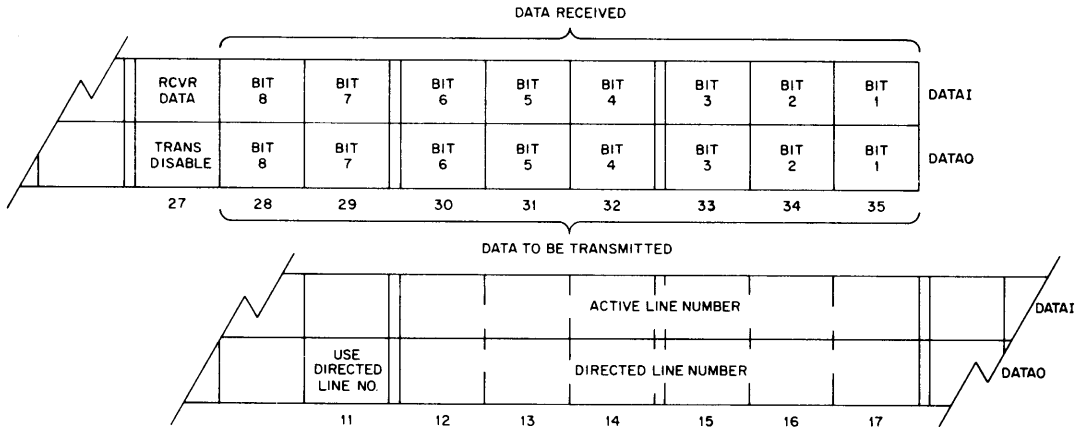
Figure 2-5 DC10B Data
