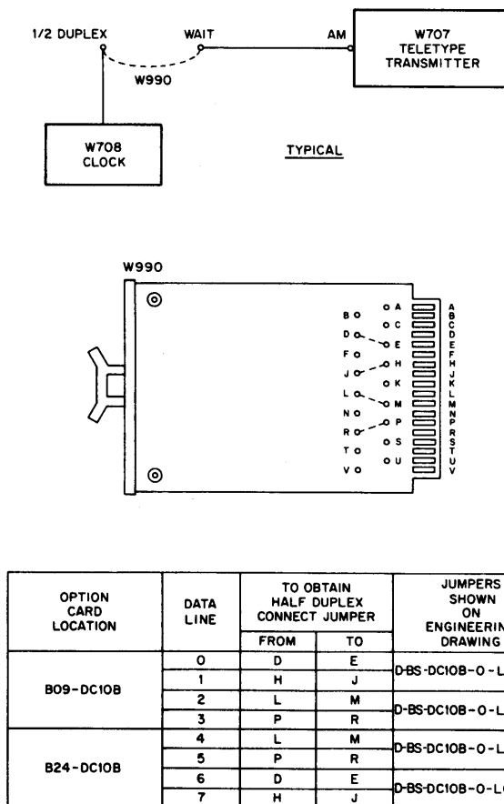
Figure 2-12 Half-Duplex Option Card (DC10B)
