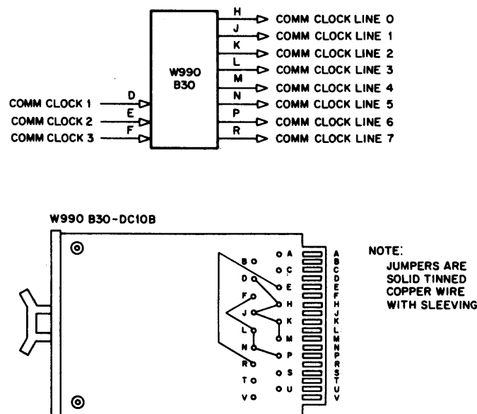
Figure 2-11 Clock Line Option Card (DC10B)
