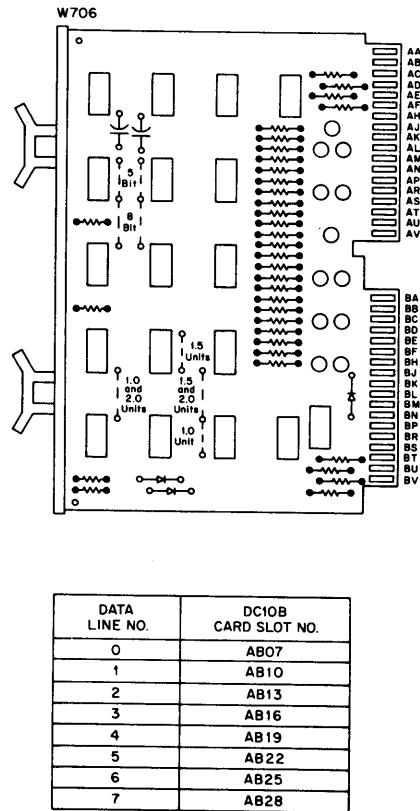
Figure 2-13 Teletype Receiver Module W706 (DC10B)
