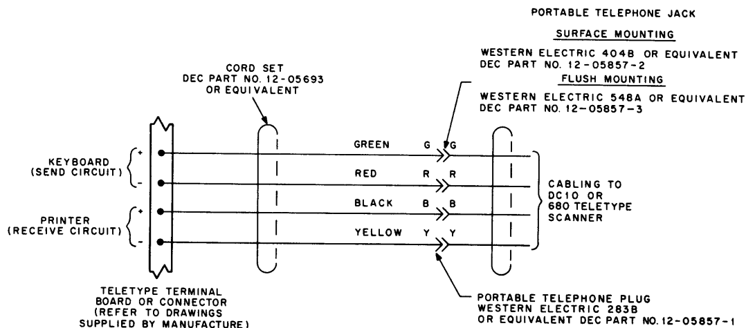
Figure 2-19 20 mA, Full Duplex Terminals
