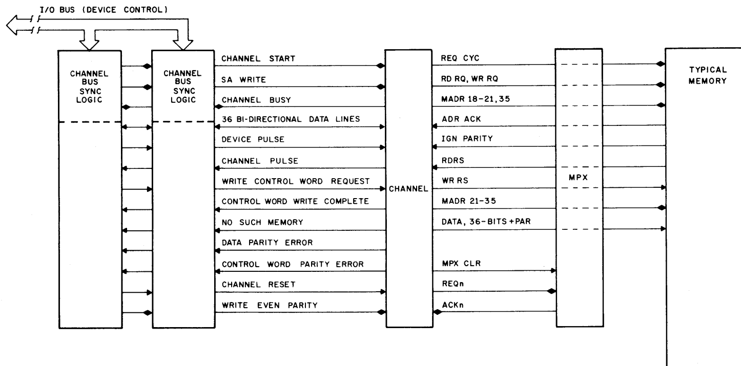
Figure 1-2 DF10 Interface
