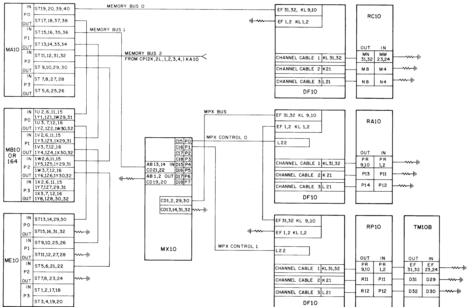
Figure 2-2 System Interconnections*
