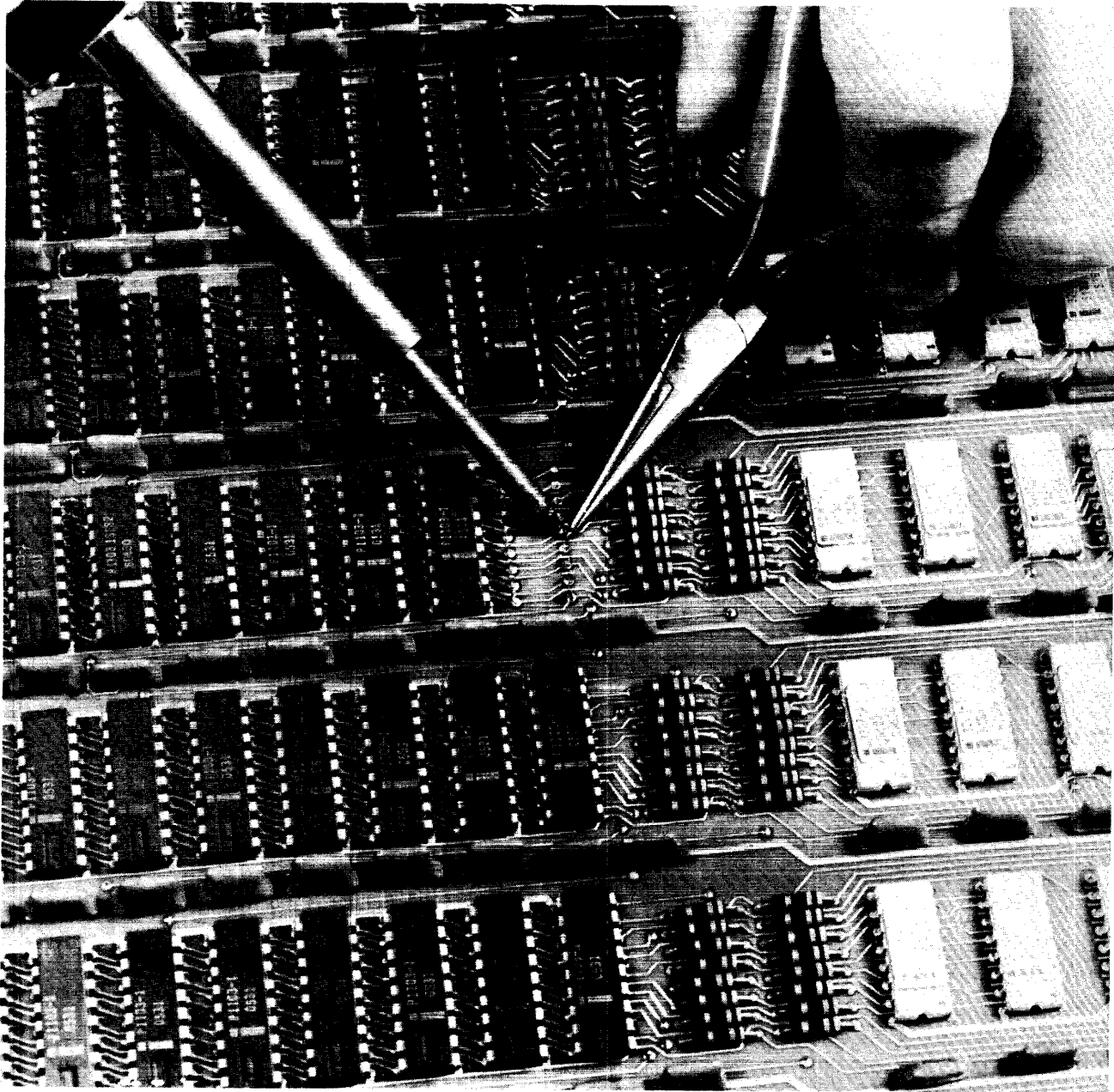
Figure B-6 removing IC Leads
