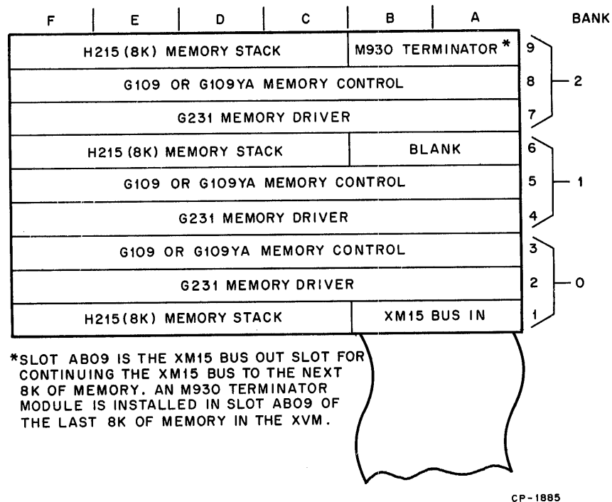
Figure 2-19 ME15 Assigned Module Slots (Module Side)
