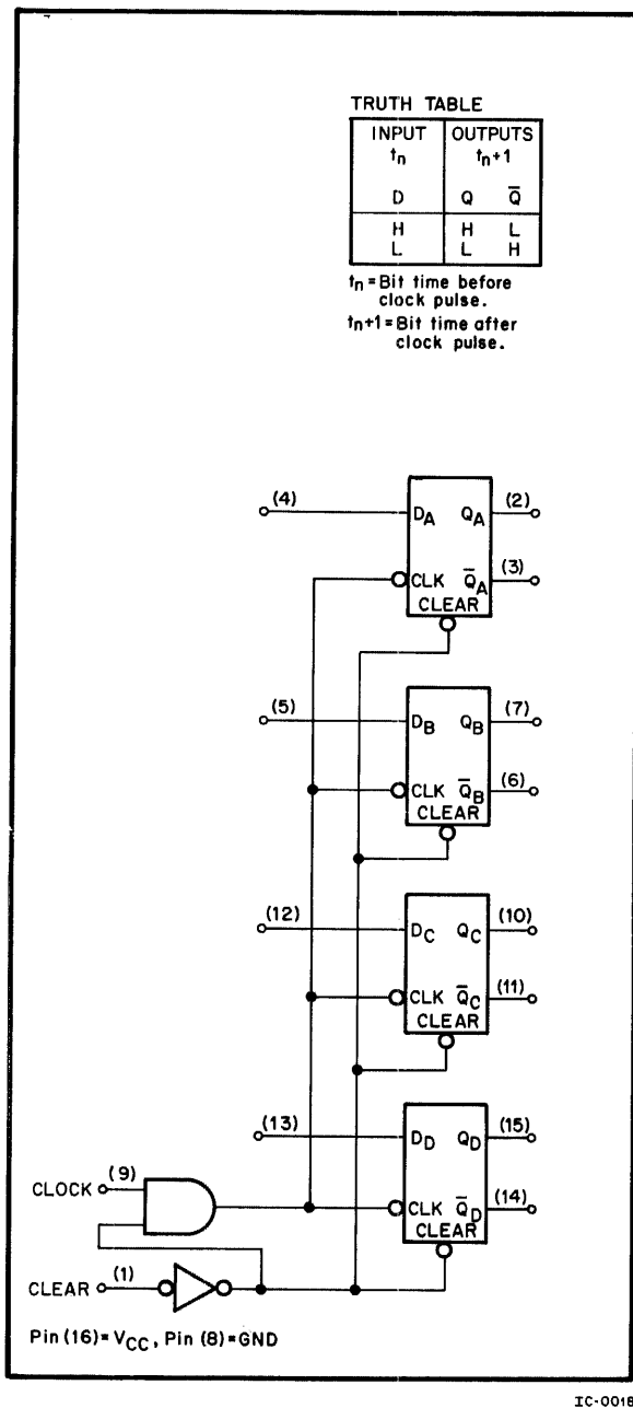
Figure C-13 74S175 Quad D-Type Flip-Flops
