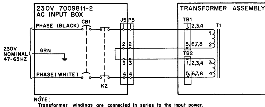
Figure 7-7 H765 Power Supply 230 V Power Configuration
