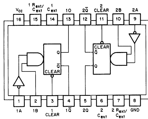
FUNCTIONAL LOGIC/PIN LOCATOR
