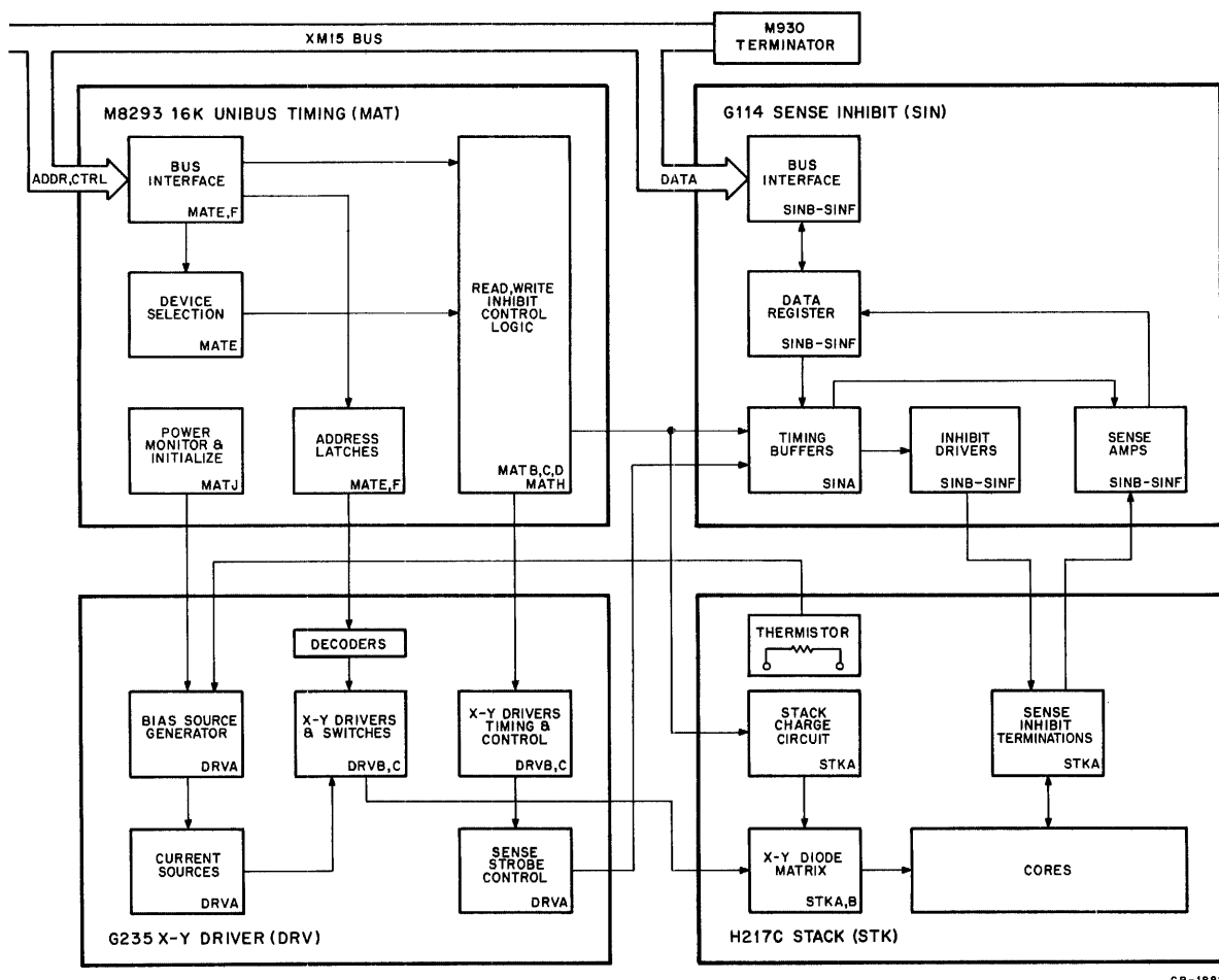
Figure 2-24 MF15 Simplified Block Diagram
