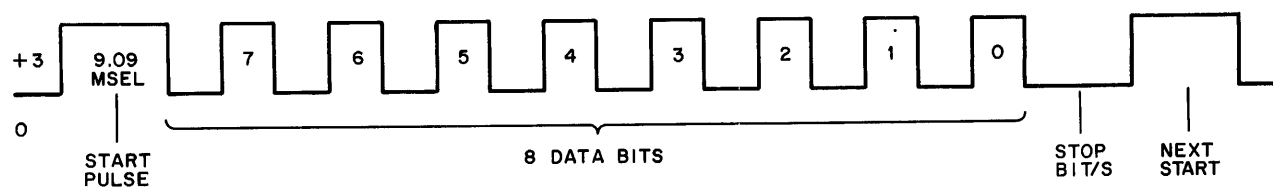
Figure 5-13 Teletype Serial ASCII Format
