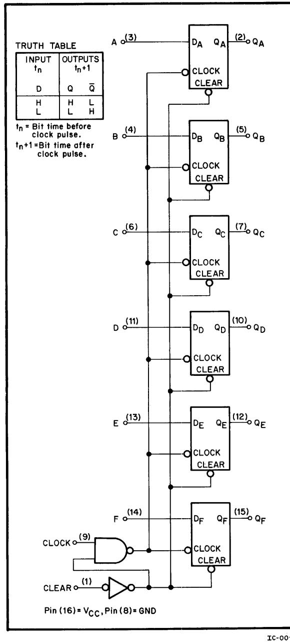
Figure C-12 74S174 Hex D-Type Flip-Flops
