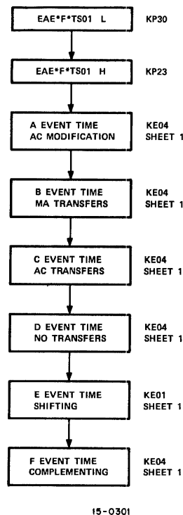
Figure 5-1 EAE General Flow Diagram
