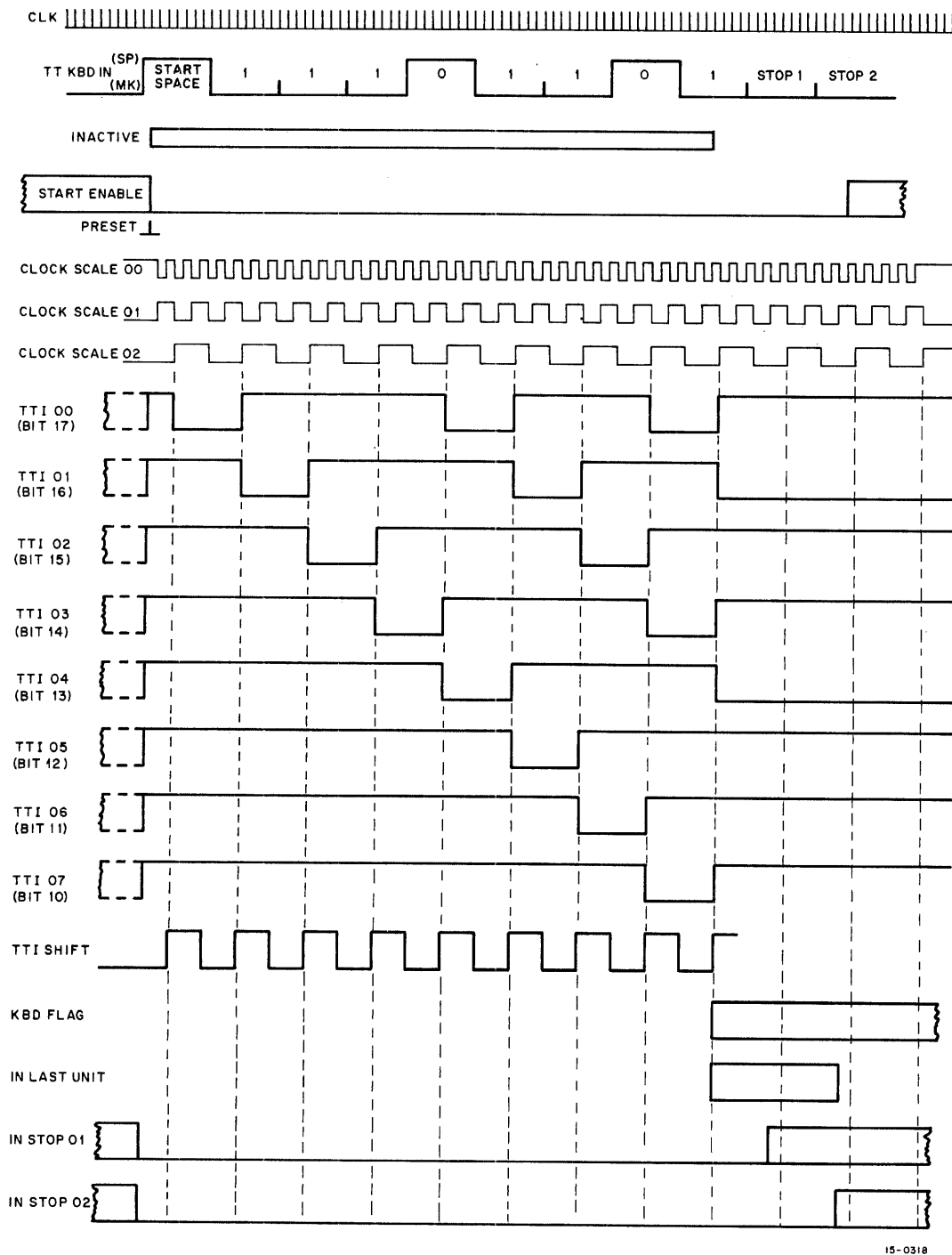
Figure 5-14 Teletype Receiver (Keyboard) Timing
