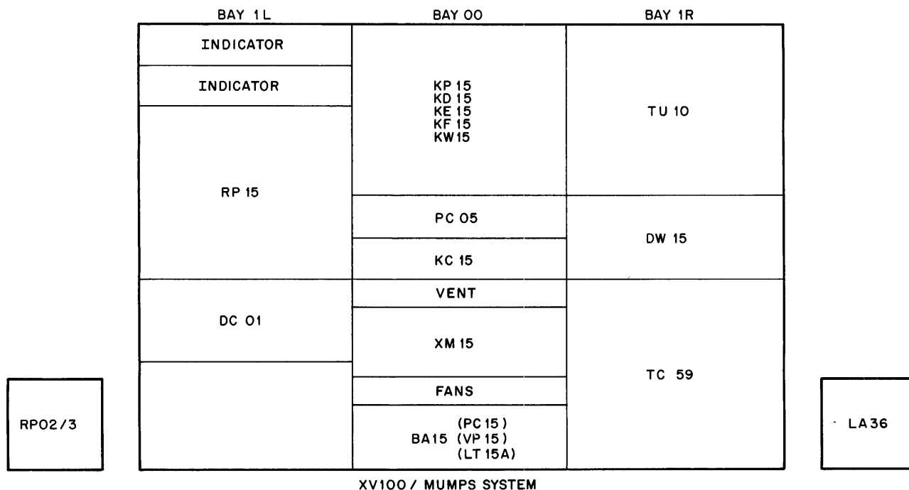
Figure 1-3 XV100 System Configuration Diagram
