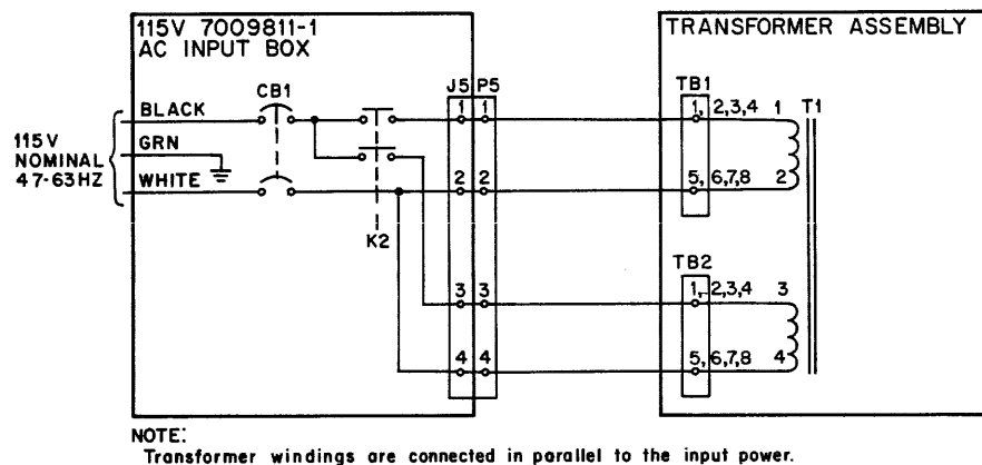
Figure 7-6 H765 Power Supply 115 V Power Configuration
