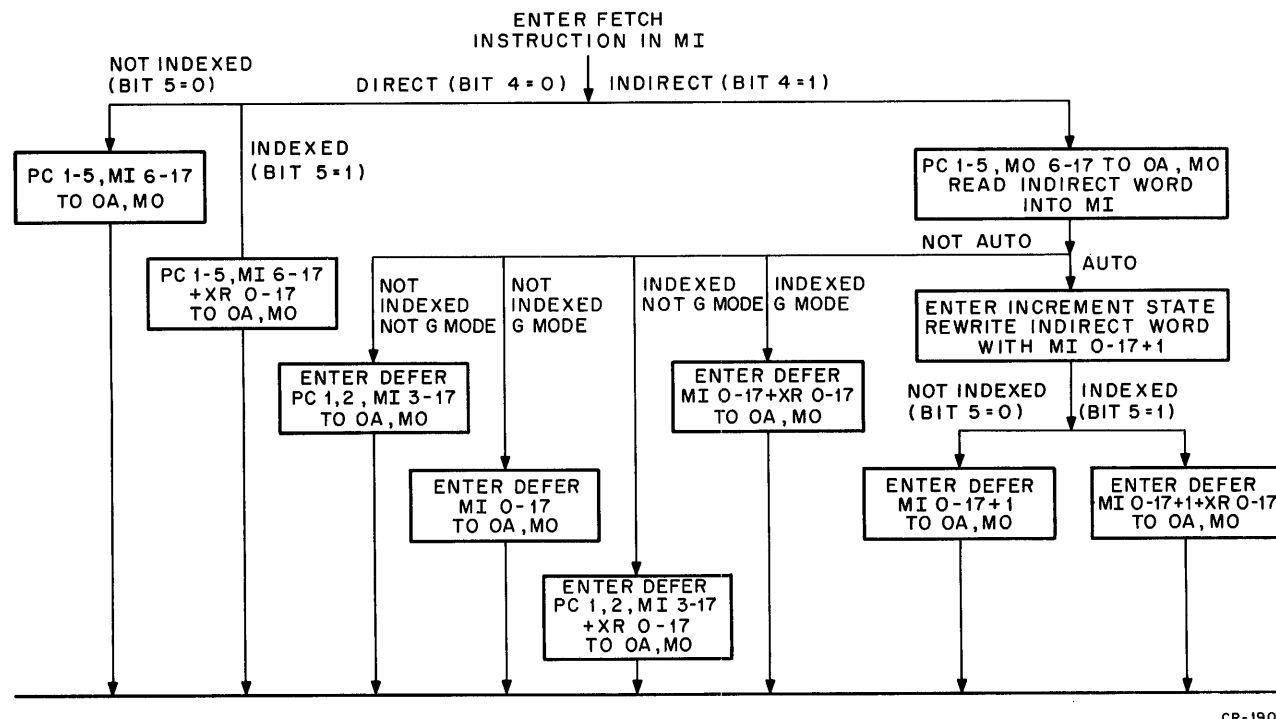
Figure 3-2 Page Mode Address Formation
