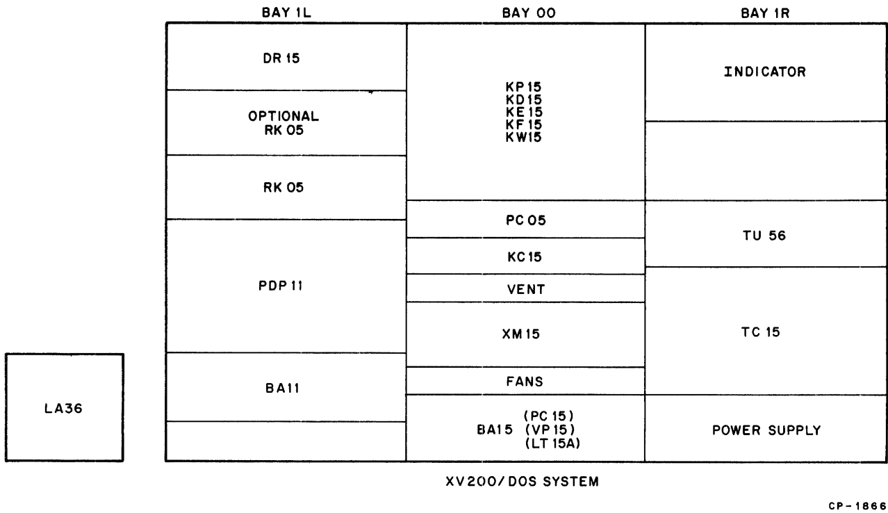
Figure 1-4 XV200 System Configuration Diagram
