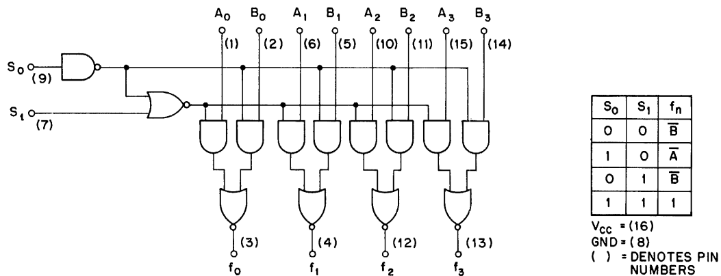
Figure C-2 8234 Digital Multiplexer
