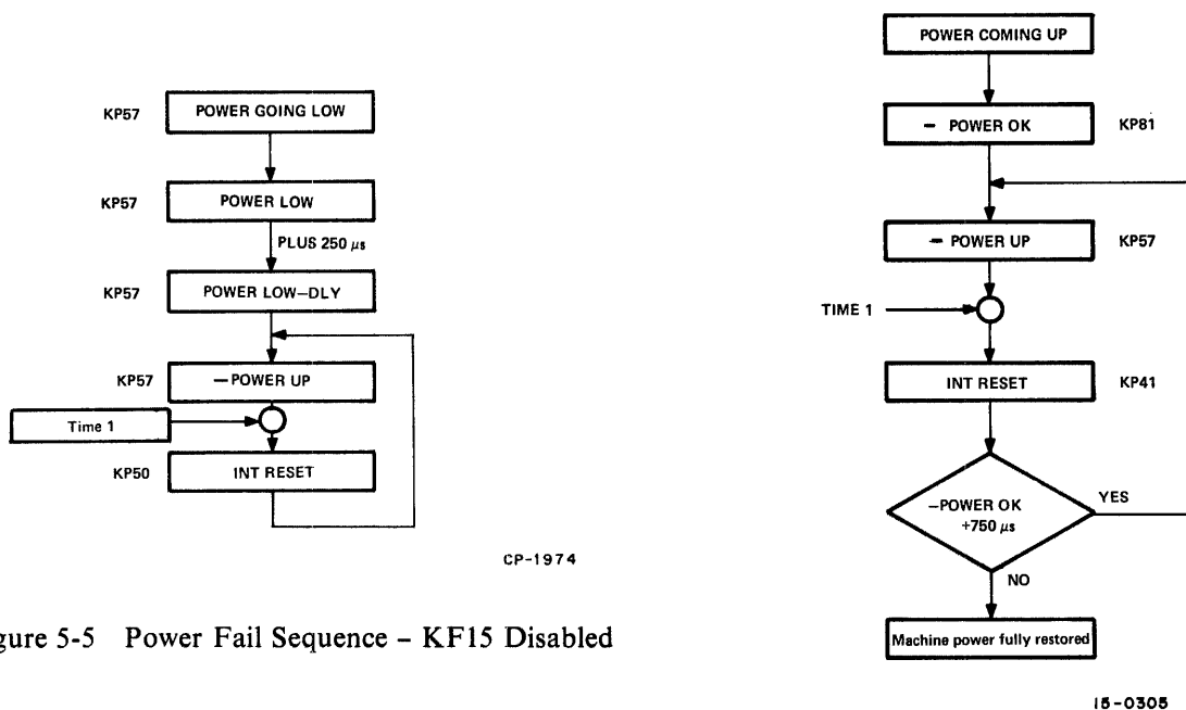
Figure 5-6 Power Restore Sequence – KF15 Disabled
